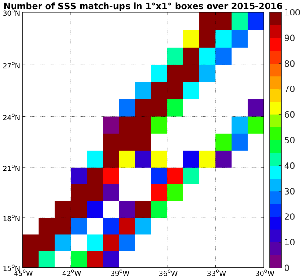
Figure 4: Number of SSS match-ups between TSG-LEGOS-DM SSS and the SMAP-L3-RSS-V2-8DAY-RUNNING-70KM SSS product for the SPURS 1 Pi-MEP region over 1°x1° boxes and for the full satellite product period.
