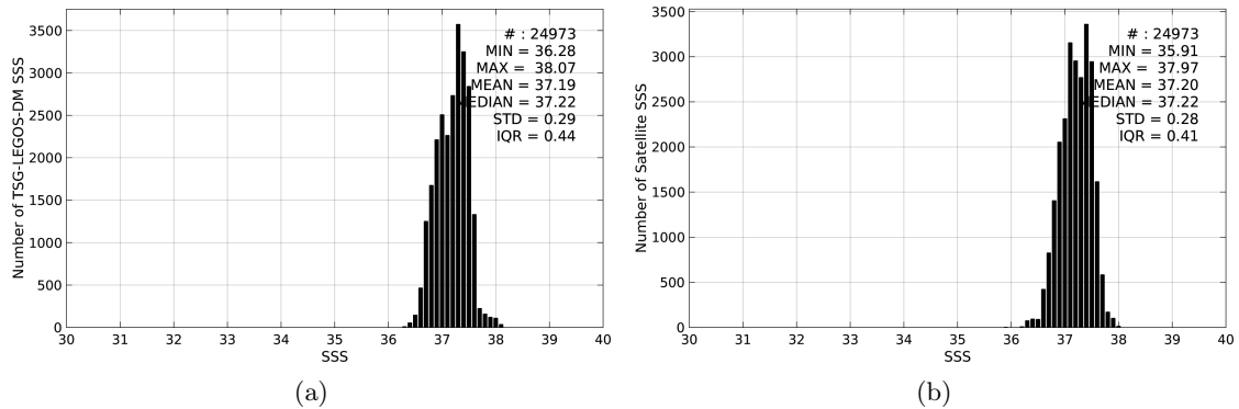
Figure 2: Histograms of SSS from TSG-LEGOS-DM (a) and SMAP-L3-RSS-V2-8DAY-RUNNING-70KM (b) considering all match-up pairs per bins of 0.1 over the SPURS 1 Pi-MEP region and for the full satellite product period.
