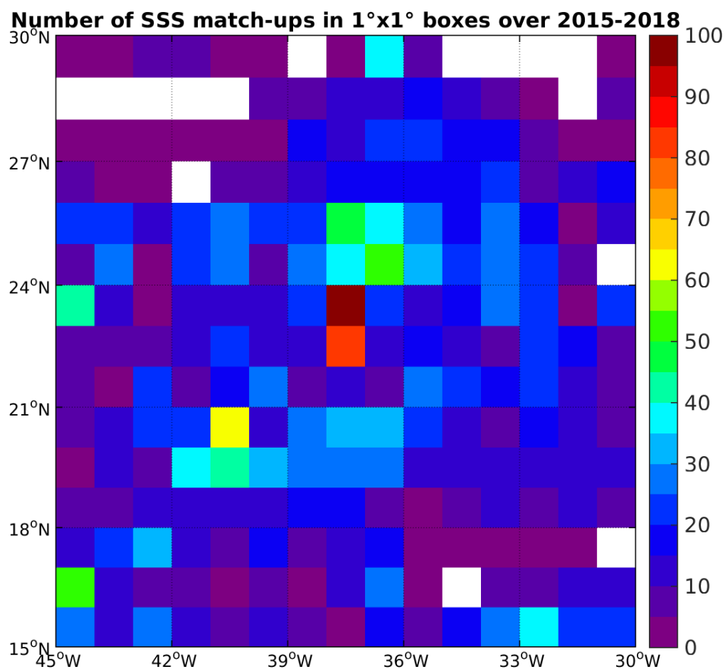
Figure 4: Number of SSS match-ups between Argo SSS and the SMAP-L3-RSS-V2-8DAY-RUNNING-70KM SSS product for the SPURS 1 Pi-MEP region over 1°x1° boxes and for the full satellite product period.
