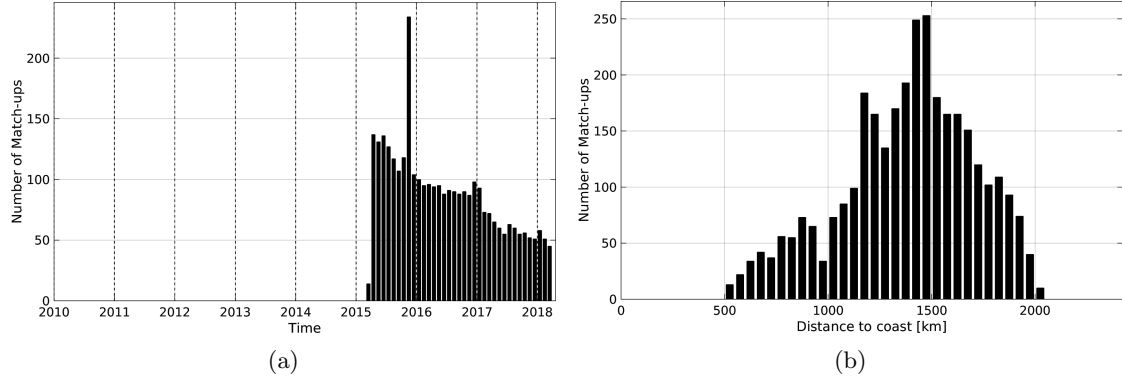
Figure 1: Number of match-ups between Argo and SMAP-L3-RSS-V2-8DAY-RUNNING-70KM SSS as a function of time (a) and as function of the distance to coast (b) over the SPURS 1 Pi-MEP region and for the full satellite product period.
