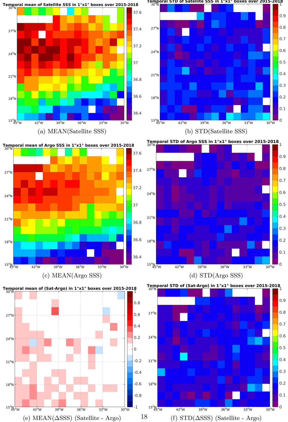
Figure 6: Temporal mean (left) and STD (right) of SSS from SMAP-L3-RSS-V2-8DAY-RUNNING-70KM (top), Argo (middle), and of \Delta SSS (Satellite - Argo). Only match-up pairs are used to generate these maps.
