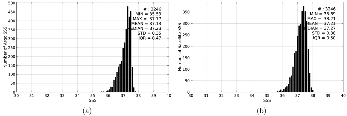
Figure 2: Histograms of SSS from Argo (a) and SMAP-L3-RSS-V2-8DAY-RUNNING-70KM (b) considering all match-up pairs per bins of 0.1 over the SPURS 1 Pi-MEP region and for the full satellite product period.
