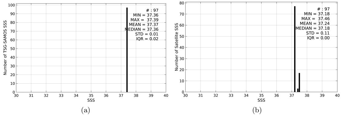
Figure 2: Histograms of SSS from TSG-SAMOS (a) and SMAP-L3-RSS-V2-MONTHLY-0.25DEG-40KM (b) considering all match-up pairs per bins of 0.1 over the SPURS 1 Pi-MEP region and for the full satellite product period.
