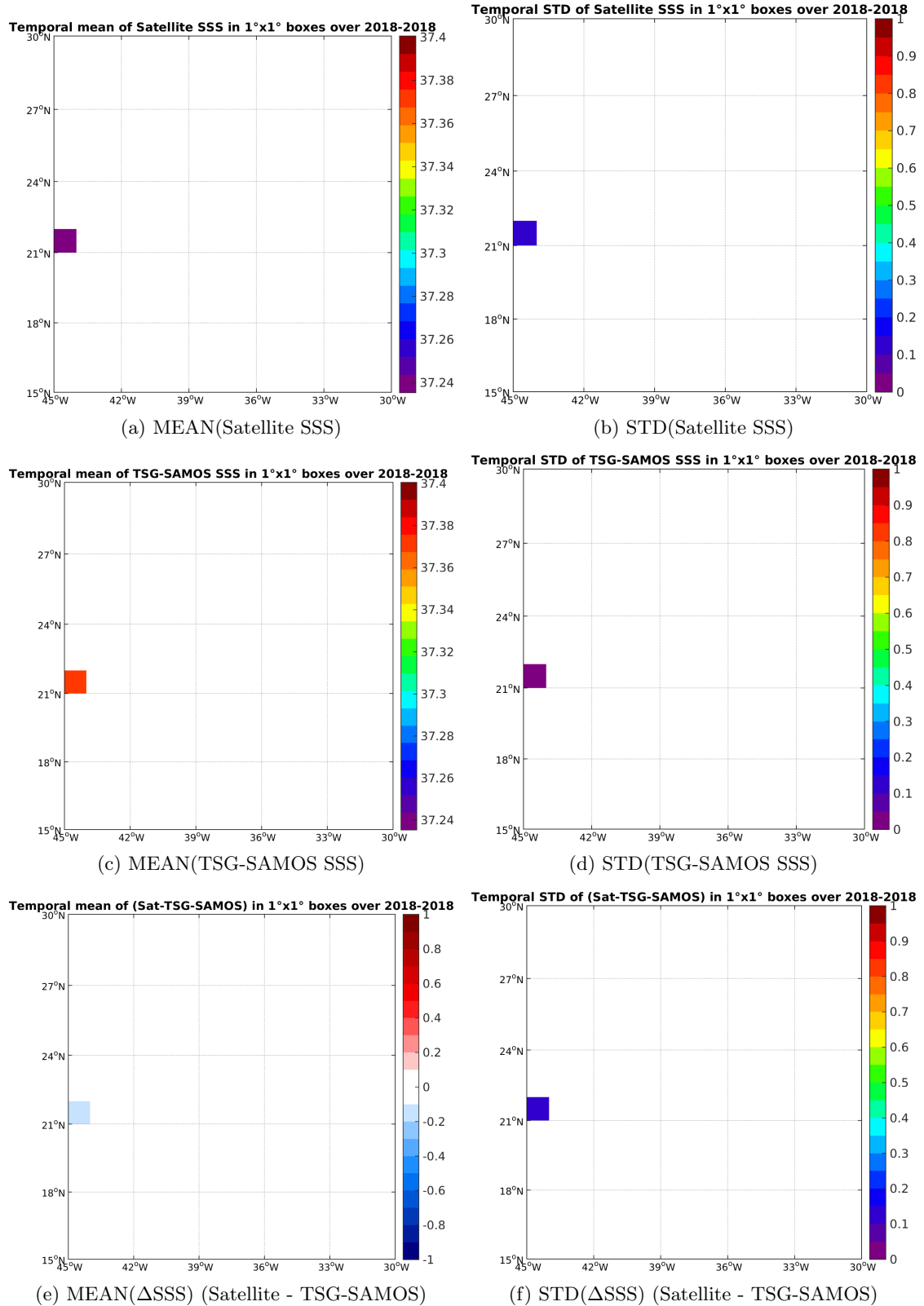
Figure 6: Temporal mean (left) and STD (right) of SSS from SMAP-L3-RSS-V2-MONTHLY-0.25DEG-40KM (top), TSG-SAMOS (middle), and of \Delta SSS (Satellite - TSG-SAMOS). Only match-up pairs are used to generate these maps.
