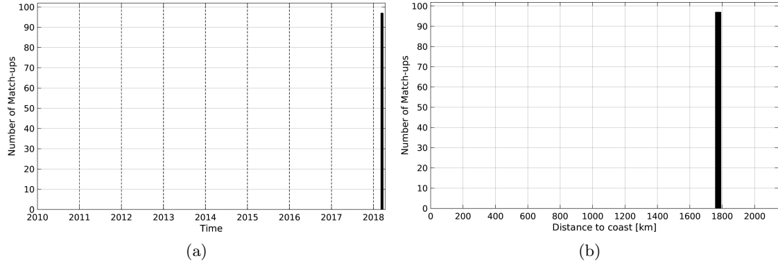
Figure 1: Number of match-ups between TSG-SAMOS and SMAP-L3-RSS-V2-MONTHLY-0.25DEG-40KM SSS as a function of time (a) and as function of the distance to coast (b) over the SPURS 1 Pi-MEP region and for the full satellite product period.
