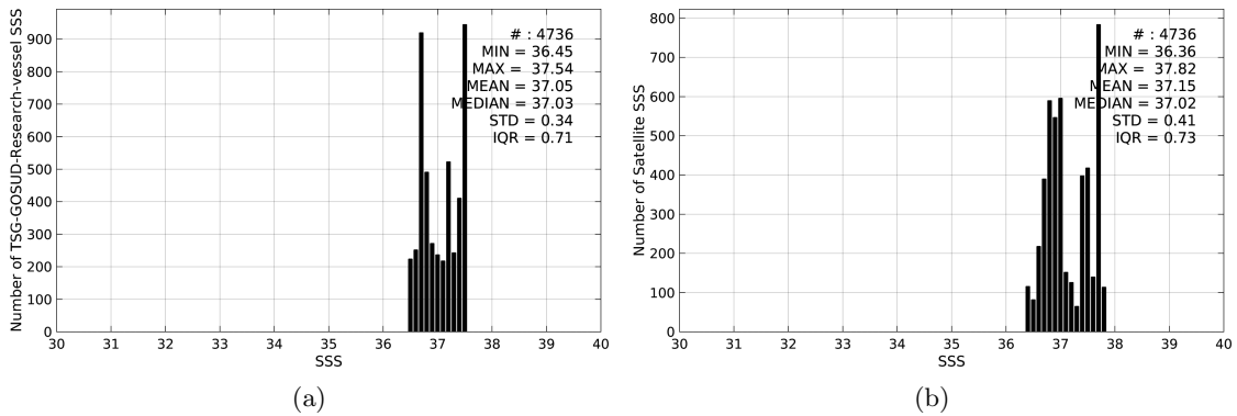
Figure 2: Histograms of SSS from TSG-GOSUD-Research-vessel (a) and SMAP-L3-RSS-V2-MONTHLY-0.25DEG-40KM (b) considering all match-up pairs per bins of 0.1 over the SPURS 1 Pi-MEP region and for the full satellite product period.
