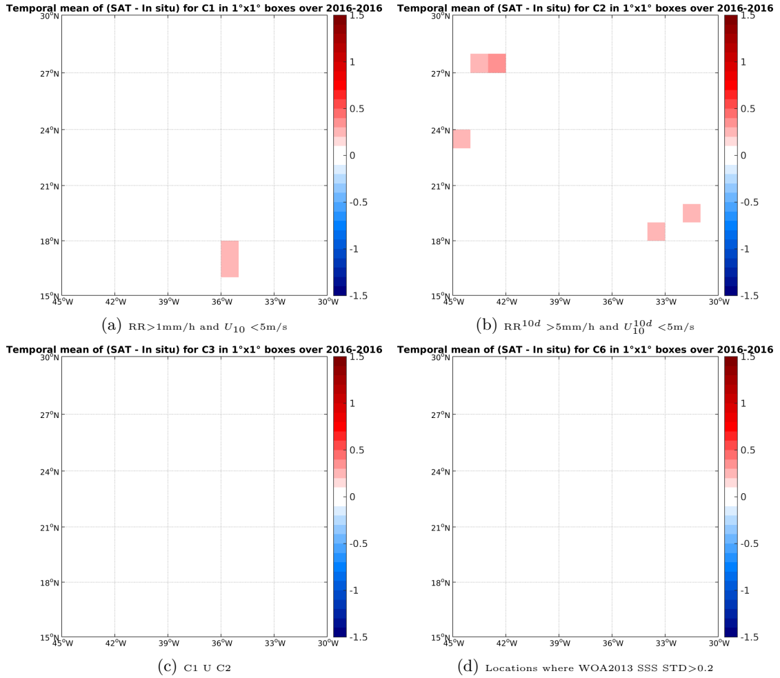
Figure 12: Temporal mean gridded over spatial boxes of size 1°x1° of \Delta SSS (SMAP-L3-RSS-V2-MONTHLY-0.25DEG-40KM - TSG-GOSUD-Research-vessel) for 4 different subdatasets corresponding to:RR>1mm/h and U_{10} < 5\text{m/s} (a), RR^{10d} > 5\text{mm/h} and U_{10}^{10d} < 5\text{m/s} (b), C1 U C2 (c),Locations where WOA2013 SSS STD>0.2 (d).
