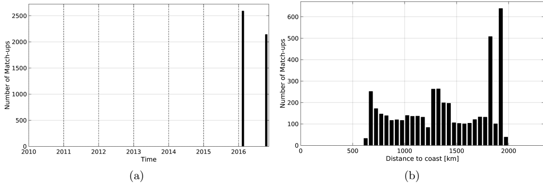
Figure 1: Number of match-ups between TSG-GOSUD-Research-vessel and SMAP-L3-RSS-V2-MONTHLY-0.25DEG-40KM SSS as a function of time (a) and as function of the distance to coast (b) over the SPURS 1 Pi-MEP region and for the full satellite product period.
