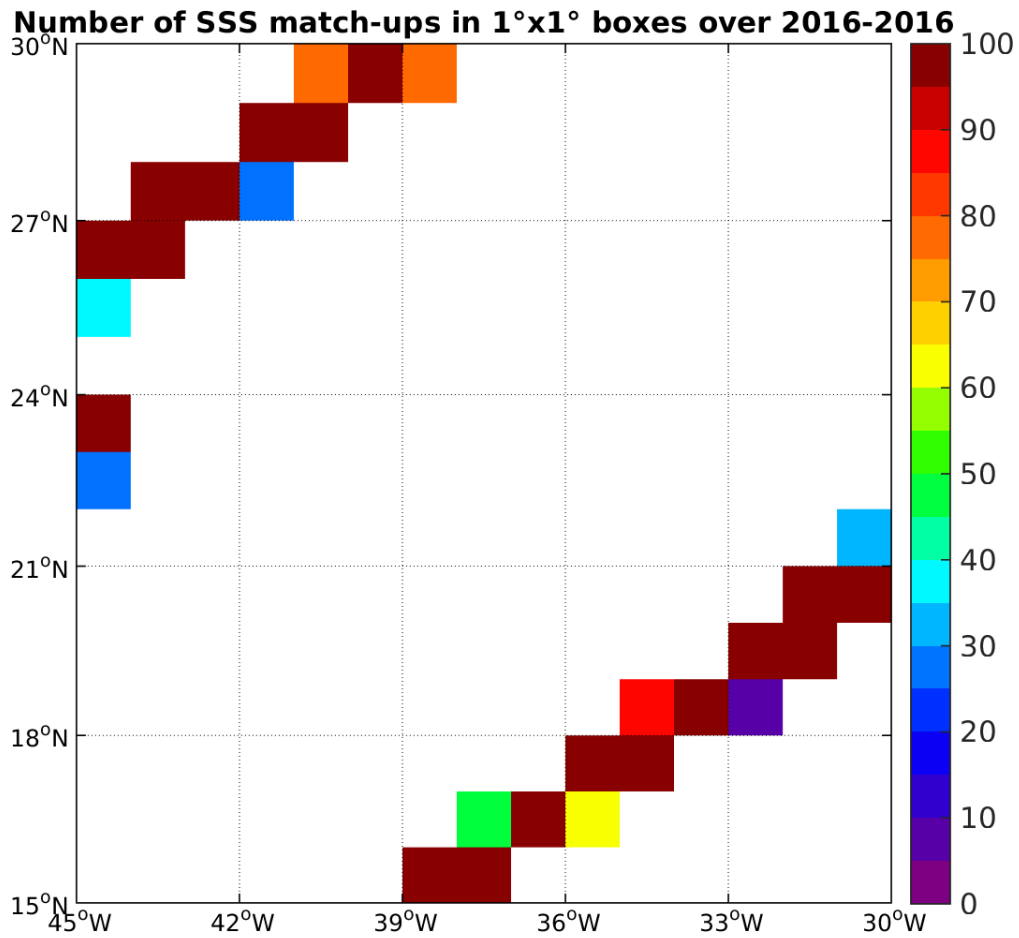
Figure 4: Number of SSS match-ups between TSG-GOSUD-Research-vessel SSS and the SMAP-L3-RSS-V2-MONTHLY-0.25DEG-40KM SSS product for the SPURS 1 Pi-MEP region over 1°x1° boxes and for the full satellite product period.
