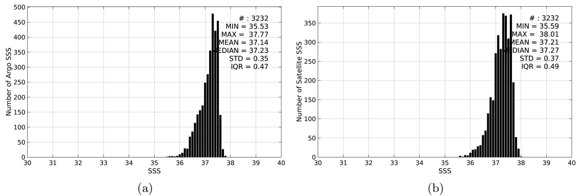
Figure 2: Histograms of SSS from Argo (a) and SMAP-L3-RSS-V2-MONTHLY-0.25DEG-40KM (b) considering all match-up pairs per bins of 0.1 over the SPURS 1 Pi-MEP region and for the full satellite product period.
