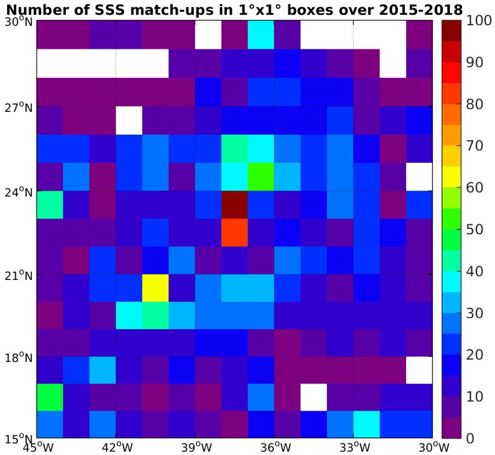
Figure 4: Number of SSS match-ups between Argo SSS and the SMAP-L3-RSS-V2-MONTHLY-0.25DEG-40KM SSS product for the SPURS 1 Pi-MEP region over 1°x1° boxes and for the full satellite product period.
