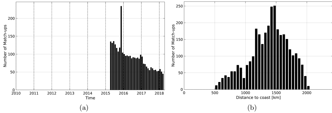
Figure 1: Number of match-ups between Argo and SMAP-L3-RSS-V2-MONTHLY-0.25DEG-40KM SSS as a function of time (a) and as function of the distance to coast (b) over the SPURS 1 Pi-MEP region and for the full satellite product period.
