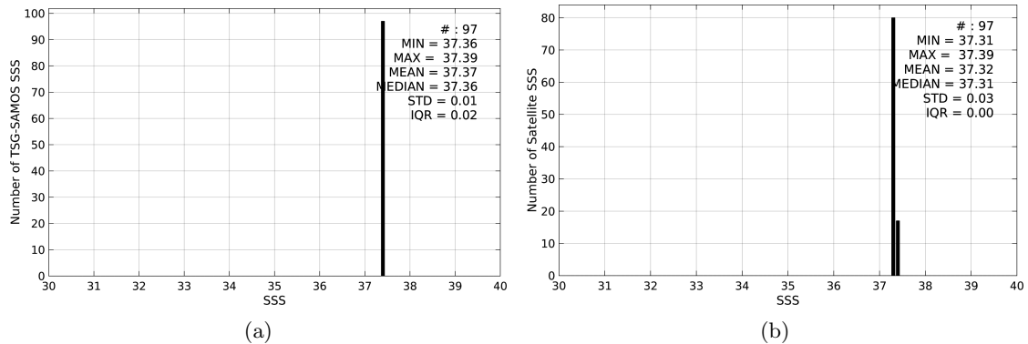
Figure 2: Histograms of SSS from TSG-SAMOS (a) and SMAP-L3-RSS-V2-MONTHLY-70KM (b) considering all match-up pairs per bins of 0.1 over the SPURS 1 Pi-MEP region and for the full satellite product period.
