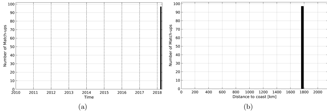
Figure 1: Number of match-ups between TSG-SAMOS and SMAP-L3-RSS-V2-MONTHLY-70KM SSS as a function of time (a) and as function of the distance to coast (b) over the SPURS 1 Pi-MEP region and for the full satellite product period.
