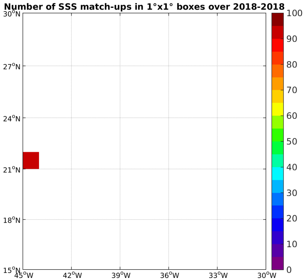
Figure 4: Number of SSS match-ups between TSG-SAMOS SSS and the SMAP-L3-RSS-V2-MONTHLY-70KM SSS product for the SPURS 1 Pi-MEP region over 1°x1° boxes and for the full satellite product period.
