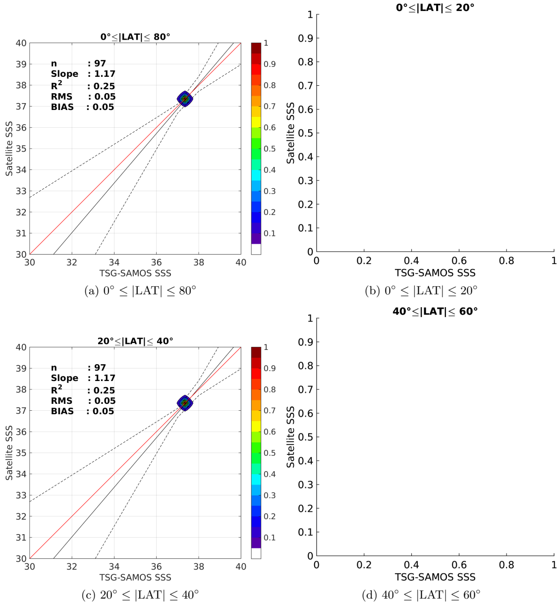
Figure 9: Contour maps of the concentration of SMAP-L3-RSS-V2-MONTHLY-70KM SSS (y-axis) versus TSG-SAMOS SSS (x-axis) at match-up pairs for different latitude bands. For each plot, the red line shows x=y . The black thin and dashed lines indicate a linear fit through the data cloud and the \pm 95\% confidence levels, respectively. The number match-up pairs n , the slope and R^2 coefficient of the linear fit, the root mean square (RMS) and the mean bias between satellite and in situ data are indicated for each latitude band in each plots.
