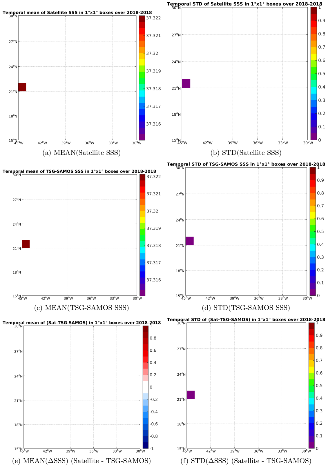
Figure 6: Temporal mean (left) and STD (right) of SSS from SMAP-L3-RSS-V2-MONTHLY-70KM (top), TSG-SAMOS (middle), and of \Delta SSS (Satellite - TSG-SAMOS). Only match-up pairs are used to generate these maps.
