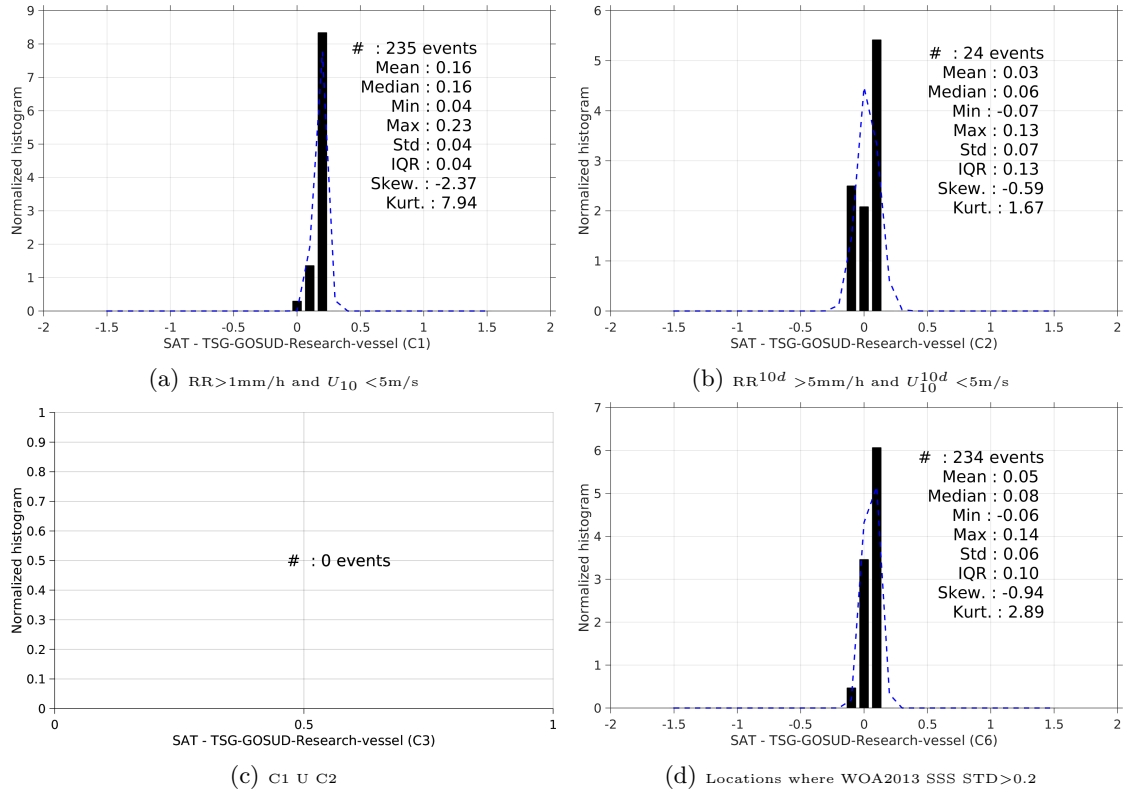
Figure 13: Normalized histogram of \Delta\text{SSS} (SMAP-L3-RSS-V2-MONTHLY-70KM - TSG-GOSUD-Research-vessel) for 6 different subdatasets corresponding to: RR > 1\text{mm/h} and U_{10} < 5\text{m/s} (a), RR^{10d} > 5\text{mm/h} and U_{10}^{10d} < 5\text{m/s} (b), C1 U C2 (c), Locations where WOA2013 SSS STD > 0.2 (d).
