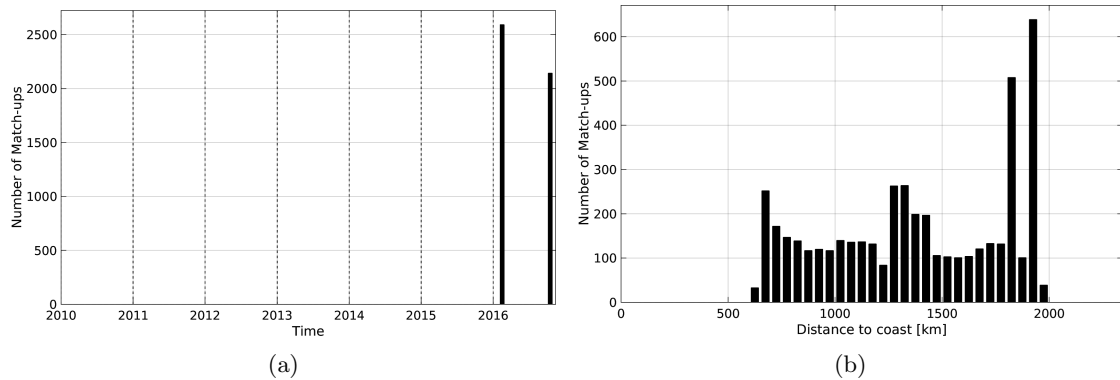
Figure 1: Number of match-ups between TSG-GOSUD-Research-vessel and SMAP-L3-RSS-V2-MONTHLY-70KM SSS as a function of time (a) and as function of the distance to coast (b) over the SPURS 1 Pi-MEP region and for the full satellite product period.
