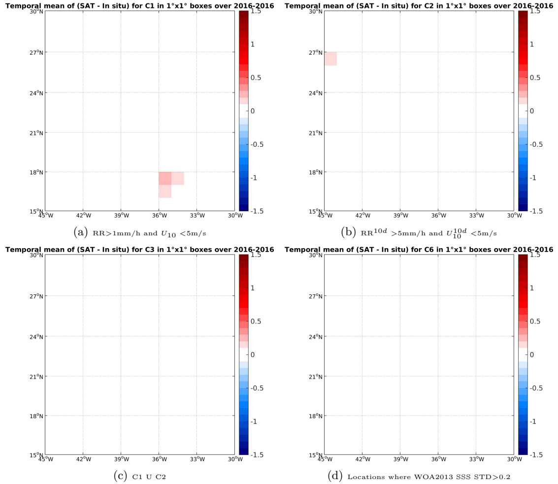
Figure 12: Temporal mean gridded over spatial boxes of size 1^\circ \times 1^\circ of \Delta SSS (SMAP-L3-RSS-V2-MONTHLY-70KM - TSG-GOSUD-Research-vessel) for 4 different subdatasets corresponding to: RR > 1\text{mm/h} and U_{10} < 5\text{m/s} (a), RR^{10d} > 5\text{mm/h} and U_{10}^{10d} < 5\text{m/s} (b), C1 U C2 (c), Locations where WOA2013 SSS STD > 0.2 (d).
