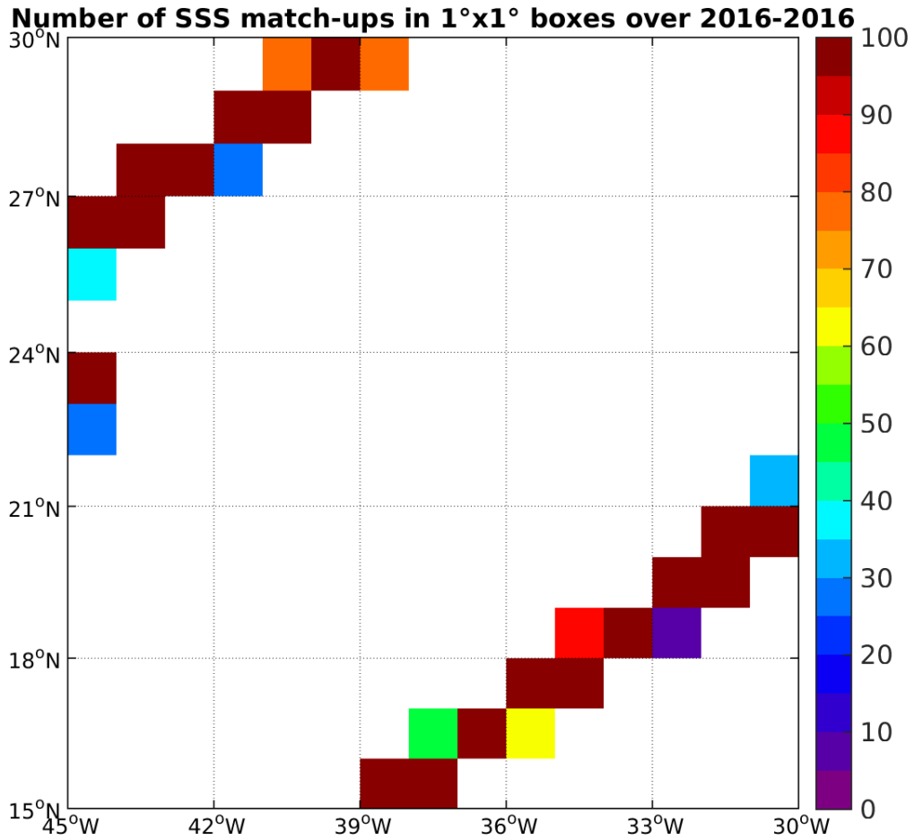
Figure 4: Number of SSS match-ups between TSG-GOSUD-Research-vessel SSS and the SMAP-L3-RSS-V2-MONTHLY-70KM SSS product for the SPURS 1 Pi-MEP region over 1°x1° boxes and for the full satellite product period.
