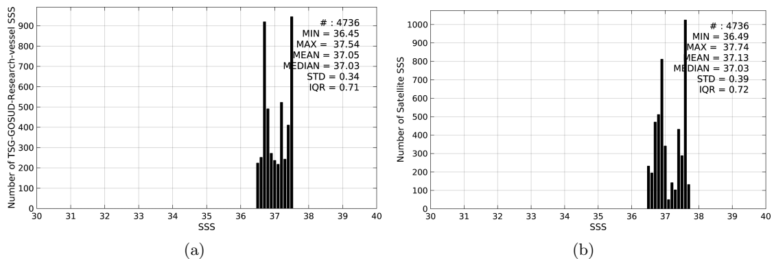
Figure 2: Histograms of SSS from TSG-GOSUD-Research-vessel (a) and SMAP-L3-RSS-V2-MONTHLY-70KM (b) considering all match-up pairs per bins of 0.1 over the SPURS 1 Pi-MEP region and for the full satellite product period.
