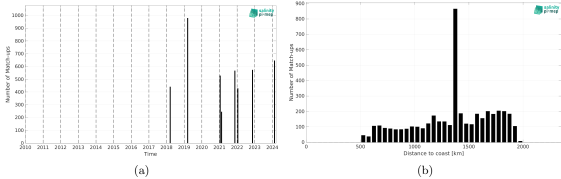
Figure 2: Number of match-ups between TSG (SAMOS) and SMAP SSS L3 v5.0 - 8-Day running (JPL) SSS as a function of time (a) and as function of the distance to coast (b) over the SPURS 1 Pi-MEP region and for the full satellite product period.
