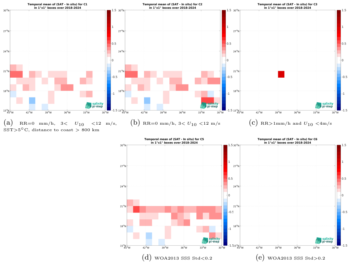
Figure 14: Temporal mean gridded over spatial boxes of size 1^\circ \times 1^\circ of \Delta\text{SSS} (SMAP SSS L3 v5.0 - 8-Day running (JPL) - TSG (SAMOS)) for 5 different subdatasets corresponding to: \text{RR}=0 mm/h, 3 < U_{10} < 12 m/s, \text{SST} > 5^\circ\text{C} , distance to coast > 800 km (a), \text{RR}=0 mm/h, 3 < U_{10} < 12 m/s (b), \text{RR} > 1\text{mm/h} and U_{10} < 4\text{m/s} (c), WOA2013 SSS Std < 0.2 (d), WOA2013 SSS Std > 0.2 (e).
