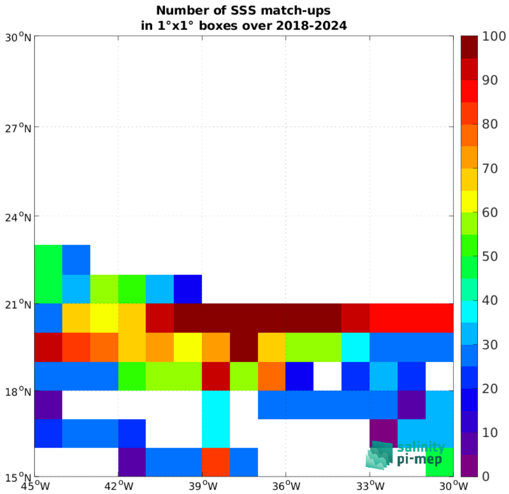
Figure 5: Number of SSS match-ups between TSG (SAMOS) SSS and the SMAP SSS L3 v5.0 - 8-Day running (JPL) SSS product for the SPURS 1 Pi-MEP region over 1^\circ \times 1^\circ boxes and for the full satellite product period.
