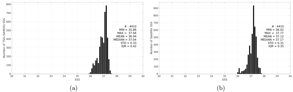
Figure 3: Histograms of SSS from TSG (SAMOS) (a) and SMAP SSS L3 v5.0 - 8-Day running (JPL) (b) considering all match-up pairs per bins of 0.1 over the SPURS 1 Pi-MEP region and for the full satellite product period.
