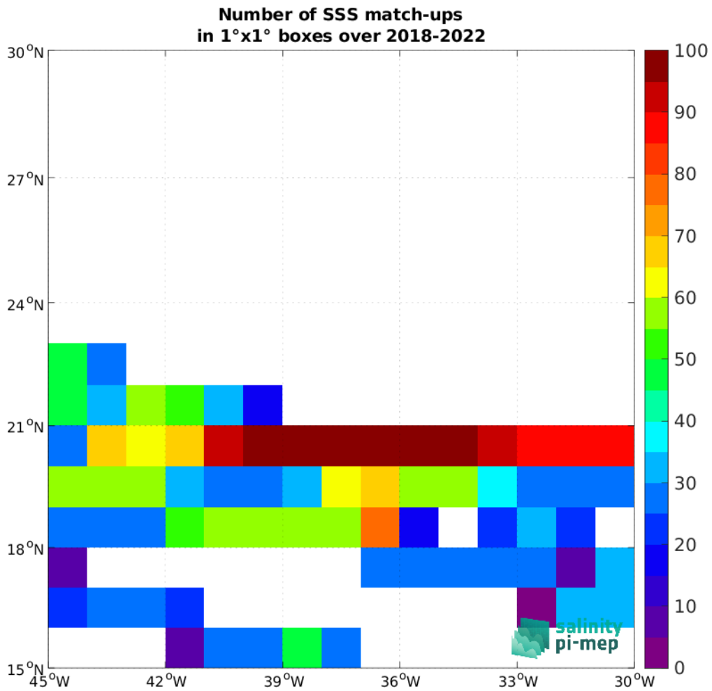
Figure 4: Number of SSS match-ups between TSG (SAMOS) SSS and the SMAP SSS L3 v5.0 - 8-Day running (JPL) SSS product for the SPURS 1 Pi-MEP region over 1°x1° boxes and for the full satellite product period.
