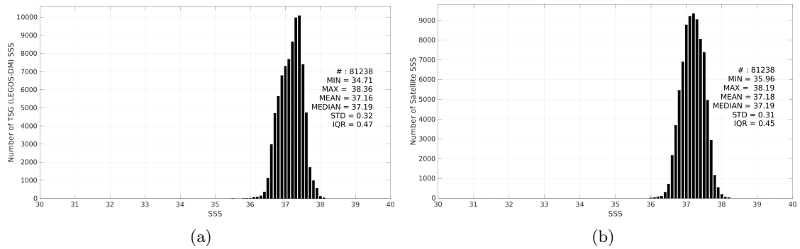
Figure 3: Histograms of SSS from TSG (LEGOS-DM) (a) and SMAP SSS L3 v5.0 - 8-Day running (JPL) (b) considering all match-up pairs per bins of 0.1 over the SPURS 1 Pi-MEP region and for the full satellite product period.
