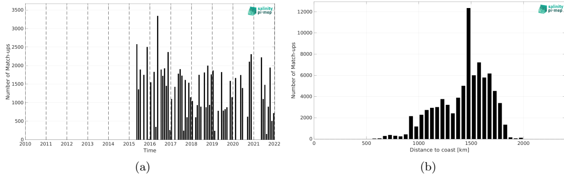
Figure 2: Number of match-ups between TSG (LEGOS-DM) and SMAP SSS L3 v5.0 - 8-Day running (JPL) SSS as a function of time (a) and as function of the distance to coast (b) over the SPURS 1 Pi-MEP region and for the full satellite product period.
