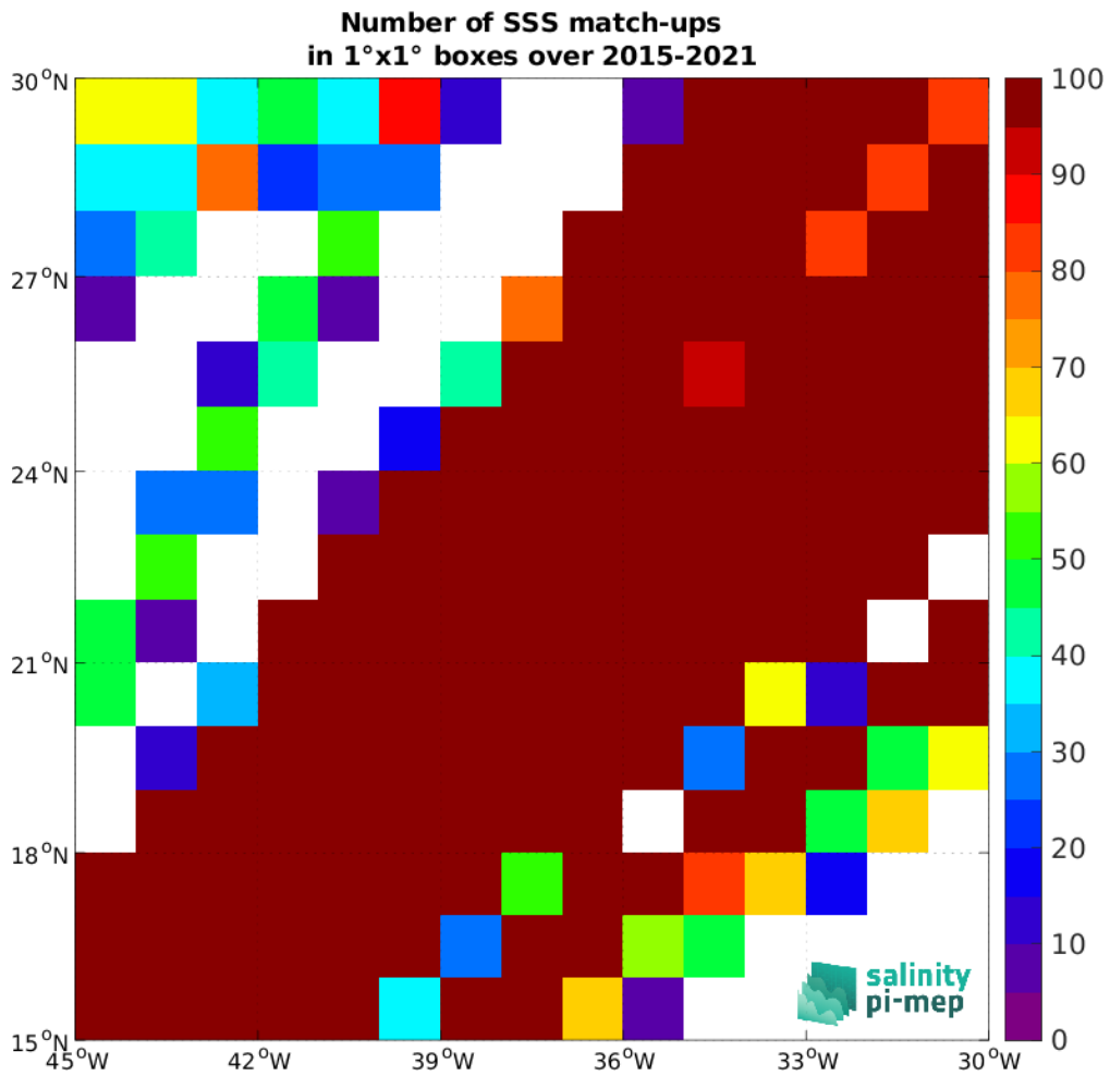
Figure 5: Number of SSS match-ups between TSG (LEGOS-DM) SSS and the SMAP SSS L3 v5.0 - 8-Day running (JPL) SSS product for the SPURS 1 Pi-MEP region over 1°x1° boxes and for the full satellite product period.
