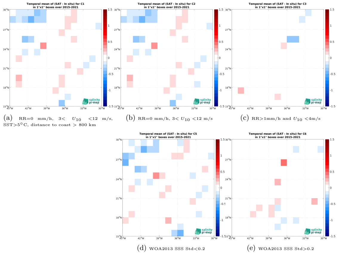
Figure 12: Temporal mean gridded over spatial boxes of size 1^\circ \times 1^\circ of \Delta\text{SSS} (SMAP SSS L3 v5.0 - 8-Day running (JPL) - TSG (LEGOS-DM)) for 5 different subdatasets corresponding to:RR=0 mm/h, 3 < U_{10} < 12 m/s, SST >5^\circ\text{C} , distance to coast > 800 km (a), RR=0 mm/h, 3 < U_{10} < 12 m/s (b), RR >1 mm/h and U_{10} < 4 m/s (c), WOA2013 SSS Std <0.2 (d), WOA2013 SSS Std >0.2 (e).
