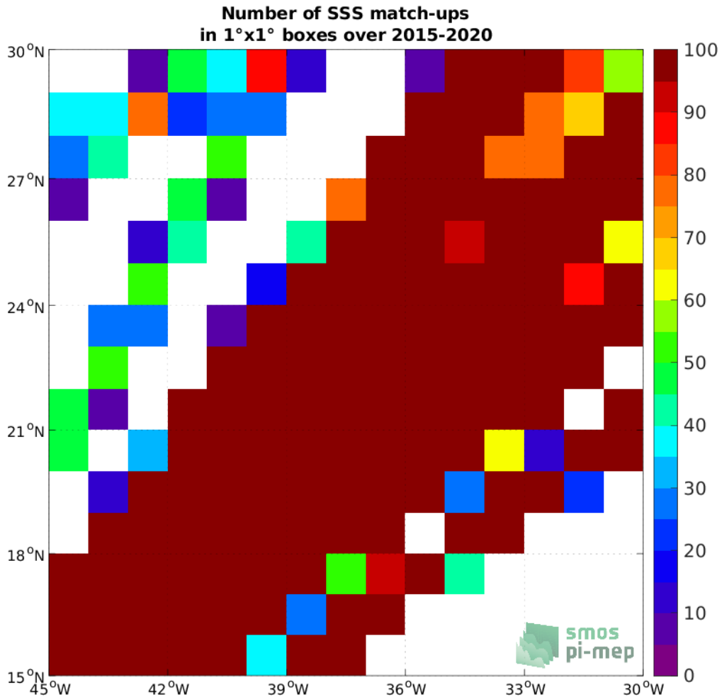
Figure 4: Number of SSS match-ups between TSG (LEGOS-DM) SSS and the SMAP SSS L3 v5.0 - 8-Day running (JPL) SSS product for the SPURS 1 Pi-MEP region over 1°×1° boxes and for the full satellite product period.
