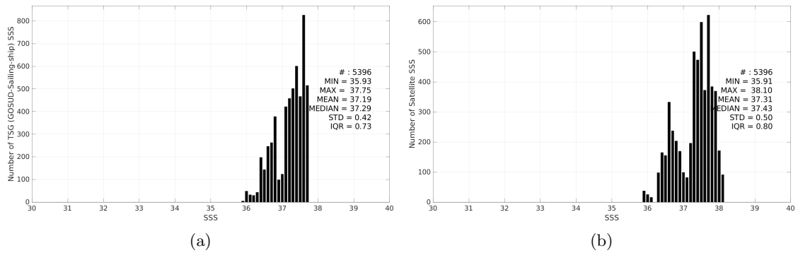
Figure 3: Histograms of SSS from TSG (GOSUD-Sailing-ship) (a) and SMAP SSS L3 v5.0 - 8-Day running (JPL) (b) considering all match-up pairs per bins of 0.1 over the SPURS 1 Pi-MEP region and for the full satellite product period.
