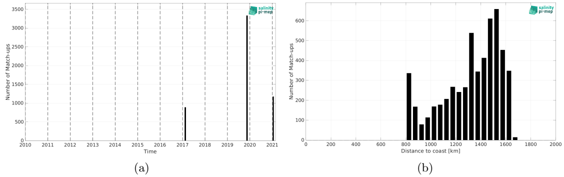
Figure 2: Number of match-ups between TSG (GOSUD-Sailing-ship) and SMAP SSS L3 v5.0 - 8-Day running (JPL) SSS as a function of time (a) and as function of the distance to coast (b) over the SPURS 1 Pi-MEP region and for the full satellite product period.
