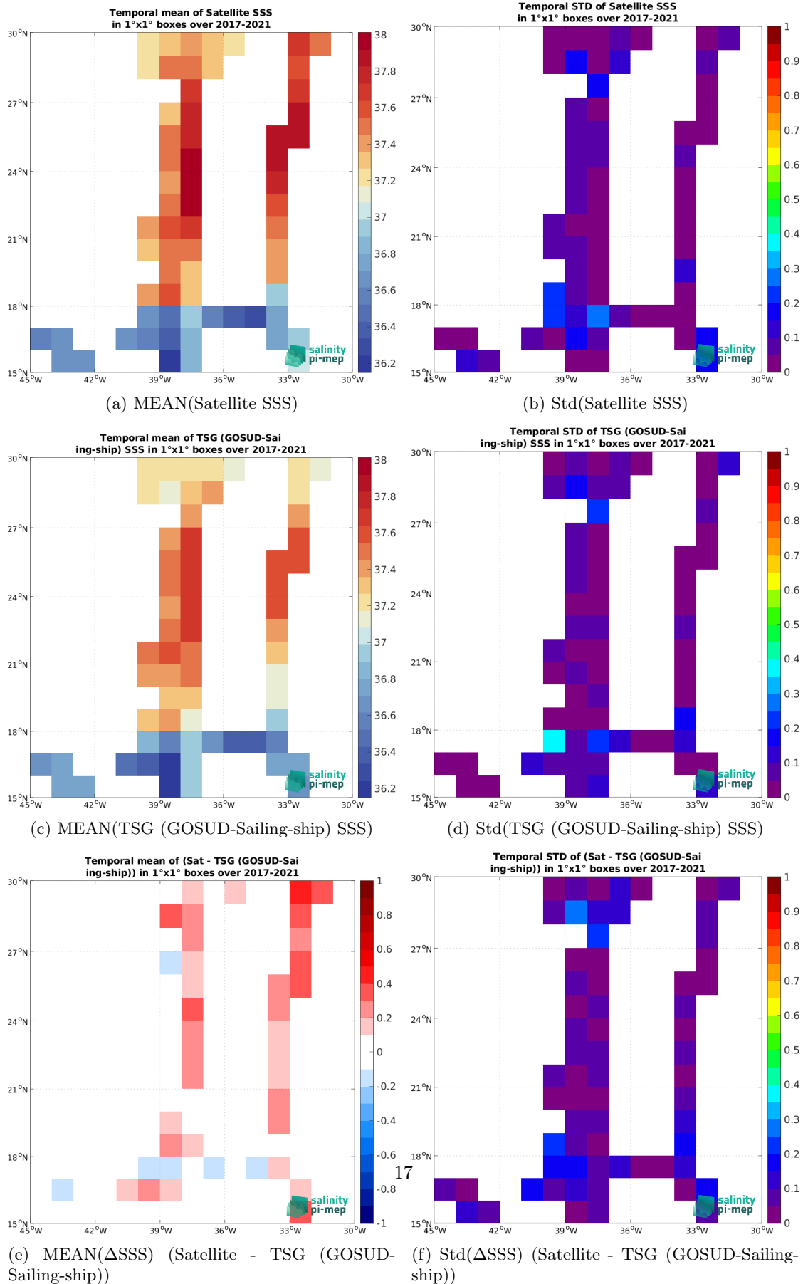
Figure 7: Temporal mean (left) and Std (right) of SSS from SMAP SSS L3 v5.0 - 8-Day running (JPL) (top), TSG (GOSUD-Sailing-ship) (middle), and of \Delta SSS (Satellite - TSG (GOSUD-Sailing-ship)). Only match-up pairs are used to generate these maps.
