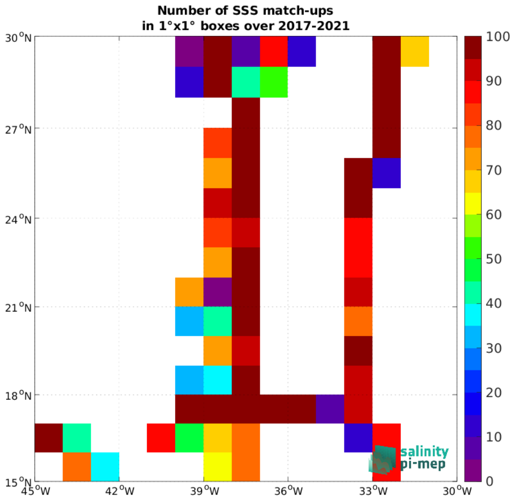
Figure 5: Number of SSS match-ups between TSG (GOSUD-Sailing-ship) SSS and the SMAP SSS L3 v5.0 - 8-Day running (JPL) SSS product for the SPURS 1 Pi-MEP region over 1°x1° boxes and for the full satellite product period.
