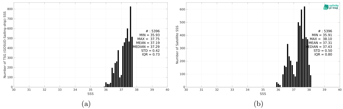
Figure 2: Histograms of SSS from TSG (GOSUD-Sailing-ship) (a) and SMAP SSS L3 v5.0 - 8-Day running (JPL) (b) considering all match-up pairs per bins of 0.1 over the SPURS 1 Pi-MEP region and for the full satellite product period.
