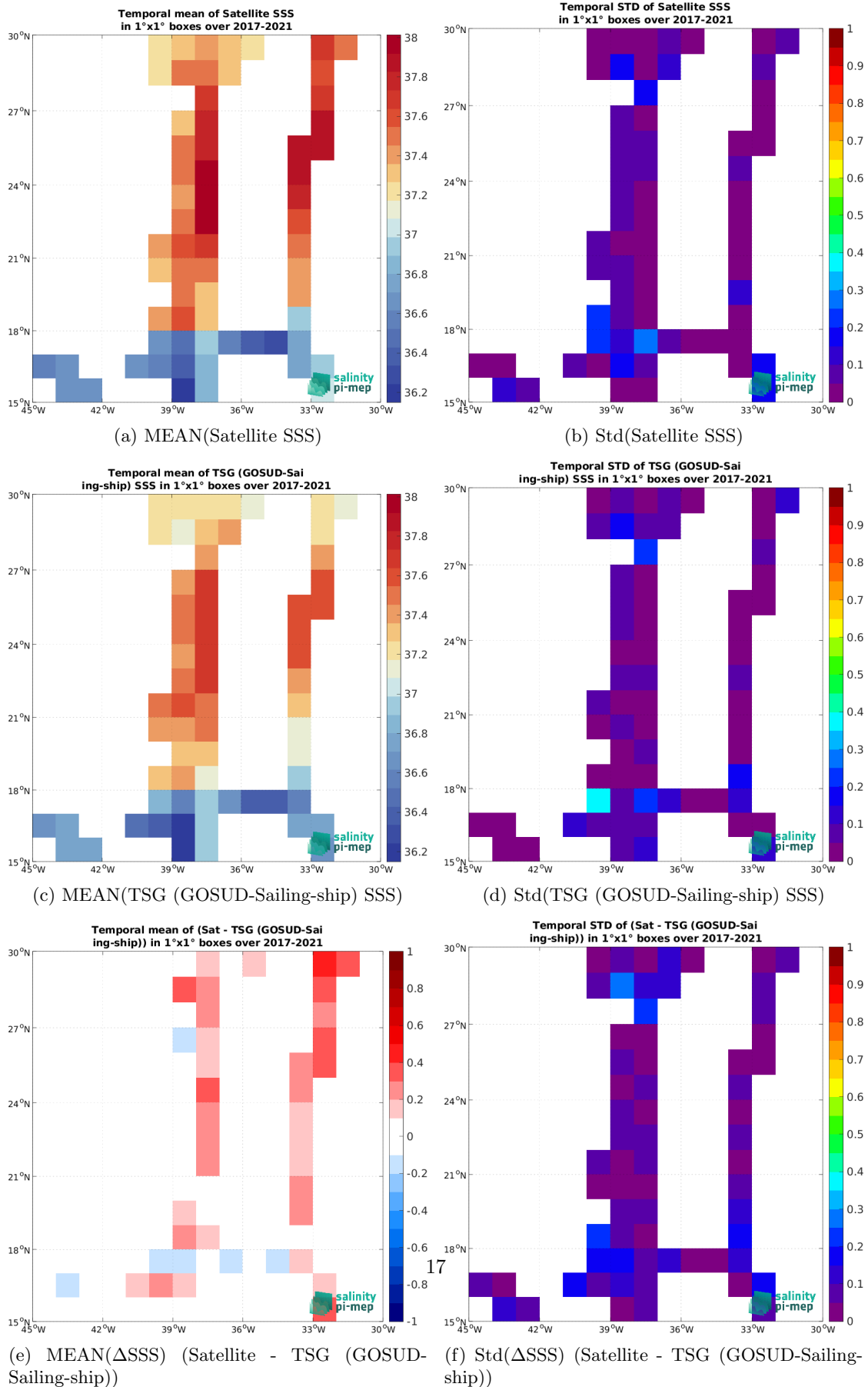
Figure 6: Temporal mean (left) and Std (right) of SSS from SMAP SSS L3 v5.0 - 8-Day running (JPL) (top), TSG (GOSUD-Sailing-ship) (middle), and of \Delta SSS (Satellite - TSG (GOSUD-Sailing-ship)). Only match-up pairs are used to generate these maps.
