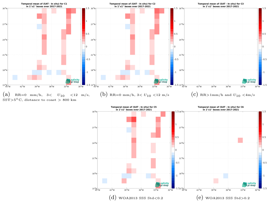
Figure 12: Temporal mean gridded over spatial boxes of size 1^\circ \times 1^\circ of \Delta\text{SSS} (SMAP SSS L3 v5.0 - 8-Day running (JPL) - TSG (GOSUD-Sailing-ship)) for 5 different subdatasets corresponding to:RR=0 mm/h, 3 < U_{10} < 12 m/s, SST>5°C, distance to coast > 800 km (a), RR=0 mm/h, 3 < U_{10} < 12 m/s (b), RR>1mm/h and U_{10} < 4 m/s (c), WOA2013 SSS Std<0.2 (d), WOA2013 SSS Std>0.2 (e).
