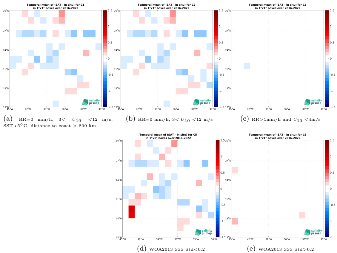
Figure 14: Temporal mean gridded over spatial boxes of size 1^\circ \times 1^\circ of \Delta SSS (SMAP SSS L3 v5.0 - 8-Day running (JPL) - TSG (GOSUD-Research-vessel)) for 5 different subdatasets corresponding to: RR=0 mm/h, 3 < U_{10} < 12 m/s, SST > 5^\circ C , distance to coast > 800 km (a), RR=0 mm/h, 3 < U_{10} < 12 m/s (b), RR > 1 mm/h and U_{10} < 4 m/s (c), WOA2013 SSS Std < 0.2 (d), WOA2013 SSS Std > 0.2 (e).
