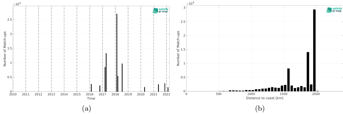
Figure 2: Number of match-ups between TSG (GOSUD-Research-vessel) and SMAP SSS L3 v5.0 - 8-Day running (JPL) SSS as a function of time (a) and as function of the distance to coast (b) over the SPURS 1 Pi-MEP region and for the full satellite product period.
