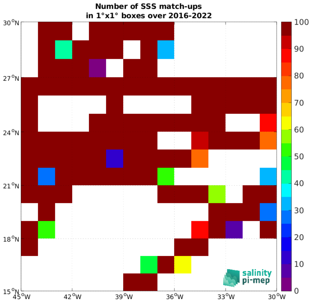
Figure 5: Number of SSS match-ups between TSG (GOSUD-Research-vessel) SSS and the SMAP SSS L3 v5.0 - 8-Day running (JPL) SSS product for the SPURS 1 Pi-MEP region over 1°x1° boxes and for the full satellite product period.
