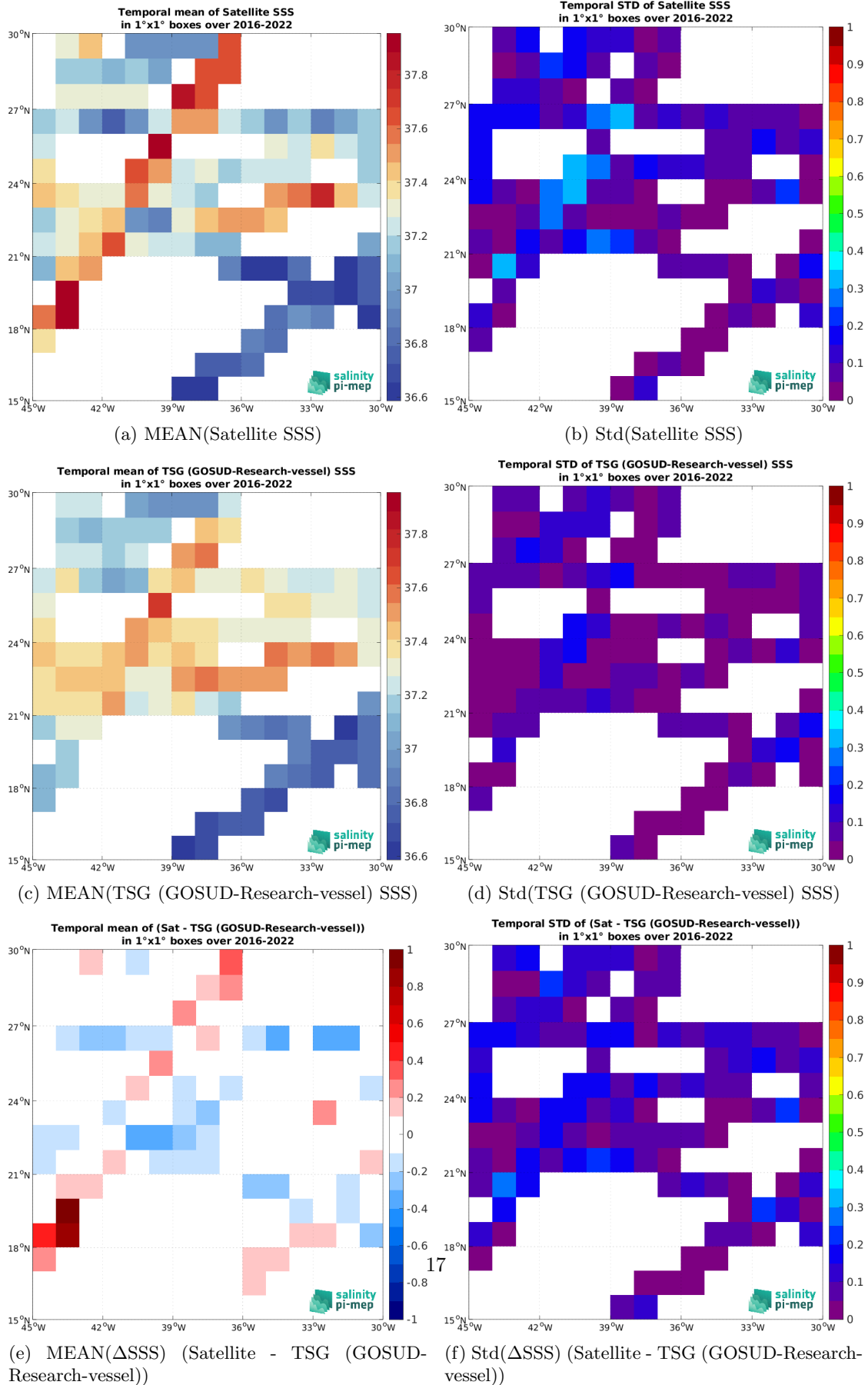
Figure 7: Temporal mean (left) and Std (right) of SSS from SMAP SSS L3 v5.0 - 8-Day running (JPL) (top), TSG (GOSUD-Research-vessel) (middle), and of \Delta SSS (Satellite - TSG (GOSUD-Research-vessel)). Only match-up pairs are used to generate these maps.
