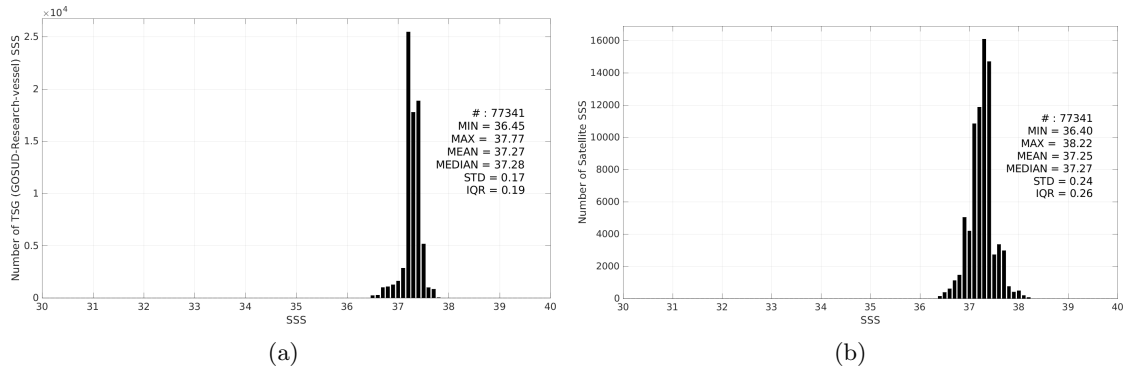
Figure 3: Histograms of SSS from TSG (GOSUD-Research-vessel) (a) and SMAP SSS L3 v5.0 - 8-Day running (JPL) (b) considering all match-up pairs per bins of 0.1 over the SPURS 1 Pi-MEP region and for the full satellite product period.
