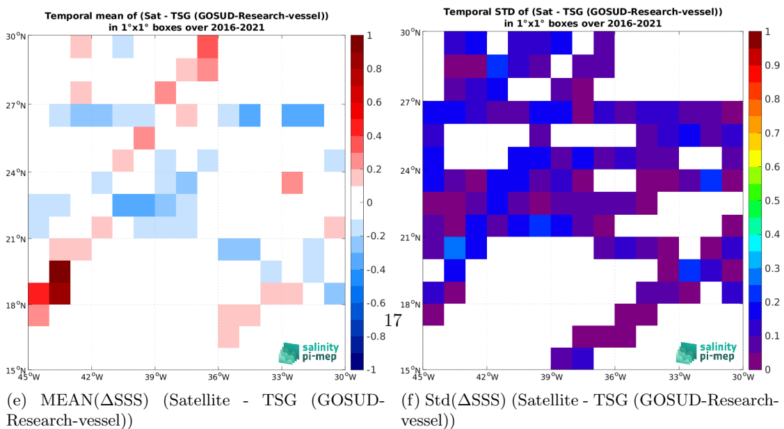
Figure 7: Temporal mean (left) and Std (right) of SSS from SMAP SSS L3 v5.0 - 8-Day running (JPL) (top), TSG (GOSUD-Research-vessel) (middle), and of \Delta SSS (Satellite - TSG (GOSUD-Research-vessel)). Only match-up pairs are used to generate these maps.
