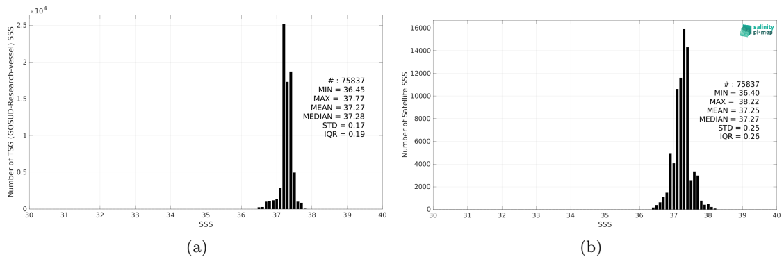
Figure 2: Histograms of SSS from TSG (GOSUD-Research-vessel) (a) and SMAP SSS L3 v5.0 - 8-Day running (JPL) (b) considering all match-up pairs per bins of 0.1 over the SPURS 1 Pi-MEP region and for the full satellite product period.
