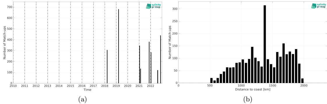
Figure 2: Number of match-ups between TSG (SAMOS) and SMAP SSS L3 v5.0 - Monthly (JPL) SSS as a function of time (a) and as function of the distance to coast (b) over the SPURS 1 Pi-MEP region and for the full satellite product period.
