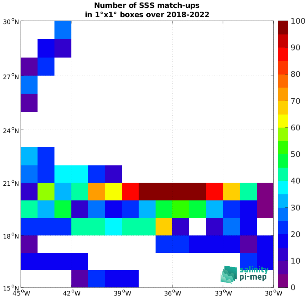
Figure 5: Number of SSS match-ups between TSG (SAMOS) SSS and the SMAP SSS L3 v5.0 - Monthly (JPL) SSS product for the SPURS 1 Pi-MEP region over 1^\circ \times 1^\circ boxes and for the full satellite product period.
