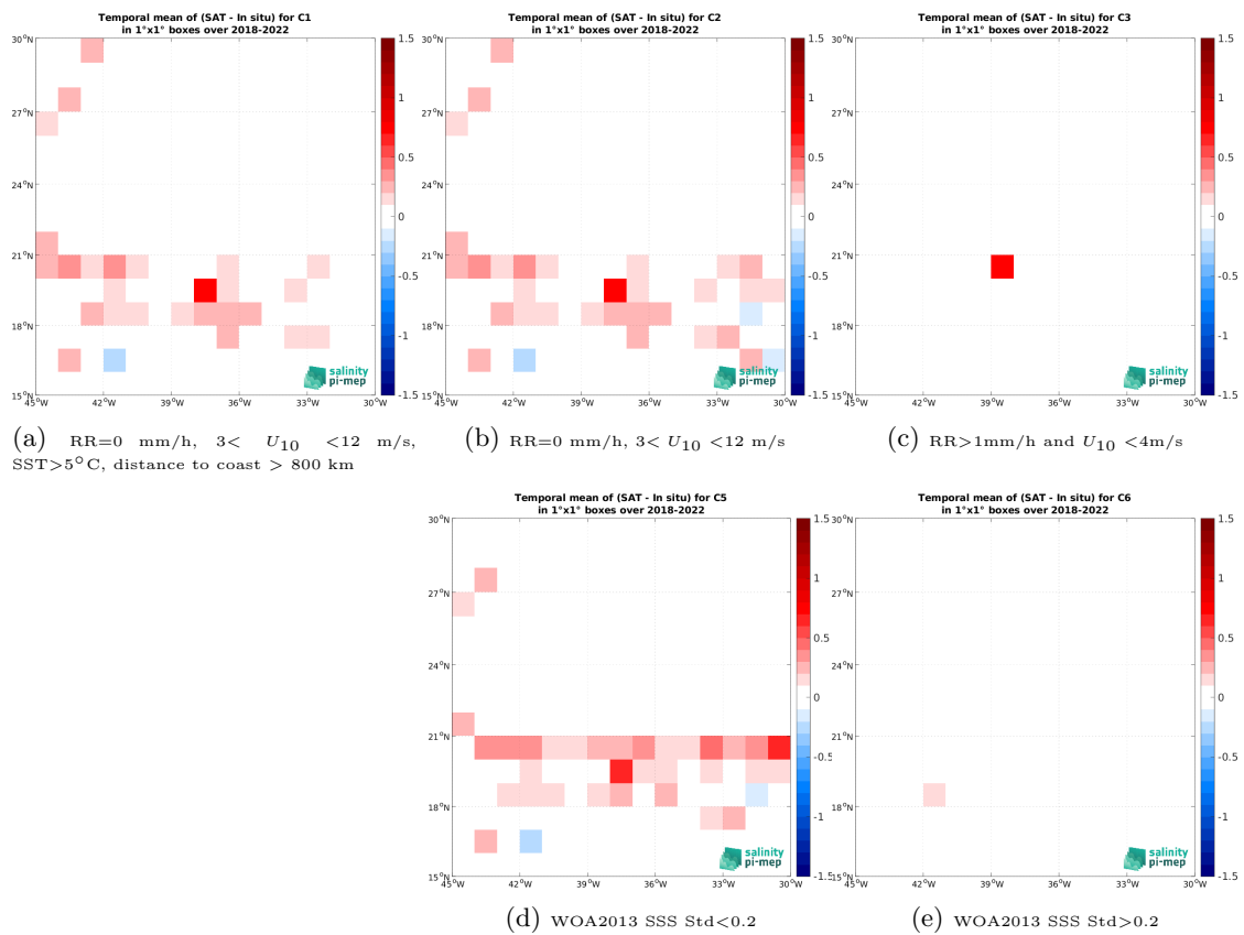
Figure 14: Temporal mean gridded over spatial boxes of size 1^\circ \times 1^\circ of \Delta SSS (SMAP SSS L3 v5.0 - Monthly (JPL) - TSG (SAMOS)) for 5 different subdatasets corresponding to: RR=0 mm/h, 3 < U_{10} < 12 m/s, SST > 5^\circ C , distance to coast > 800 km (a), RR=0 mm/h, 3 < U_{10} < 12 m/s (b), RR > 1 mm/h and U_{10} < 4 m/s (c), WOA2013 SSS Std < 0.2 (d), WOA2013 SSS Std > 0.2 (e).
