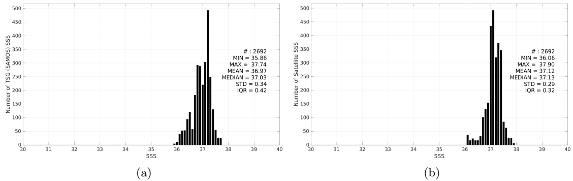
Figure 3: Histograms of SSS from TSG (SAMOS) (a) and SMAP SSS L3 v5.0 - Monthly (JPL) (b) considering all match-up pairs per bins of 0.1 over the SPURS 1 Pi-MEP region and for the full satellite product period.
