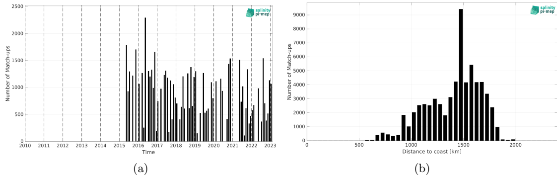
Figure 2: Number of match-ups between TSG (LEGOS-DM) and SMAP SSS L3 v5.0 - Monthly (JPL) SSS as a function of time (a) and as function of the distance to coast (b) over the SPURS 1 Pi-MEP region and for the full satellite product period.
