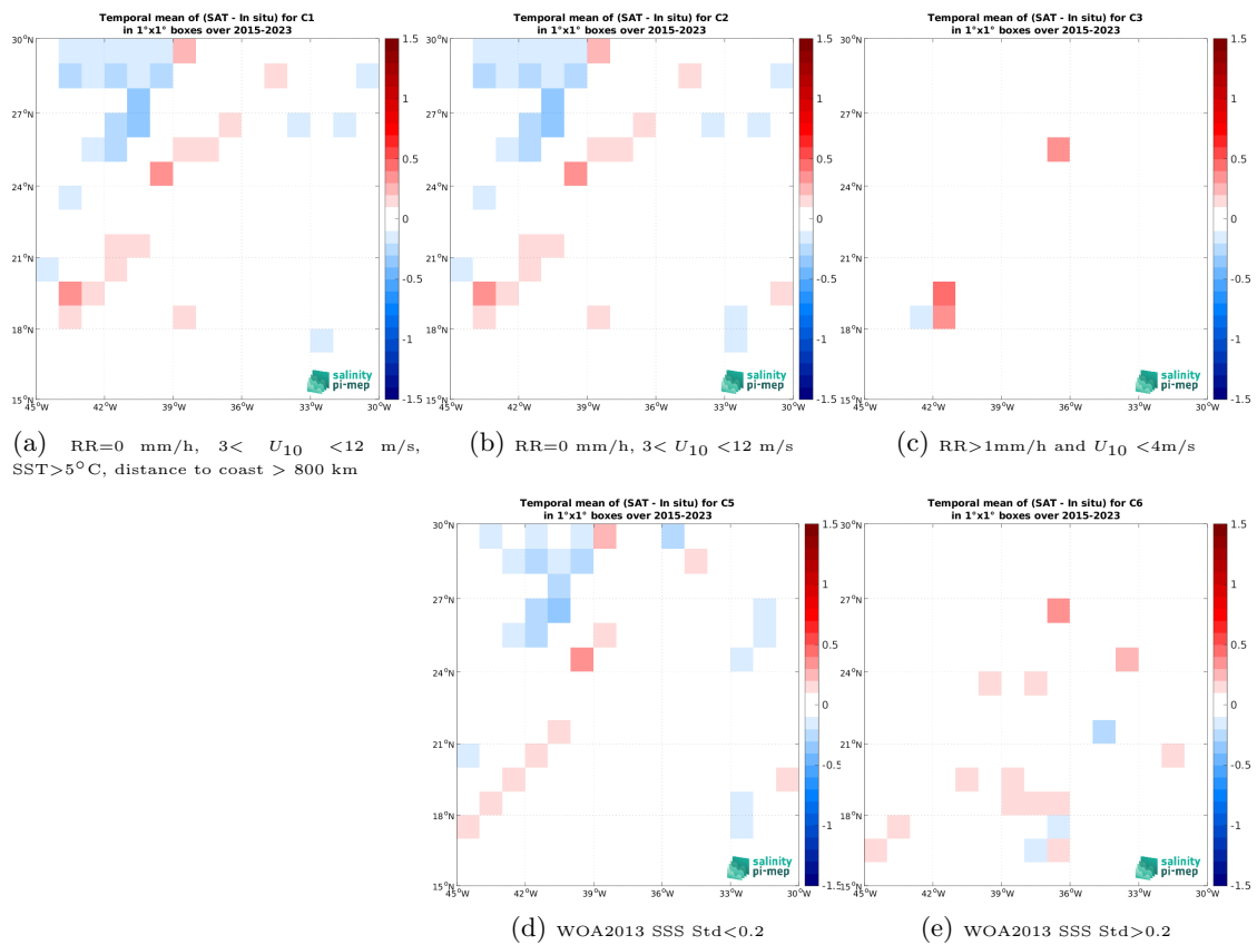
Figure 14: Temporal mean gridded over spatial boxes of size 1^\circ \times 1^\circ of \Delta SSS (SMAP SSS L3 v5.0 - Monthly (JPL) - TSG (LEGOS-DM)) for 5 different subdatasets corresponding to: RR=0 mm/h, 3 < U_{10} < 12 m/s, SST > 5^\circ C , distance to coast > 800 km (a), RR=0 mm/h, 3 < U_{10} < 12 m/s (b), RR > 1 mm/h and U_{10} < 4 m/s (c), WOA2013 SSS Std < 0.2 (d), WOA2013 SSS Std > 0.2 (e).
