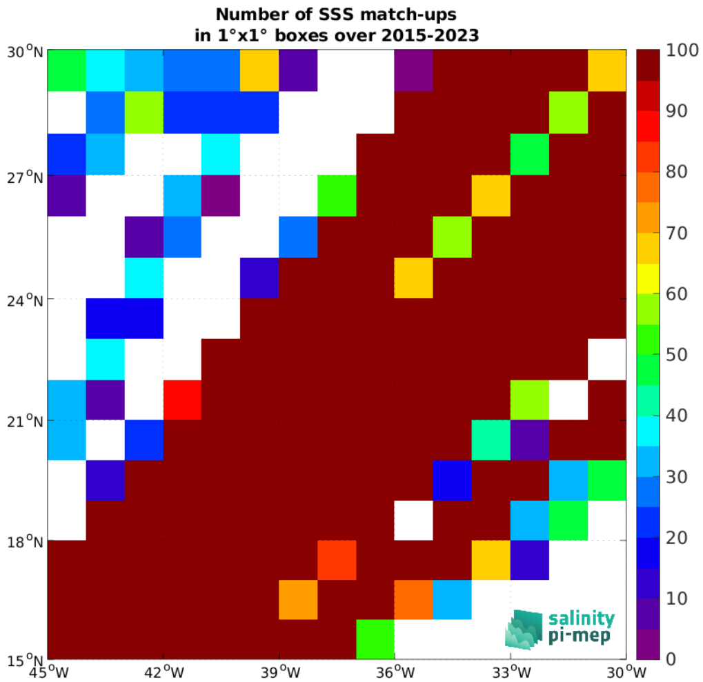
Figure 5: Number of SSS match-ups between TSG (LEGOS-DM) SSS and the SMAP SSS L3 v5.0 - Monthly (JPL) SSS product for the SPURS 1 Pi-MEP region over 1°x1° boxes and for the full satellite product period.
