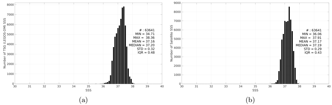
Figure 3: Histograms of SSS from TSG (LEGOS-DM) (a) and SMAP SSS L3 v5.0 - Monthly (JPL) (b) considering all match-up pairs per bins of 0.1 over the SPURS 1 Pi-MEP region and for the full satellite product period.
