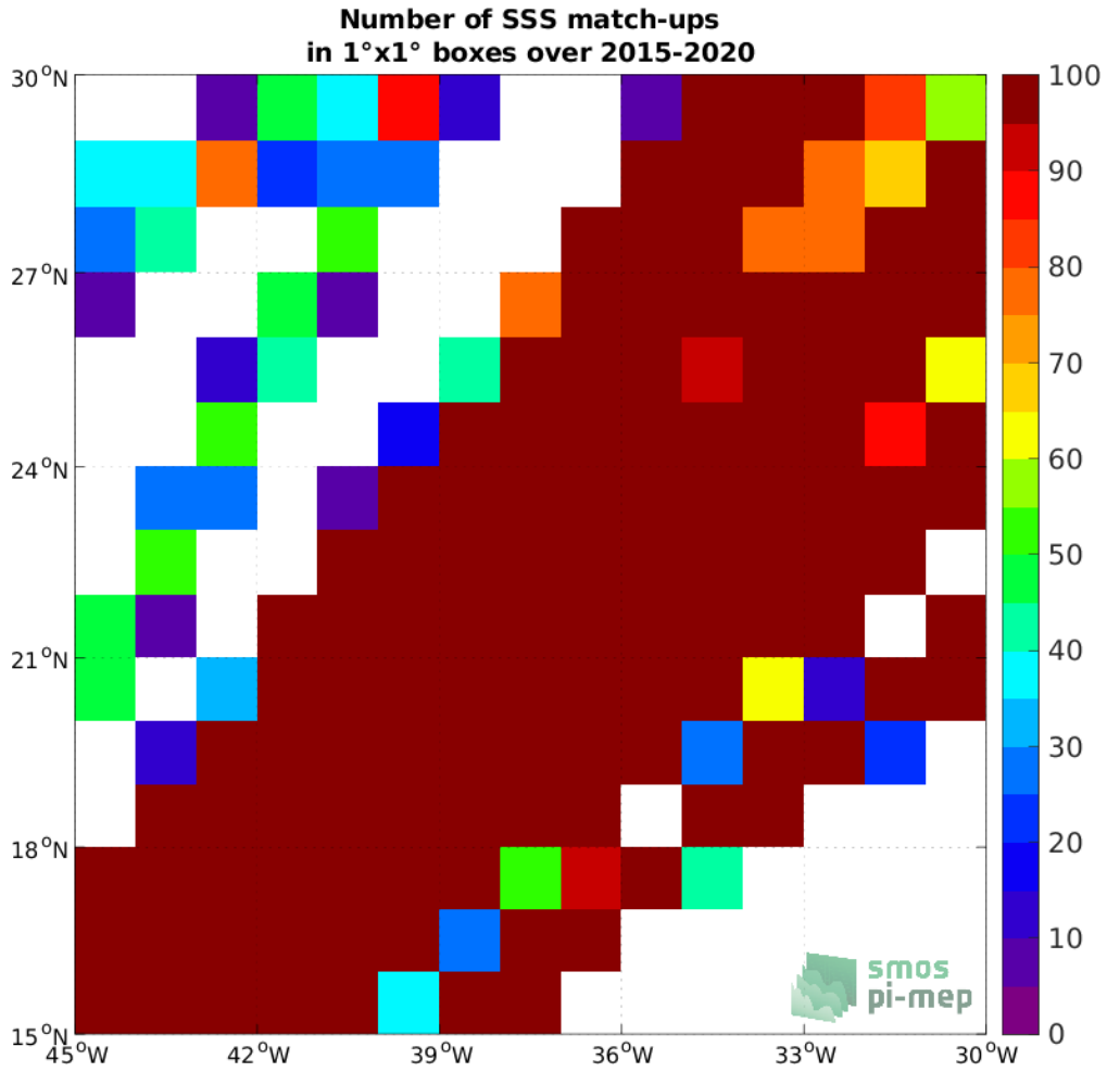
Figure 4: Number of SSS match-ups between TSG (LEGOS-DM) SSS and the SMAP SSS L3 v5.0 - Monthly (JPL) SSS product for the SPURS 1 Pi-MEP region over 1^\circ \times 1^\circ boxes and for the full satellite product period.
