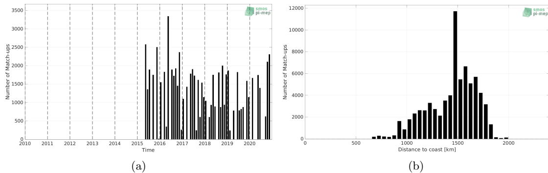
Figure 1: Number of match-ups between TSG (LEGOS-DM) and SMAP SSS L3 v5.0 - Monthly (JPL) SSS as a function of time (a) and as function of the distance to coast (b) over the SPURS 1 Pi-MEP region and for the full satellite product period.
