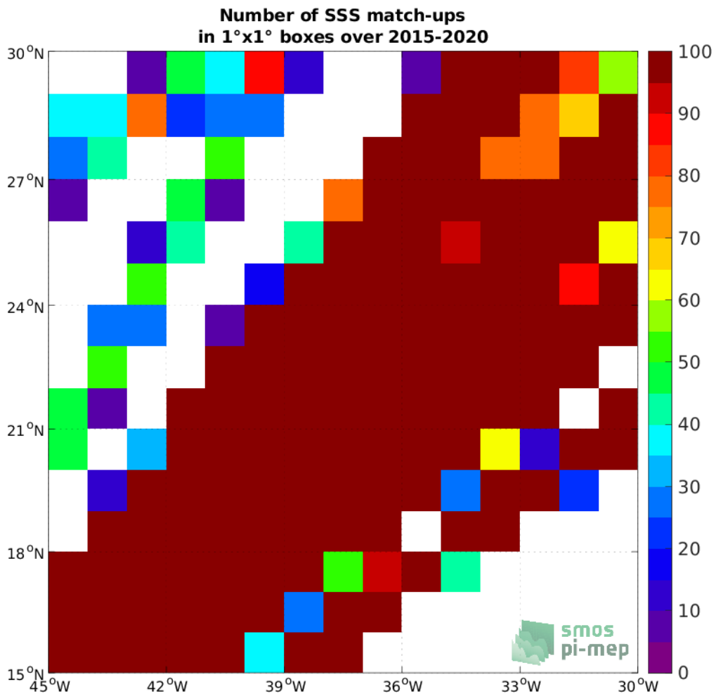
Figure 4: Number of SSS match-ups between TSG (LEGOS-DM) SSS and the SMAP SSS L3 v5.0 - Monthly (JPL) SSS product for the SPURS 1 Pi-MEP region over 1°x1° boxes and for the full satellite product period.
