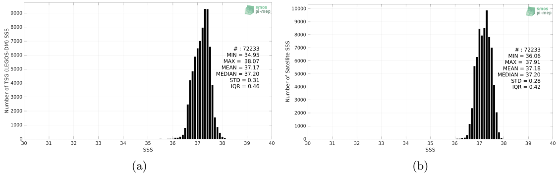
Figure 2: Histograms of SSS from TSG (LEGOS-DM) (a) and SMAP SSS L3 v5.0 - Monthly (JPL) (b) considering all match-up pairs per bins of 0.1 over the SPURS 1 Pi-MEP region and for the full satellite product period.
