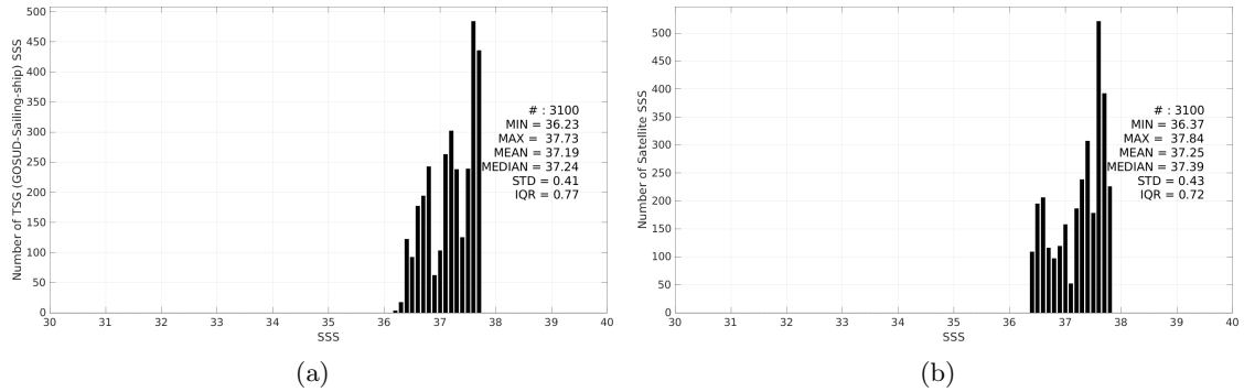
Figure 3: Histograms of SSS from TSG (GOSUD-Sailing-ship) (a) and SMAP SSS L3 v5.0 - Monthly (JPL) (b) considering all match-up pairs per bins of 0.1 over the SPURS 1 Pi-MEP region and for the full satellite product period.
