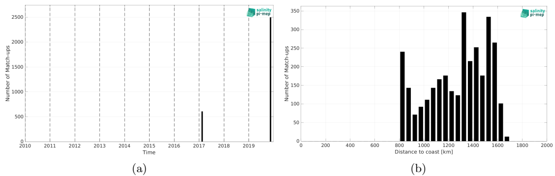
Figure 2: Number of match-ups between TSG (GOSUD-Sailing-ship) and SMAP SSS L3 v5.0 - Monthly (JPL) SSS as a function of time (a) and as function of the distance to coast (b) over the SPURS 1 Pi-MEP region and for the full satellite product period.
