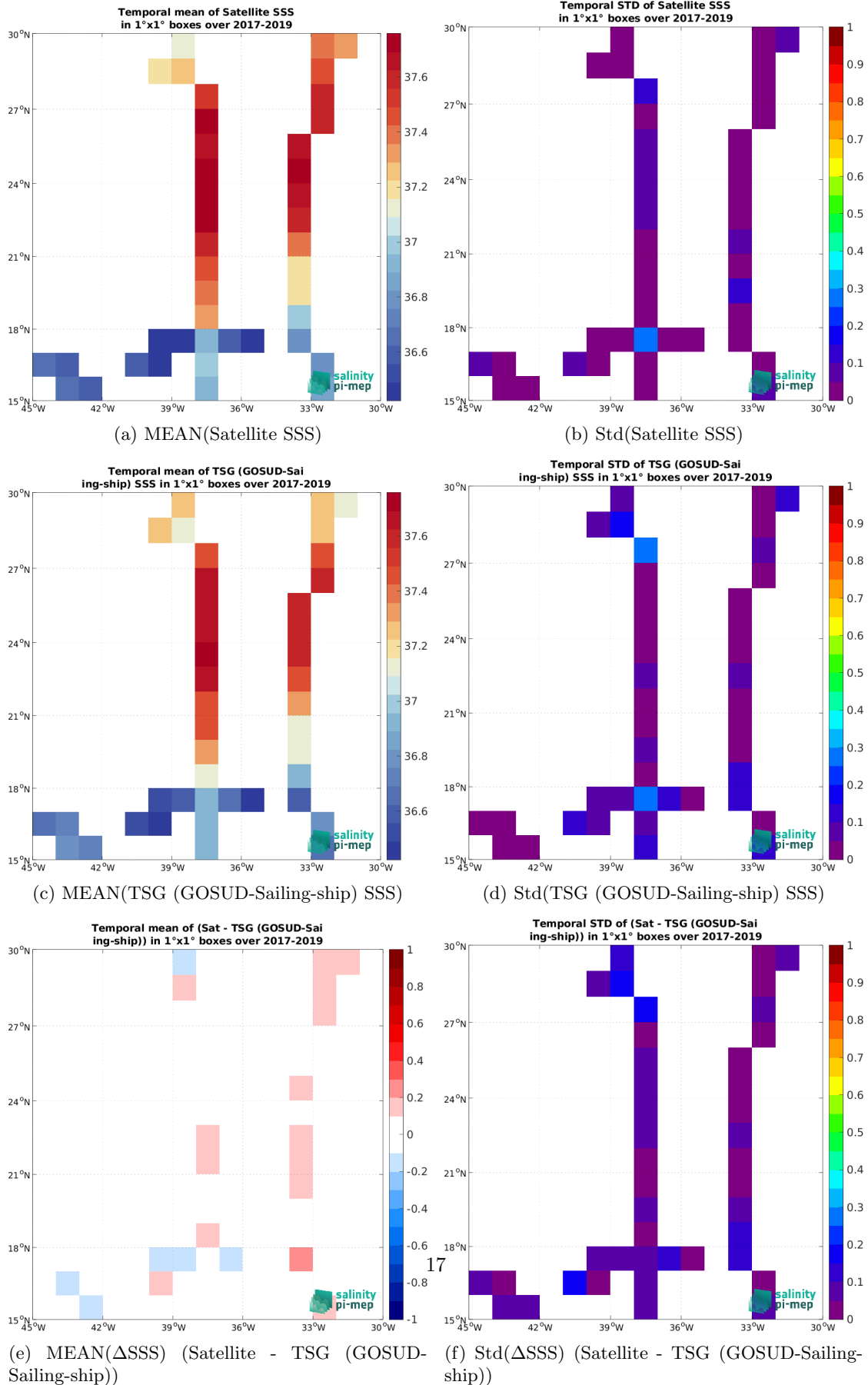
Figure 7: Temporal mean (left) and Std (right) of SSS from SMAP SSS L3 v5.0 - Monthly (JPL) (top), TSG (GOSUD-Sailing-ship) (middle), and of \Delta SSS (Satellite - TSG (GOSUD-Sailing-ship)). Only match-up pairs are used to generate these maps.
