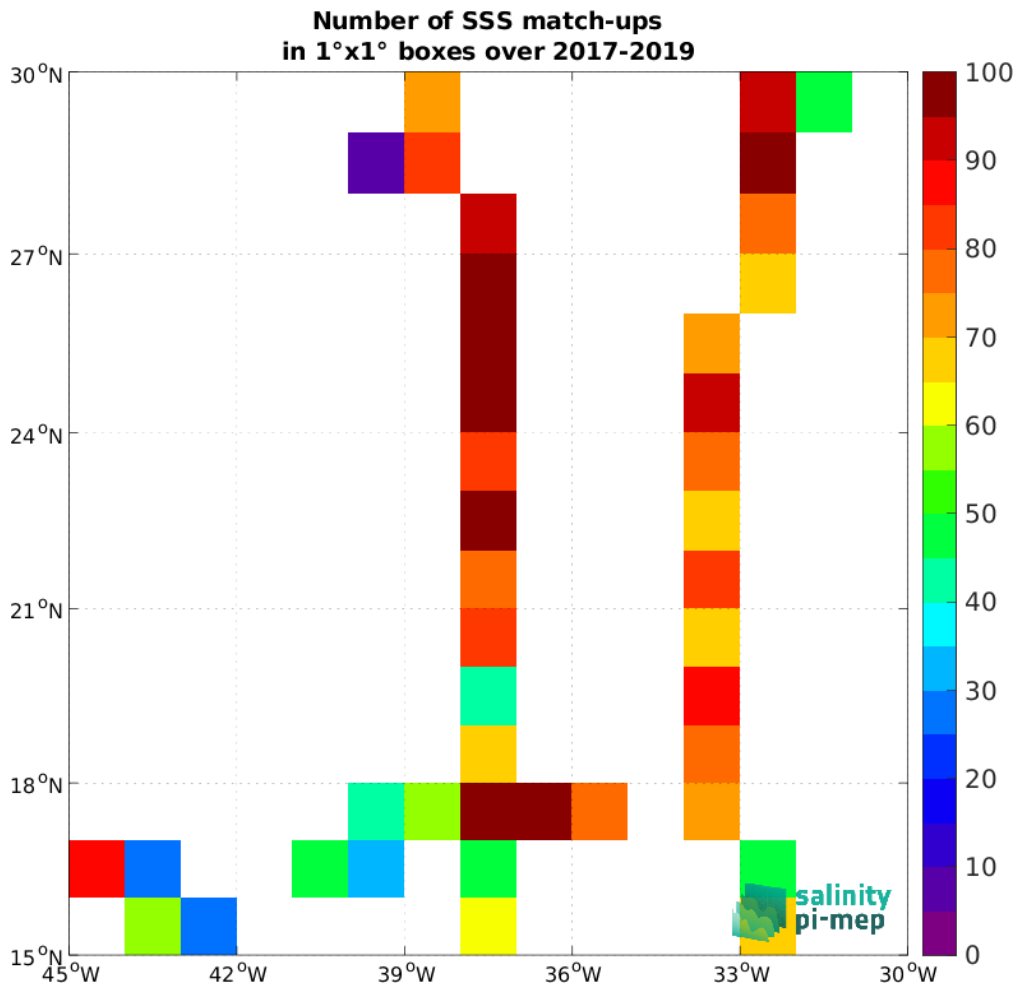
Figure 5: Number of SSS match-ups between TSG (GOSUD-Sailing-ship) SSS and the SMAP SSS L3 v5.0 - Monthly (JPL) SSS product for the SPURS 1 Pi-MEP region over 1°x1° boxes and for the full satellite product period.
