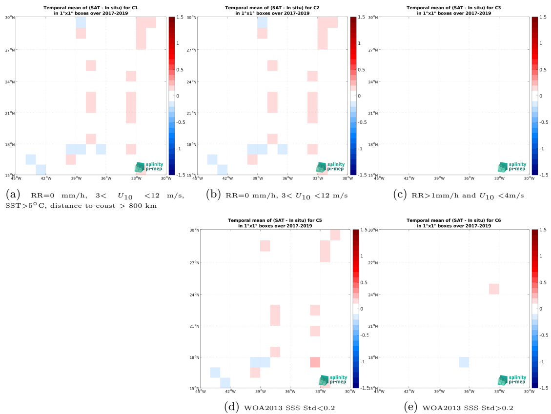
Figure 14: Temporal mean gridded over spatial boxes of size 1^\circ \times 1^\circ of \Delta SSS (SMAP SSS L3 v5.0 - Monthly (JPL) - TSG (GOSUD-Sailing-ship)) for 5 different subdatasets corresponding to:RR=0 mm/h, 3 < U_{10} < 12 m/s, SST >5^\circ C, distance to coast > 800 km (a), RR=0 mm/h, 3 < U_{10} < 12 m/s (b), RR >1 mm/h and U_{10} < 4 m/s (c), WOA2013 SSS Std <0.2 (d), WOA2013 SSS Std >0.2 (e).
