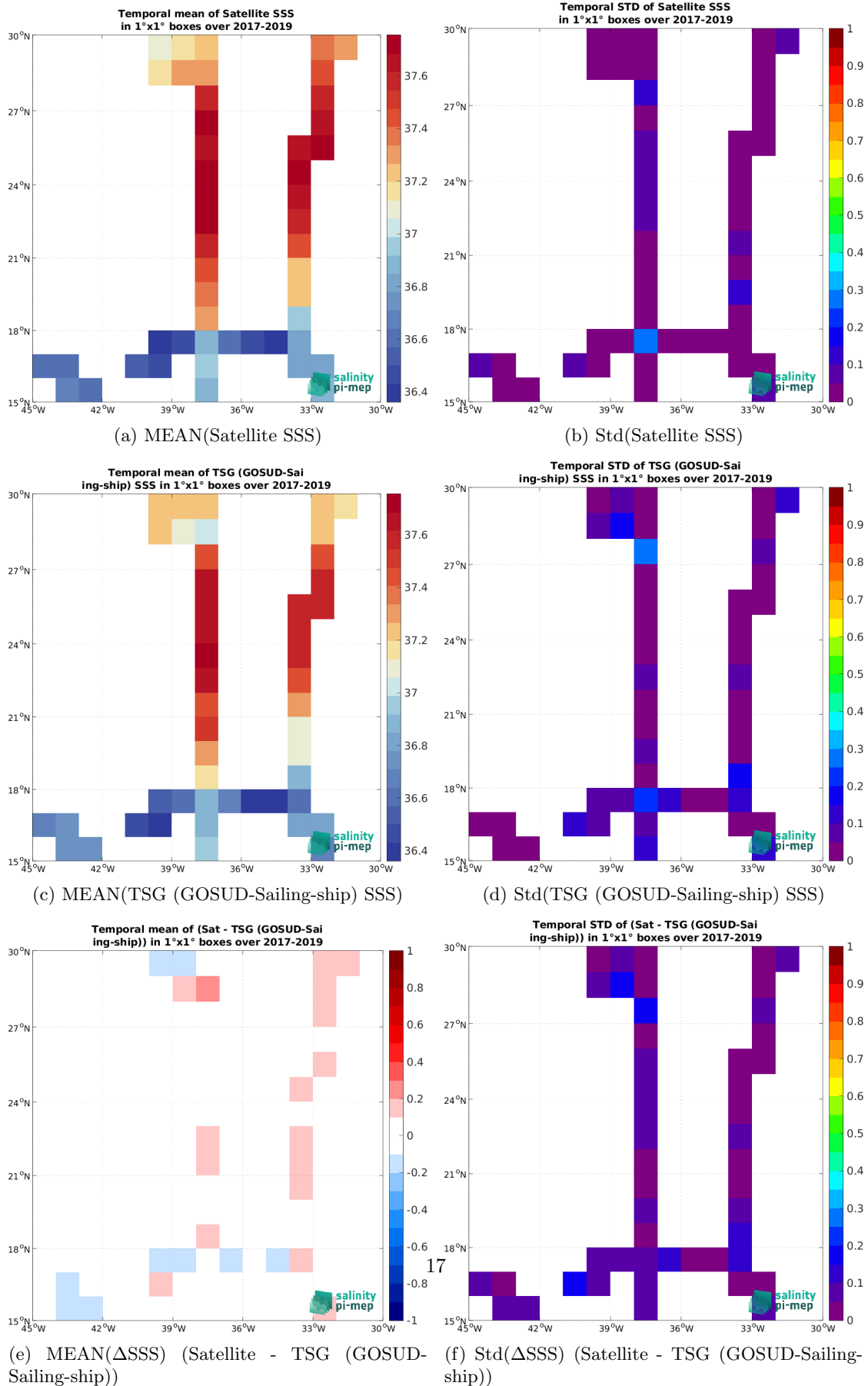
Figure 6: Temporal mean (left) and Std (right) of SSS from SMAP SSS L3 v5.0 - Monthly (JPL) (top), TSG (GOSUD-Sailing-ship) (middle), and of \Delta SSS (Satellite - TSG (GOSUD-Sailing-ship)). Only match-up pairs are used to generate these maps.
