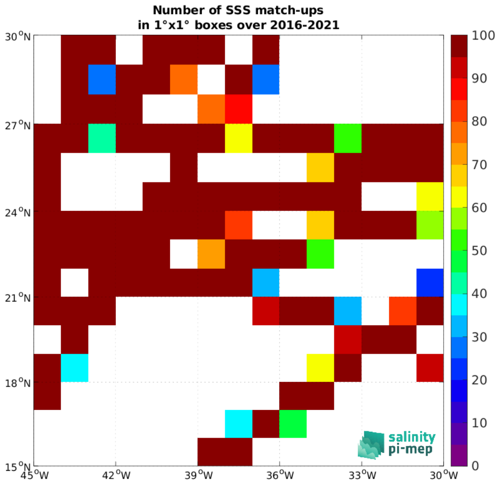
Figure 5: Number of SSS match-ups between TSG (GOSUD-Research-vessel) SSS and the SMAP SSS L3 v5.0 - Monthly (JPL) SSS product for the SPURS 1 Pi-MEP region over 1°x1° boxes and for the full satellite product period.
