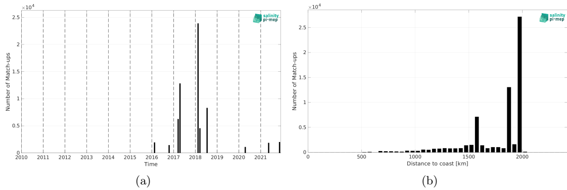
Figure 2: Number of match-ups between TSG (GOSUD-Research-vessel) and SMAP SSS L3 v5.0 - Monthly (JPL) SSS as a function of time (a) and as function of the distance to coast (b) over the SPURS 1 Pi-MEP region and for the full satellite product period.
