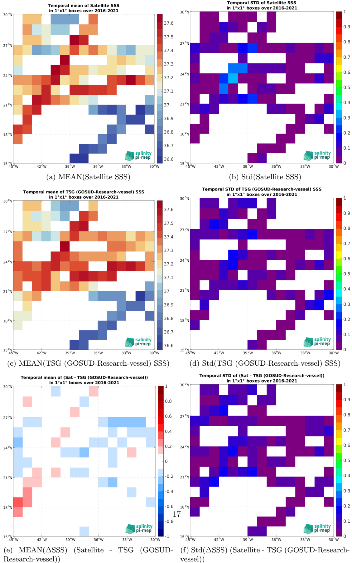
Figure 7: Temporal mean (left) and Std (right) of SSS from SMAP SSS L3 v5.0 - Monthly (JPL) (top), TSG (GOSUD-Research-vessel) (middle), and of \Delta SSS (Satellite - TSG (GOSUD-Research-vessel)). Only match-up pairs are used to generate these maps.
