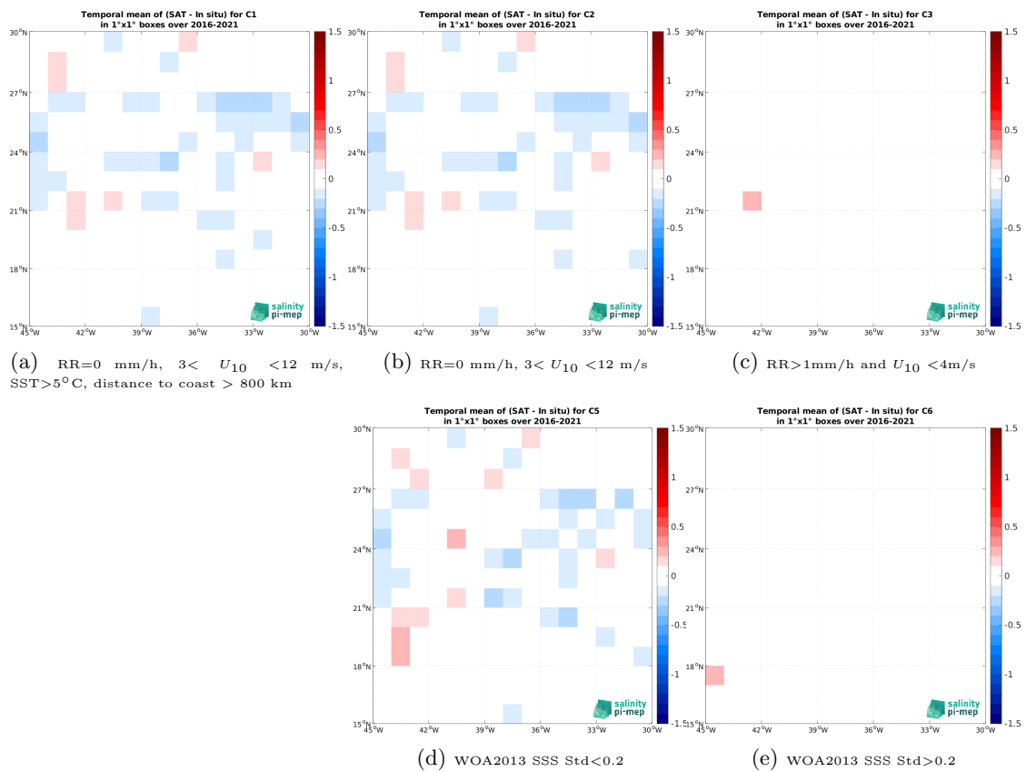
Figure 14: Temporal mean gridded over spatial boxes of size 1^\circ \times 1^\circ of \Delta SSS (SMAP SSS L3 v5.0 - Monthly (JPL) - TSG (GOSUD-Research-vessel)) for 5 different subdatasets corresponding to:RR=0 mm/h, 3 < U_{10} < 12 m/s, SST>5°C, distance to coast > 800 km (a), RR=0 mm/h, 3 < U_{10} < 12 m/s (b), RR>1mm/h and U_{10} < 4 m/s (c), WOA2013 SSS Std<0.2 (d), WOA2013 SSS Std>0.2 (e).
