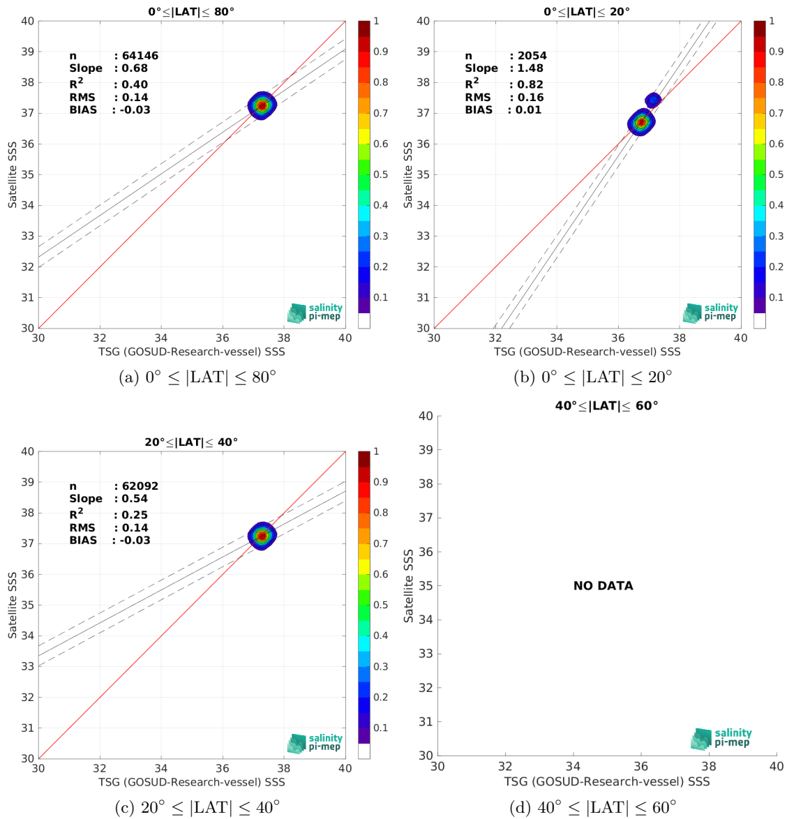
Figure 10: Contour maps of the concentration of SMAP SSS L3 v5.0 - Monthly (JPL) SSS (y-axis) versus TSG (GOSUD-Research-vessel) SSS (x-axis) at match-up pairs for different latitude bands. For each plot, the red line shows x=y . The black thin and dashed lines indicate a linear fit through the data cloud and the \pm 95\% confidence levels, respectively. The number match-up pairs n , the slope and R^2 coefficient of the linear fit, the root mean square (RMS) and the mean bias between satellite and in situ data are indicated for each latitude band in each plots.
