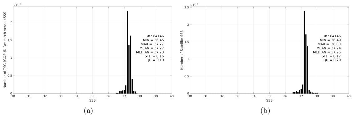
Figure 3: Histograms of SSS from TSG (GOSUD-Research-vessel) (a) and SMAP SSS L3 v5.0 - Monthly (JPL) (b) considering all match-up pairs per bins of 0.1 over the SPURS 1 Pi-MEP region and for the full satellite product period.
