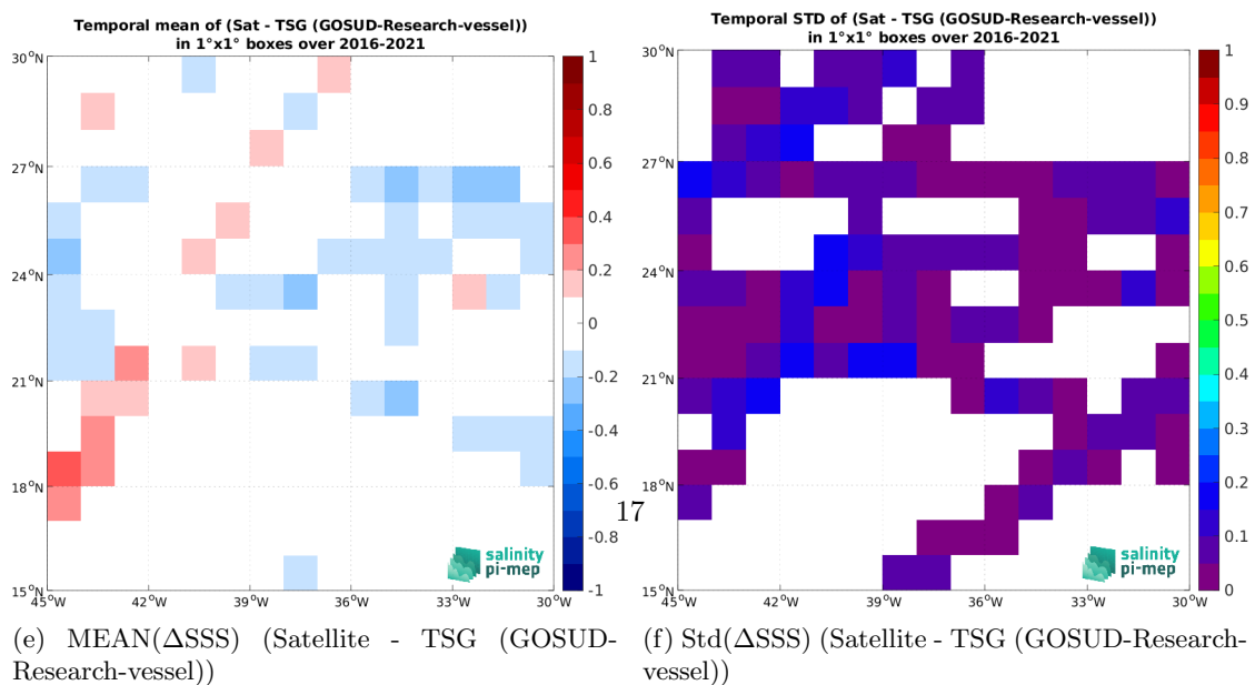
Figure 6: Temporal mean (left) and Std (right) of SSS from SMAP SSS L3 v5.0 - Monthly (JPL) (top), TSG (GOSUD-Research-vessel) (middle), and of \Delta SSS (Satellite - TSG (GOSUD-Research-vessel)). Only match-up pairs are used to generate these maps.
