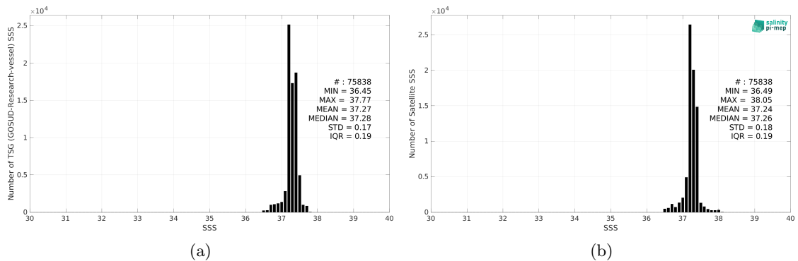
Figure 2: Histograms of SSS from TSG (GOSUD-Research-vessel) (a) and SMAP SSS L3 v5.0 - Monthly (JPL) (b) considering all match-up pairs per bins of 0.1 over the SPURS 1 Pi-MEP region and for the full satellite product period.
