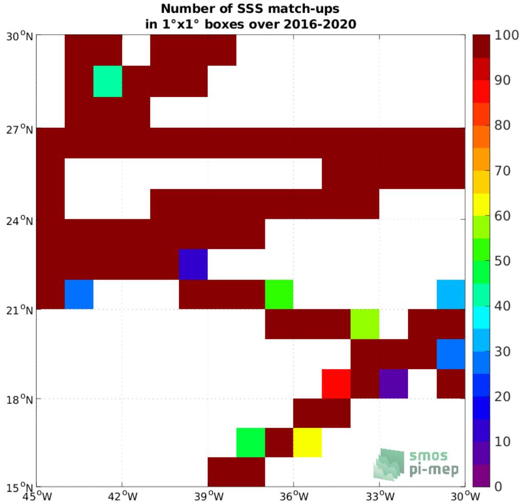
Figure 4: Number of SSS match-ups between TSG (GOSUD-Research-vessel) SSS and the SMAP SSS L3 v5.0 - Monthly (JPL) SSS product for the SPURS 1 Pi-MEP region over 1^\circ \times 1^\circ boxes and for the full satellite product period.
