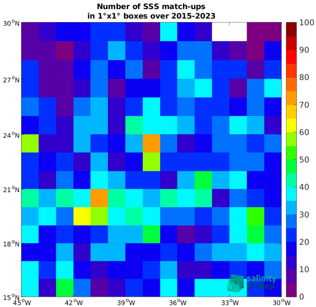
Figure 5: Number of SSS match-ups between Argo SSS and the SMAP SSS L3 v5.0 - Monthly (JPL) SSS product for the SPURS 1 Pi-MEP region over 1°x1° boxes and for the full satellite product period.
