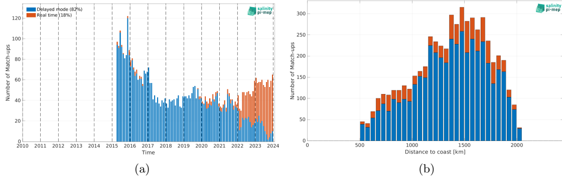
Figure 2: Number of match-ups between Argo and SMAP SSS L3 v5.0 - Monthly (JPL) SSS as a function of time (a) and as function of the distance to coast (b) over the SPURS 1 Pi-MEP region and for the full satellite product period.
