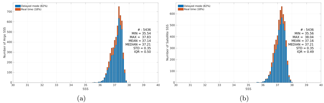
Figure 3: Histograms of SSS from Argo (a) and SMAP SSS L3 v5.0 - Monthly (JPL) (b) considering all match-up pairs per bins of 0.1 over the SPURS 1 Pi-MEP region and for the full satellite product period.
