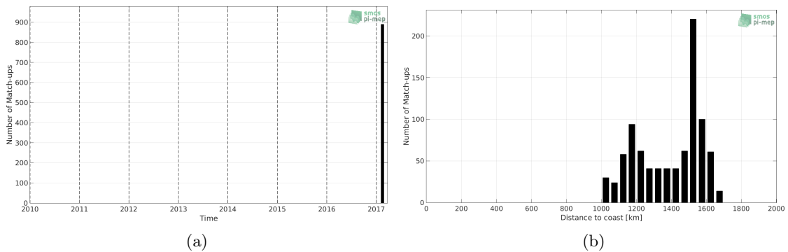
Figure 1: Number of match-ups between TSG-GOSUD-Sailing-ship and SMAP-L3-JPL-V4.3-MONTHLY-60KM SSS as a function of time (a) and as function of the distance to coast (b) over the SPURS 1 Pi-MEP region and for the full satellite product period.
