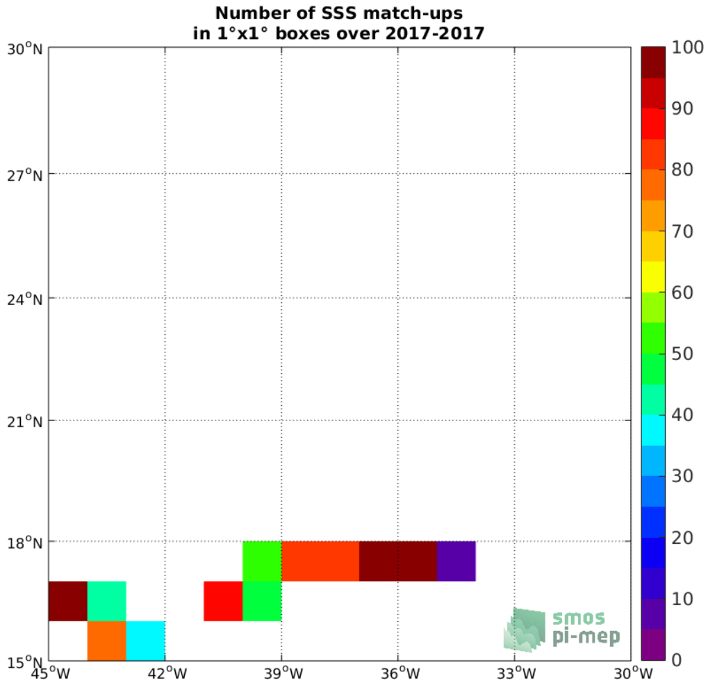
Figure 4: Number of SSS match-ups between TSG-GOSUD-Sailing-ship SSS and the SMAP-L3-JPL-V4.3-MONTHLY-60KM SSS product for the SPURS 1 Pi-MEP region over 1°x1° boxes and for the full satellite product period.
