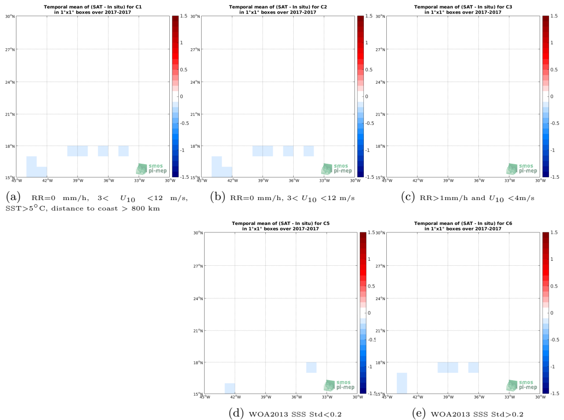
Figure 12: Temporal mean gridded over spatial boxes of size 1^\circ \times 1^\circ of \Delta SSS (SMAP-L3-JPL-V4.3-MONTHLY-60KM - TSG-GOSUD-Sailing-ship) for 5 different subdatasets corresponding to: RR=0 mm/h, 3 < U_{10} < 12 m/s, SST > 5^\circ C , distance to coast > 800 km (a), RR=0 mm/h, 3 < U_{10} < 12 m/s (b), RR > 1 mm/h and U_{10} < 4 m/s (c), WOA2013 SSS Std < 0.2 (d), WOA2013 SSS Std > 0.2 (e).
