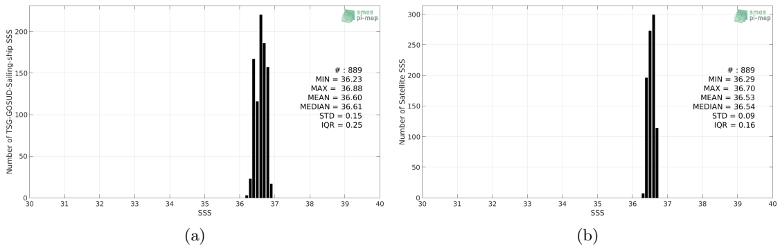
Figure 2: Histograms of SSS from TSG-GOSUD-Sailing-ship (a) and SMAP-L3-JPL-V4.3-MONTHLY-60KM (b) considering all match-up pairs per bins of 0.1 over the SPURS 1 Pi-MEP region and for the full satellite product period.
