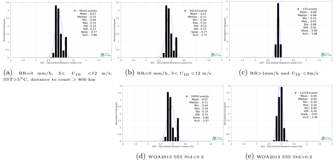
Figure 13: Normalized histogram of \Delta SSS (SMAP-L3-JPL-V4.3-MONTHLY-60KM - TSG-GOSUD-Research-vessel) for 5 different subdatasets corresponding to: RR=0 mm/h, 3 < U_{10} < 12 m/s, SST>5°C, distance to coast > 800 km (a), RR=0 mm/h, 3 < U_{10} < 12 m/s (b), RR>1mm/h and U_{10} < 4 m/s (c), WOA2013 SSS Std<0.2 (d), WOA2013 SSS Std>0.2 (e).
