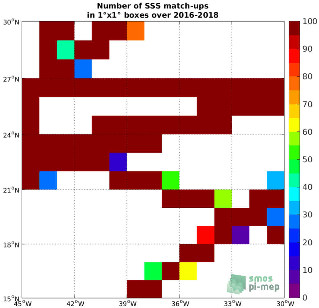
Figure 4: Number of SSS match-ups between TSG-GOSUD-Research-vessel SSS and the SMAP-L3-JPL-V4.3-MONTHLY-60KM SSS product for the SPURS 1 Pi-MEP region over 1°x1° boxes and for the full satellite product period.
