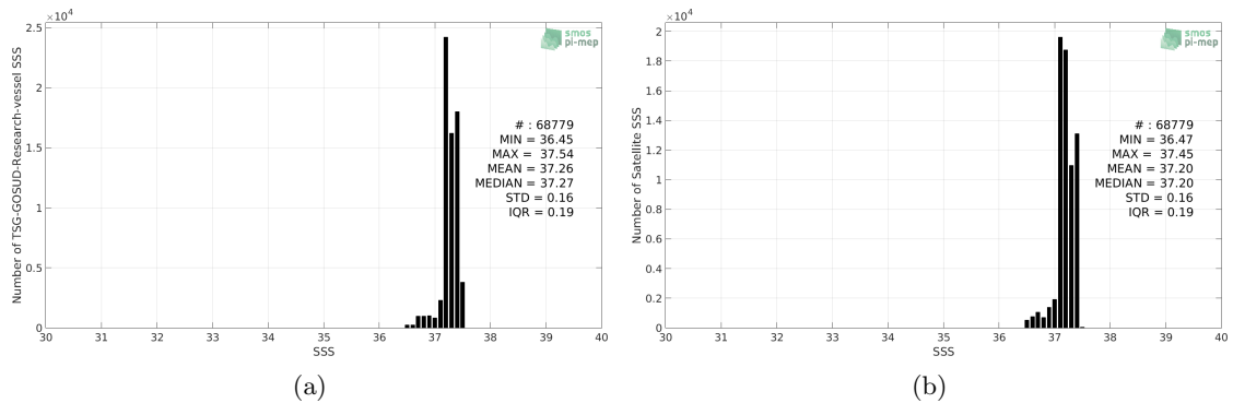
Figure 2: Histograms of SSS from TSG-GOSUD-Research-vessel (a) and SMAP-L3-JPL-V4.3-MONTHLY-60KM (b) considering all match-up pairs per bins of 0.1 over the SPURS 1 Pi-MEP region and for the full satellite product period.
