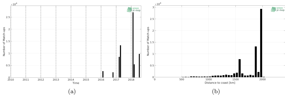
Figure 1: Number of match-ups between TSG-GOSUD-Research-vessel and SMAP-L3-JPL-V4.3-MONTHLY-60KM SSS as a function of time (a) and as function of the distance to coast (b) over the SPURS 1 Pi-MEP region and for the full satellite product period.
