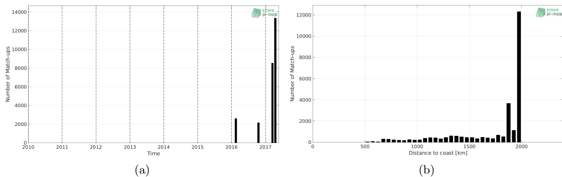
Figure 1: Number of match-ups between TSG-GOSUD-Research-vessel and SMAP-L3-JPL-V4.2-8DAY-RUNNING-60KM SSS as a function of time (a) and as function of the distance to coast (b) over the SPURS 1 Pi-MEP region and for the full satellite product period.
