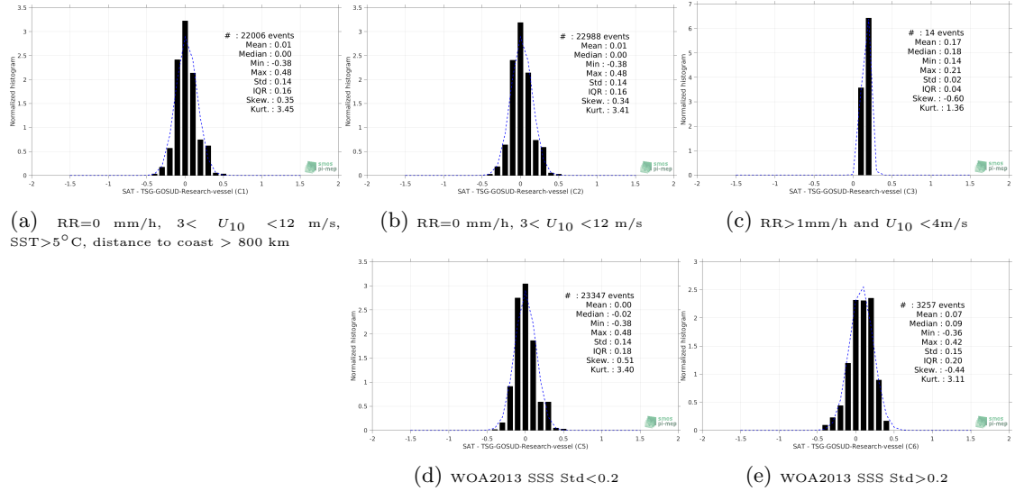
Figure 13: Normalized histogram of \Delta\text{SSS} (SMAP-L3-JPL-V4.2-8DAY-RUNNING-60KM - TSG-GOSUD-Research-vessel) for 5 different subdatasets corresponding to: RR=0 mm/h, 3 < U_{10} < 12 m/s, SST > 5^{\circ}\text{C} , distance to coast > 800 km (a), RR=0 mm/h, 3 < U_{10} < 12 m/s (b), RR > 1\text{mm/h} and U_{10} < 4\text{m/s} (c), WOA2013 SSS Std < 0.2 (d), WOA2013 SSS Std > 0.2 (e).
