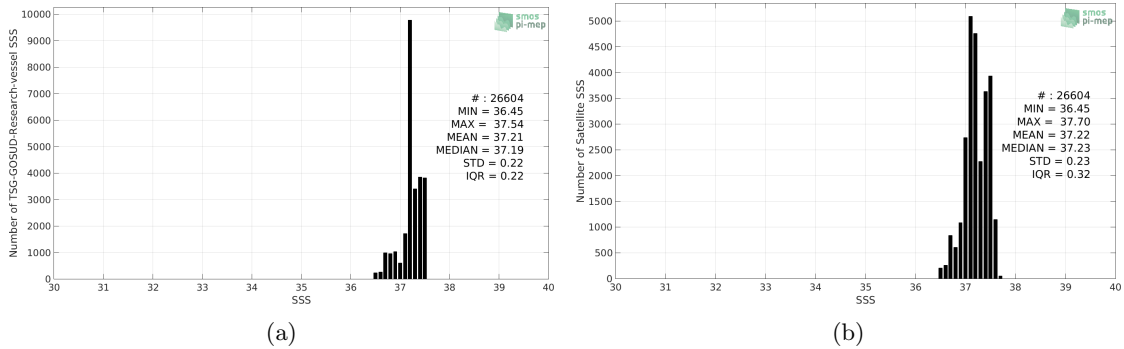
Figure 2: Histograms of SSS from TSG-GOSUD-Research-vessel (a) and SMAP-L3-JPL-V4.2-8DAY-RUNNING-60KM (b) considering all match-up pairs per bins of 0.1 over the SPURS 1 Pi-MEP region and for the full satellite product period.
