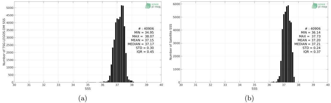
Figure 2: Histograms of SSS from TSG-LEGOS-DM (a) and SMAP-L3-JPL-V4.2-MONTHLY-60KM (b) considering all match-up pairs per bins of 0.1 over the SPURS 1 Pi-MEP region and for the full satellite product period.
