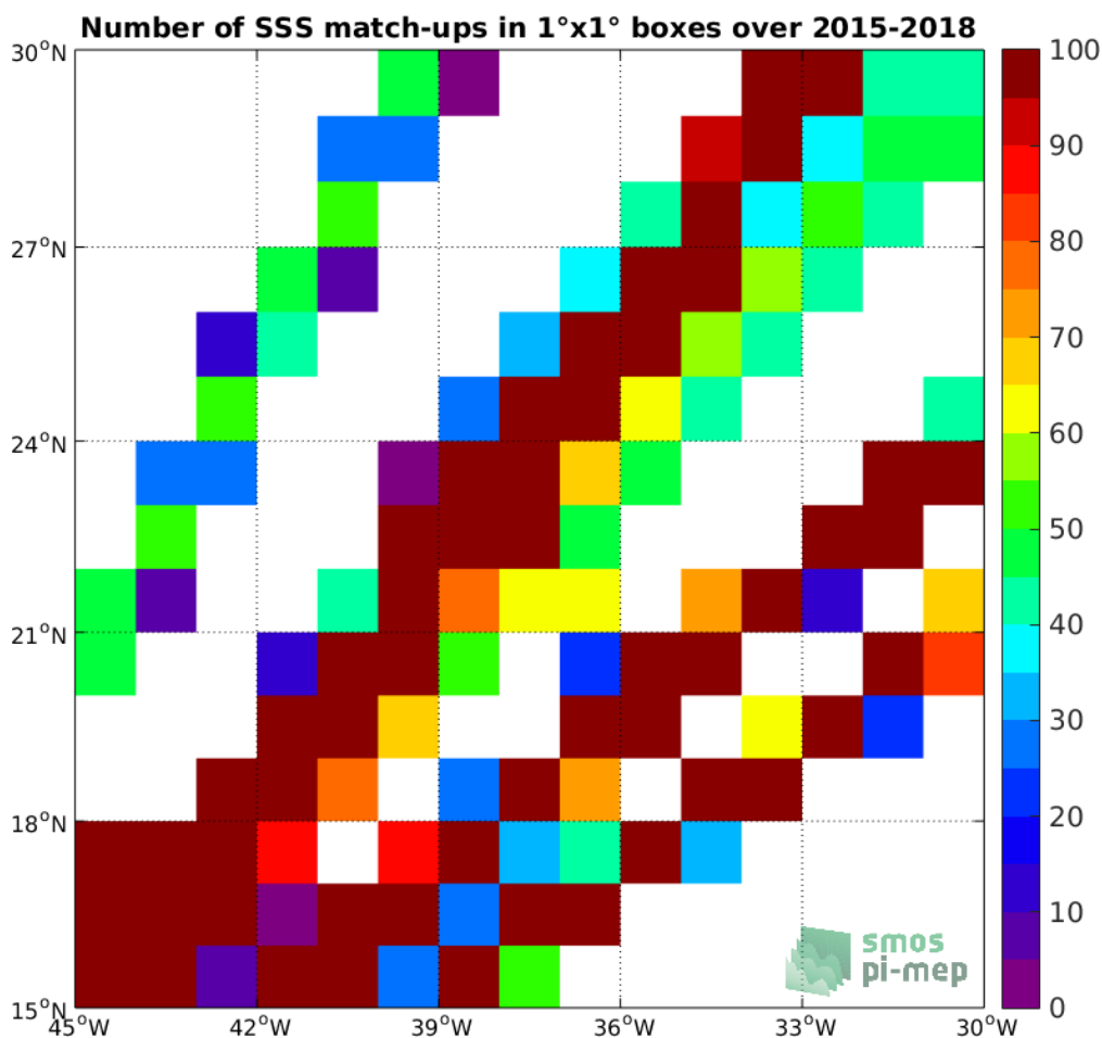
Figure 4: Number of SSS match-ups between TSG-LEGOS-DM SSS and the SMAP-L3-JPL-V4.2-MONTHLY-60KM SSS product for the SPURS 1 Pi-MEP region over 1°x1° boxes and for the full satellite product period.
