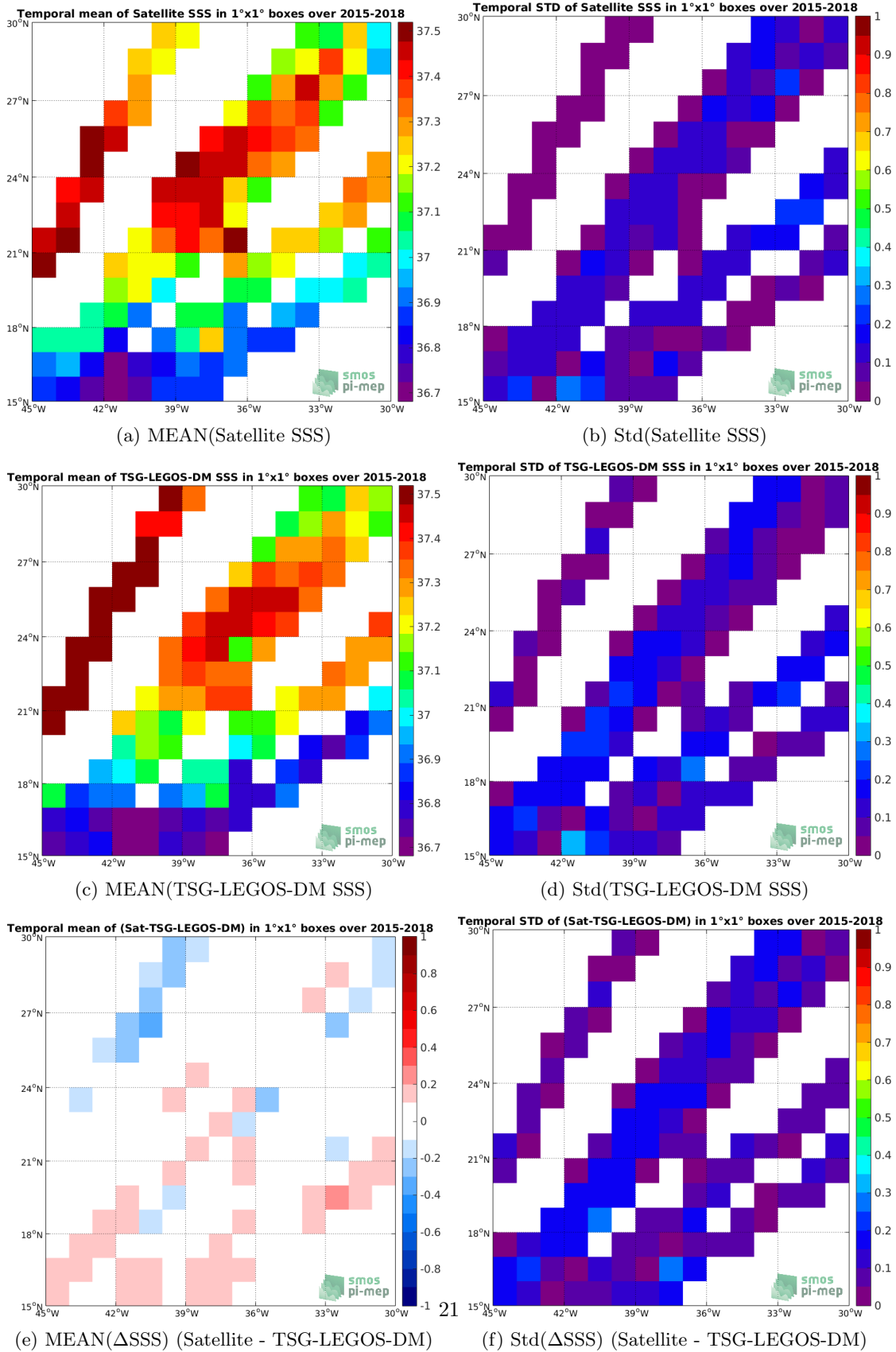
Figure 6: Temporal mean (left) and Std (right) of SSS from SMAP-L3-JPL-V4.2-MONTHLY-60KM (top), TSG-LEGOS-DM (middle), and of \Delta SSS (Satellite - TSG-LEGOS-DM). Only match-up pairs are used to generate these maps.
