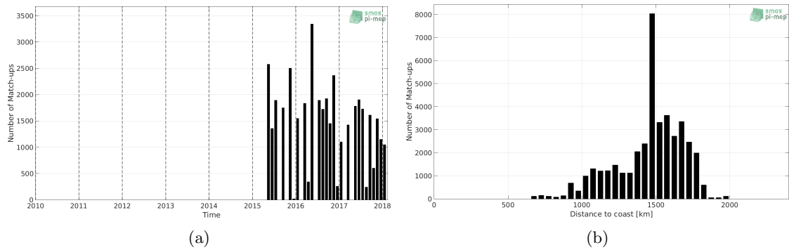
Figure 1: Number of match-ups between TSG-LEGOS-DM and SMAP-L3-JPL-V4.2-MONTHLY-60KM SSS as a function of time (a) and as function of the distance to coast (b) over the SPURS 1 Pi-MEP region and for the full satellite product period.
