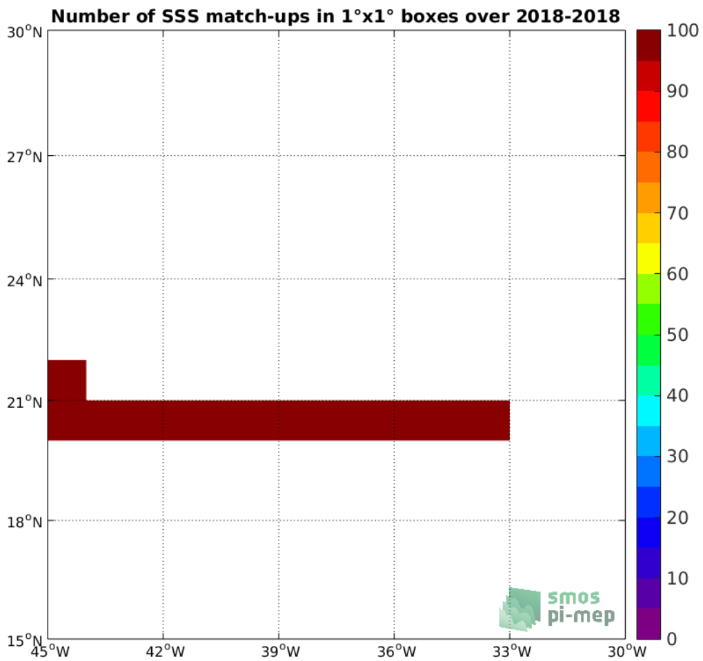
Figure 4: Number of SSS match-ups between TSG-SAMOS SSS and the SMAP-L3-JPL-V4-8DAY-RUNNING-60KM SSS product for the SPURS 1 Pi-MEP region over 1°x1° boxes and for the full satellite product period.
