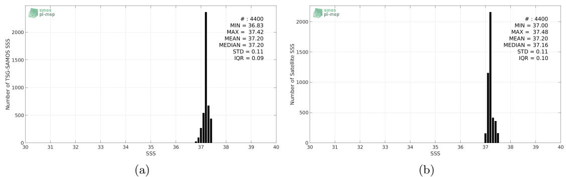
Figure 2: Histograms of SSS from TSG-SAMOS (a) and SMAP-L3-JPL-V4-8DAY-RUNNING-60KM (b) considering all match-up pairs per bins of 0.1 over the SPURS 1 Pi-MEP region and for the full satellite product period.
