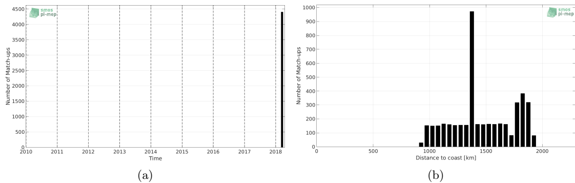
Figure 1: Number of match-ups between TSG-SAMOS and SMAP-L3-JPL-V4-8DAY-RUNNING-60KM SSS as a function of time (a) and as function of the distance to coast (b) over the SPURS 1 Pi-MEP region and for the full satellite product period.
