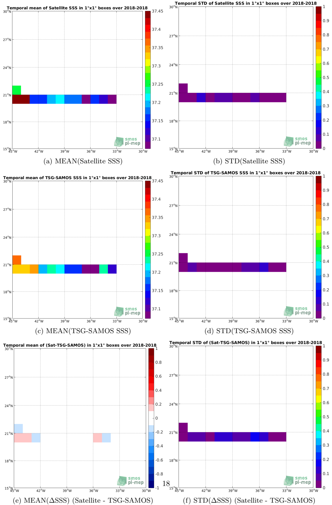
Figure 6: Temporal mean (left) and STD (right) of SSS from SMAP-L3-JPL-V4-8DAY-RUNNING-60KM (top), TSG-SAMOS (middle), and of \Delta SSS (Satellite - TSG-SAMOS). Only match-up pairs are used to generate these maps.
