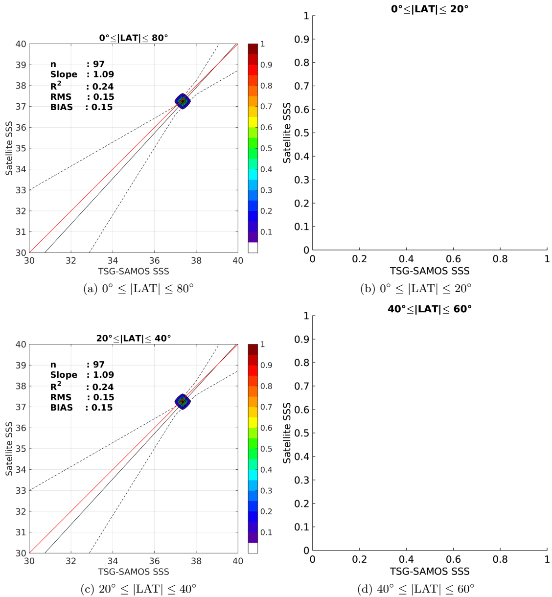
Figure 9: Contour maps of the concentration of SMAP-L3-JPL-V4-8DAY-RUNNING-60KM SSS (y-axis) versus TSG-SAMOS SSS (x-axis) at match-up pairs for different latitude bands. For each plot, the red line shows x=y . The black thin and dashed lines indicate a linear fit through the data cloud and the \pm 95\% confidence levels, respectively. The number match-up pairs n , the slope and R^2 coefficient of the linear fit, the root mean square (RMS) and the mean bias between satellite and in situ data are indicated for each latitude band in each plots.
