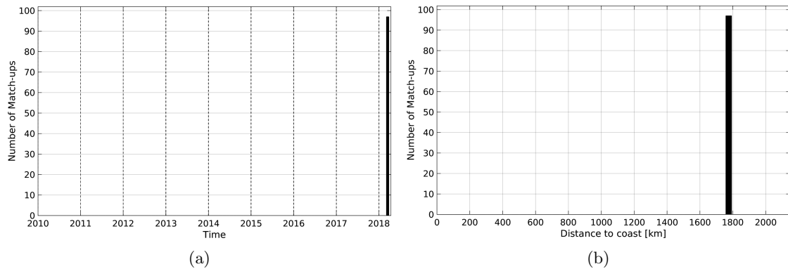
Figure 1: Number of match-ups between TSG-SAMOS and SMAP-L3-JPL-V4-8DAY-RUNNING-60KM SSS as a function of time (a) and as function of the distance to coast (b) over the SPURS 1 Pi-MEP region and for the full satellite product period.
