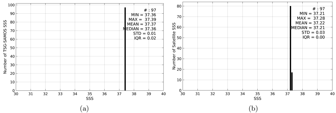
Figure 2: Histograms of SSS from TSG-SAMOS (a) and SMAP-L3-JPL-V4-8DAY-RUNNING-60KM (b) considering all match-up pairs per bins of 0.1 over the SPURS 1 Pi-MEP region and for the full satellite product period.
