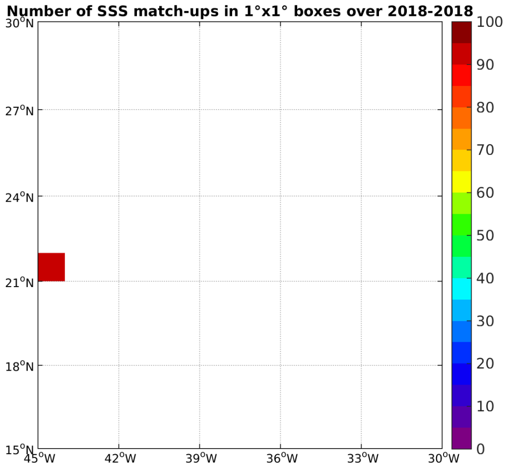
Figure 4: Number of SSS match-ups between TSG-SAMOS SSS and the SMAP-L3-JPL-V4-8DAY-RUNNING-60KM SSS product for the SPURS 1 Pi-MEP region over 1°x1° boxes and for the full satellite product period.
