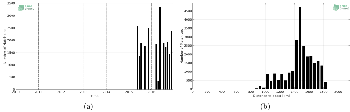
Figure 1: Number of match-ups between TSG-LEGOS-DM and SMAP-L3-JPL-V4-8DAY-RUNNING-60KM SSS as a function of time (a) and as function of the distance to coast (b) over the SPURS 1 Pi-MEP region and for the full satellite product period.
