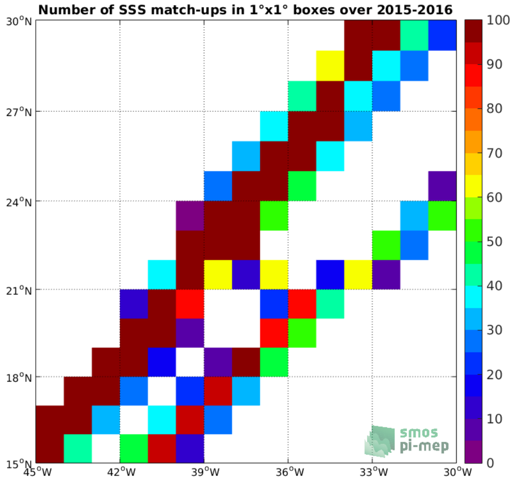
Figure 4: Number of SSS match-ups between TSG-LEGOS-DM SSS and the SMAP-L3-JPL-V4-8DAY-RUNNING-60KM SSS product for the SPURS 1 Pi-MEP region over 1°x1° boxes and for the full satellite product period.
