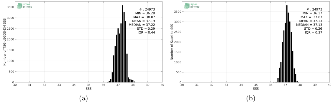
Figure 2: Histograms of SSS from TSG-LEGOS-DM (a) and SMAP-L3-JPL-V4-8DAY-RUNNING-60KM (b) considering all match-up pairs per bins of 0.1 over the SPURS 1 Pi-MEP region and for the full satellite product period.
