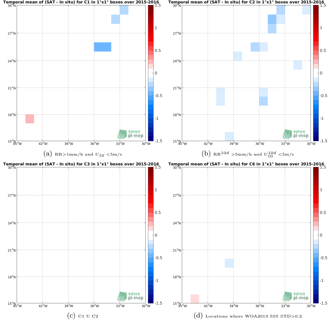
Figure 12: Temporal mean gridded over spatial boxes of size 1^\circ \times 1^\circ of \Delta SSS (SMAP-L3-JPL-V4-8DAY-RUNNING-60KM - TSG-LEGOS-DM) for 4 different subdatasets corresponding to: RR > 1\text{mm/h} and U_{10} < 5\text{m/s} (a), RR^{10d} > 5\text{mm/h} and U_{10}^{10d} < 5\text{m/s} (b), C1 U C2 (c), Locations where WOA2013 SSS STD > 0.2 (d).
