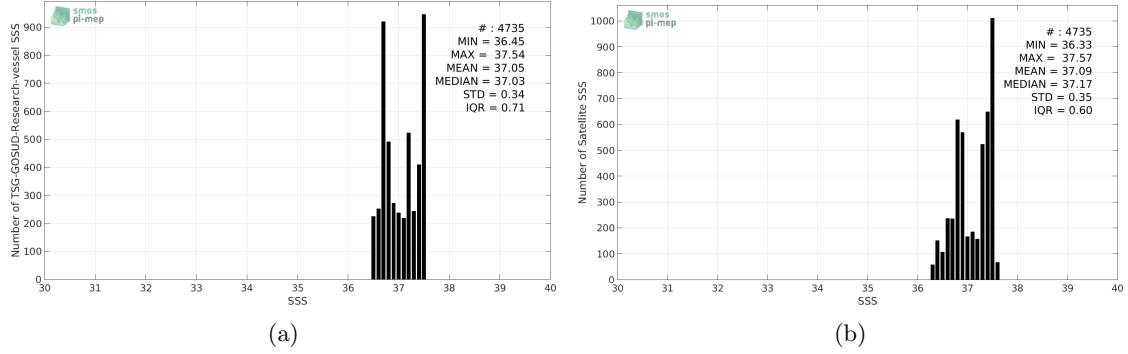
Figure 2: Histograms of SSS from TSG-GOSUD-Research-vessel (a) and SMAP-L3-JPL-V4-8DAY-RUNNING-60KM (b) considering all match-up pairs per bins of 0.1 over the SPURS 1 Pi-MEP region and for the full satellite product period.
