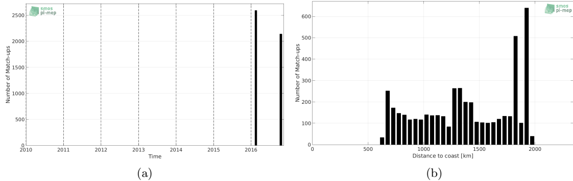
Figure 1: Number of match-ups between TSG-GOSUD-Research-vessel and SMAP-L3-JPL-V4-8DAY-RUNNING-60KM SSS as a function of time (a) and as function of the distance to coast (b) over the SPURS 1 Pi-MEP region and for the full satellite product period.
