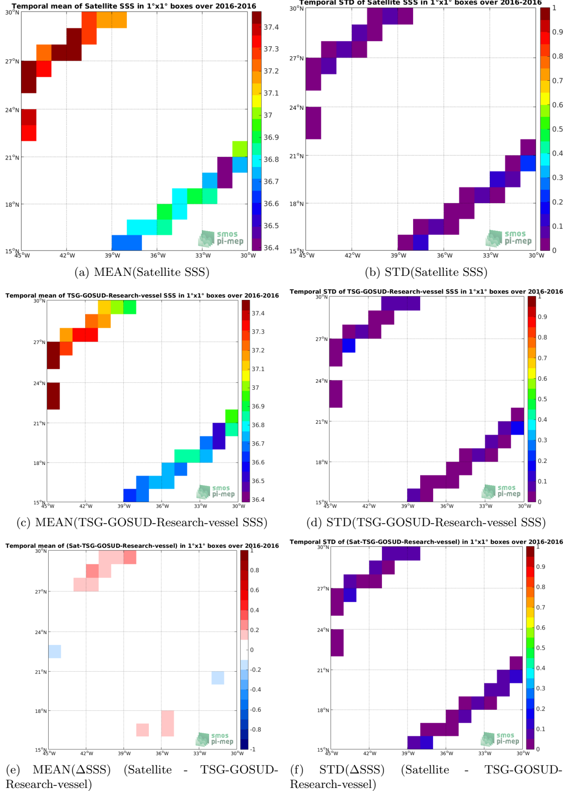
Figure 6: Temporal mean (left) and STD (right) of SSS from SMAP-L3-JPL-V4-8DAY-RUNNING-60KM (top), TSG-GOSUD-Research-vessel (middle), and of \Delta SSS (Satellite - TSG-GOSUD-Research-vessel). Only match-up pairs are used to generate these maps.
