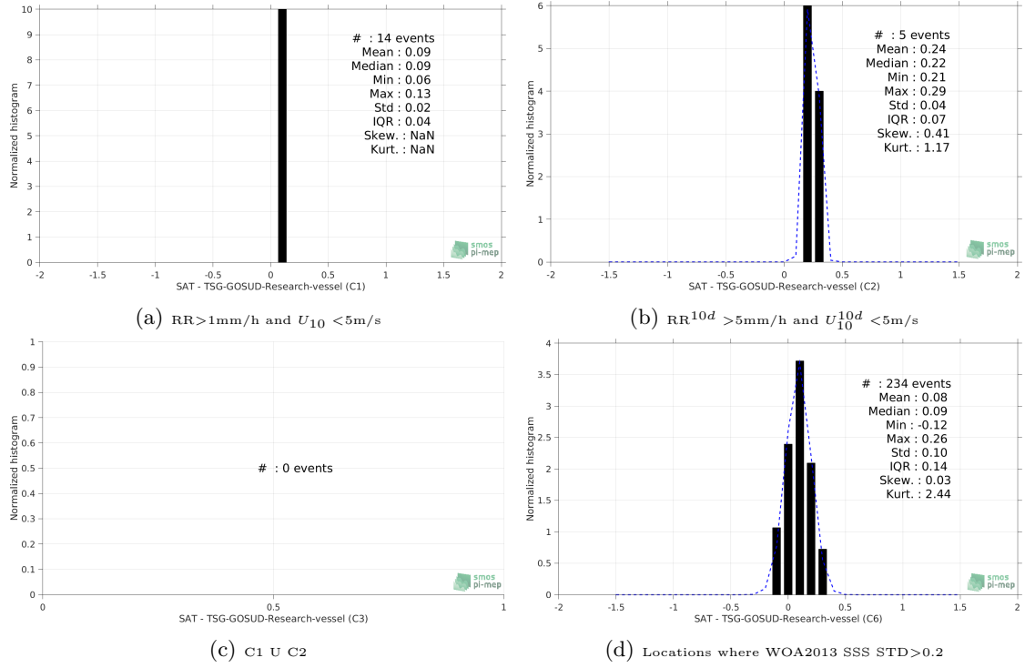
Figure 13: Normalized histogram of \Delta\text{SSS} (SMAP-L3-JPL-V4-8DAY-RUNNING-60KM - TSG-GOSUD-Research-vessel) for 6 different subdatasets corresponding to: RR>1mm/h and U_{10} < 5\text{m/s} (a), RR^{10d} > 5\text{mm/h} and U_{10}^{10d} < 5\text{m/s} (b), C1 U C2 (c), Locations where WOA2013 SSS STD>0.2 (d).
