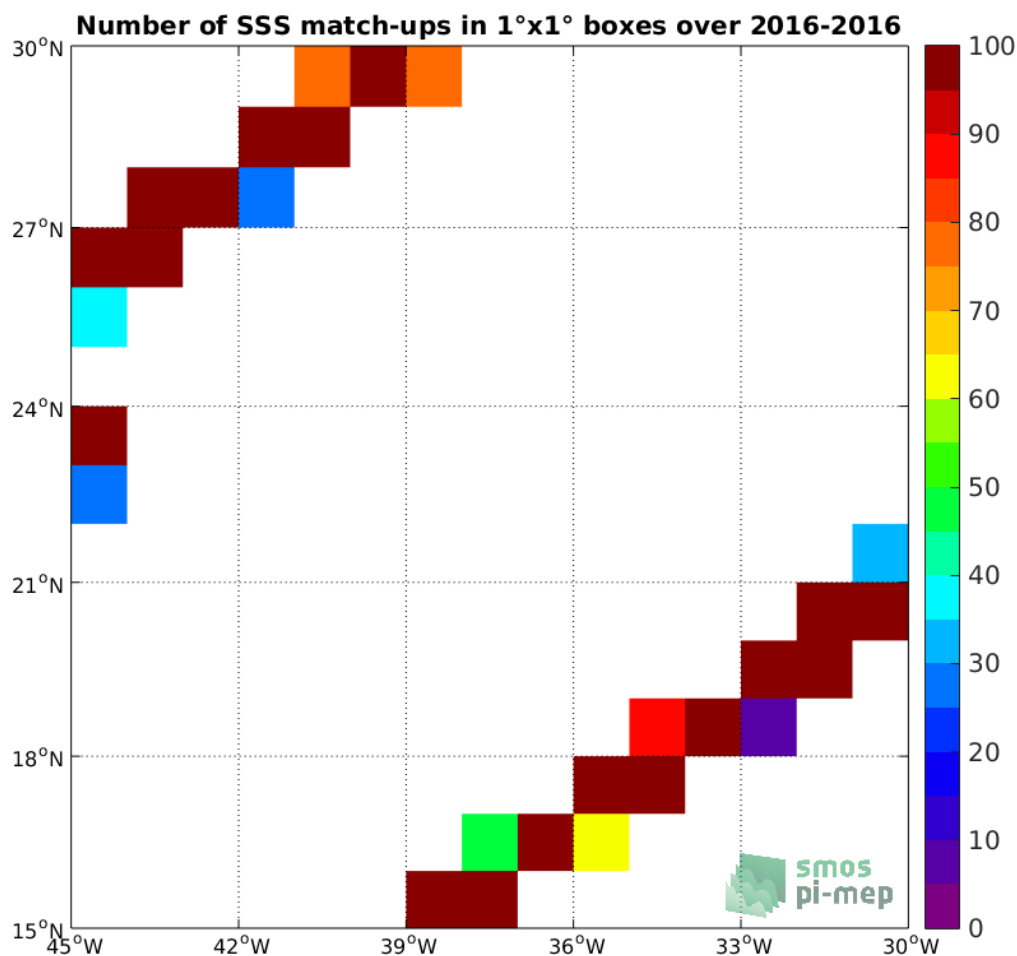
Figure 4: Number of SSS match-ups between TSG-GOSUD-Research-vessel SSS and the SMAP-L3-JPL-V4-8DAY-RUNNING-60KM SSS product for the SPURS 1 Pi-MEP region over 1°x1° boxes and for the full satellite product period.
