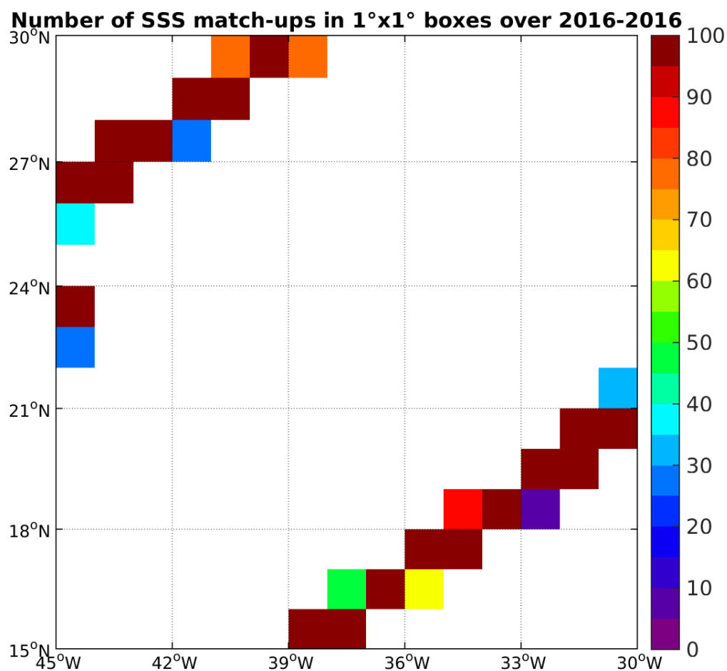
Figure 4: Number of SSS match-ups between TSG-GOSUD-Research-vessel SSS and the SMAP-L3-JPL-V4-8DAY-RUNNING-60KM SSS product for the SPURS 1 Pi-MEP region over 1°x1° boxes and for the full satellite product period.
