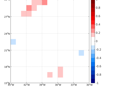
(e) MEAN( \Delta SSS) (Satellite - TSG-GOSUD-Research-vessel)
