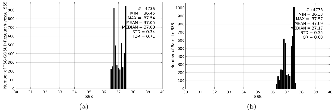
Figure 2: Histograms of SSS from TSG-GOSUD-Research-vessel (a) and SMAP-L3-JPL-V4-8DAY-RUNNING-60KM (b) considering all match-up pairs per bins of 0.1 over the SPURS 1 Pi-MEP region and for the full satellite product period.
