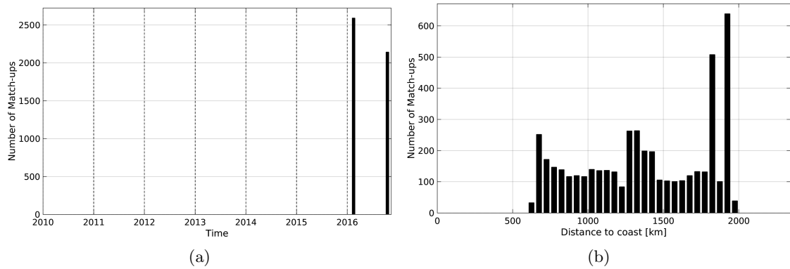
Figure 1: Number of match-ups between TSG-GOSUD-Research-vessel and SMAP-L3-JPL-V4-8DAY-RUNNING-60KM SSS as a function of time (a) and as function of the distance to coast (b) over the SPURS 1 Pi-MEP region and for the full satellite product period.
