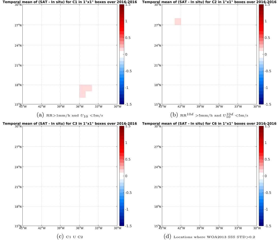
Figure 12: Temporal mean gridded over spatial boxes of size 1^\circ \times 1^\circ of \Delta SSS (SMAP-L3-JPL-V4-8DAY-RUNNING-60KM - TSG-GOSUD-Research-vessel) for 4 different subdatasets corresponding to: RR > 1 mm/h and U_{10} < 5 m/s (a), RR^{10d} > 5 mm/h and U_{10}^{10d} < 5 m/s (b), C1 U C2 (c), Locations where WOA2013 SSS STD > 0.2 (d).
