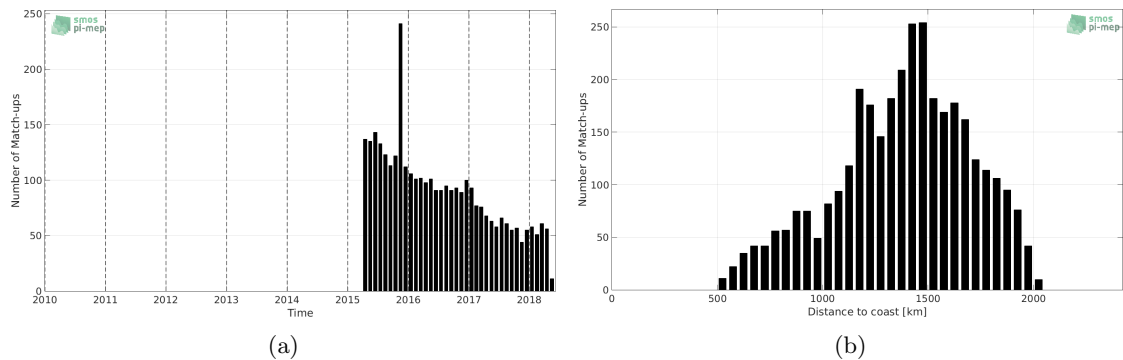
Figure 1: Number of match-ups between Argo and SMAP-L3-JPL-V4-8DAY-RUNNING-60KM SSS as a function of time (a) and as function of the distance to coast (b) over the SPURS 1 Pi-MEP region and for the full satellite product period.
