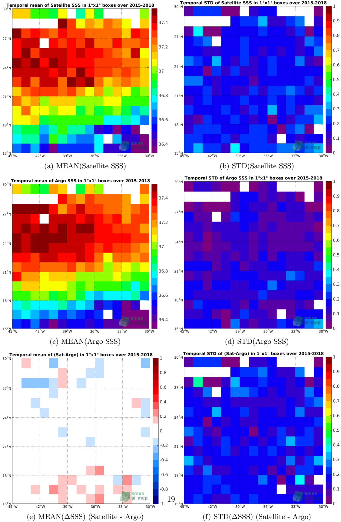
Figure 6: Temporal mean (left) and STD (right) of SSS from SMAP-L3-JPL-V4-8DAY-RUNNING-60KM (top), Argo (middle), and of \Delta SSS (Satellite - Argo). Only match-up pairs are used to generate these maps.
