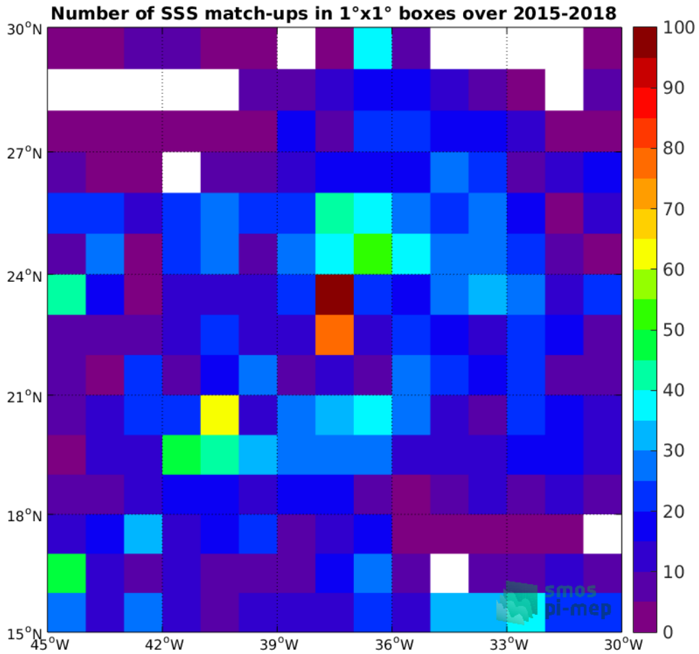
Figure 4: Number of SSS match-ups between Argo SSS and the SMAP-L3-JPL-V4-8DAY-RUNNING-60KM SSS product for the SPURS 1 Pi-MEP region over 1°x1° boxes and for the full satellite product period.
