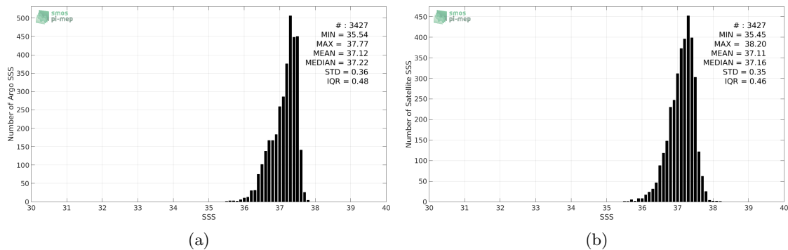
Figure 2: Histograms of SSS from Argo (a) and SMAP-L3-JPL-V4-8DAY-RUNNING-60KM (b) considering all match-up pairs per bins of 0.1 over the SPURS 1 Pi-MEP region and for the full satellite product period.
