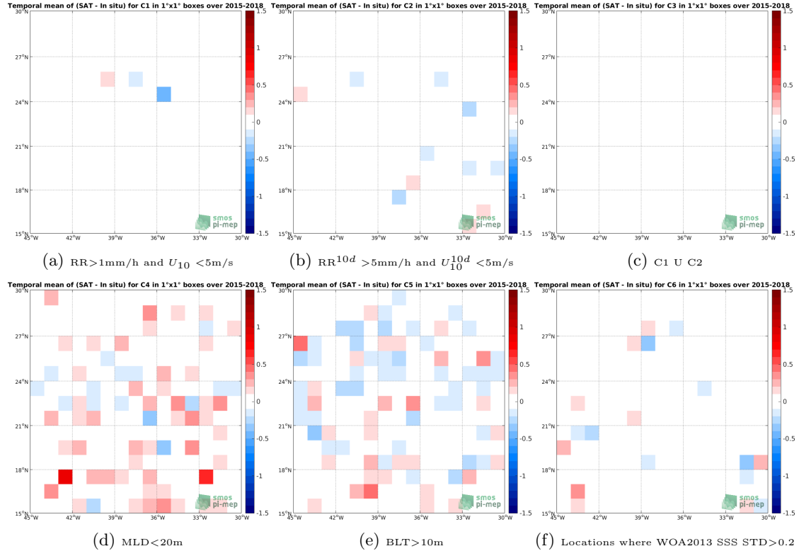
Figure 12: Temporal mean gridded over spatial boxes of size 1^\circ \times 1^\circ of \Delta\text{SSS} (SMAP-L3-JPL-V4-8DAY-RUNNING-60KM - Argo) for 6 different subdatasets corresponding to: \text{RR} > 1\text{mm/h} and U_{10} < 5\text{m/s} (a), \text{RR}^{10d} > 5\text{mm/h} and U_{10}^{10d} < 5\text{m/s} (b), C1 U C2 (c), \text{MLD} < 20\text{m} (d), \text{BLT} > 10\text{m} (e), Locations where WOA2013 SSS STD > 0.2 (f).
