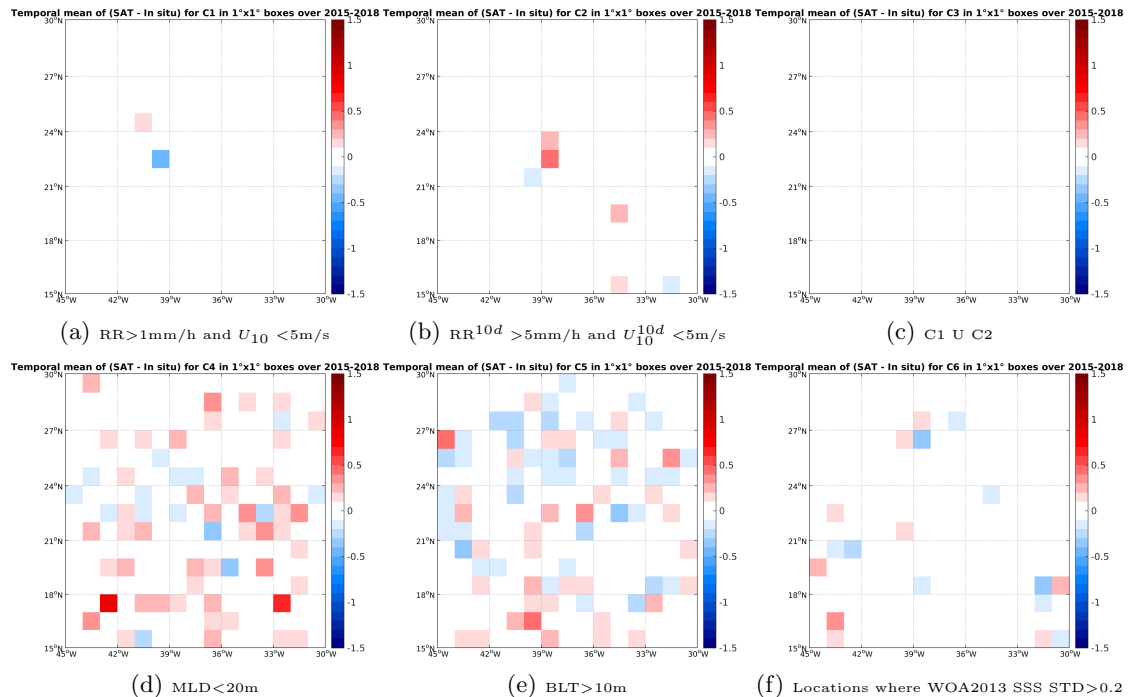
Figure 12: Temporal mean gridded over spatial boxes of size 1^\circ \times 1^\circ of \Delta SSS (SMAP-L3-JPL-V4-8DAY-RUNNING-60KM - Argo) for 6 different subdatasets corresponding to: RR > 1\text{mm/h} and U_{10} < 5\text{m/s} (a), RR^{10d} > 5\text{mm/h} and U_{10}^{10d} < 5\text{m/s} (b), C1 U C2 (c), MLD < 20\text{m} (d), BLT > 10\text{m} (e), Locations where WOA2013 SSS STD > 0.2 (f).
