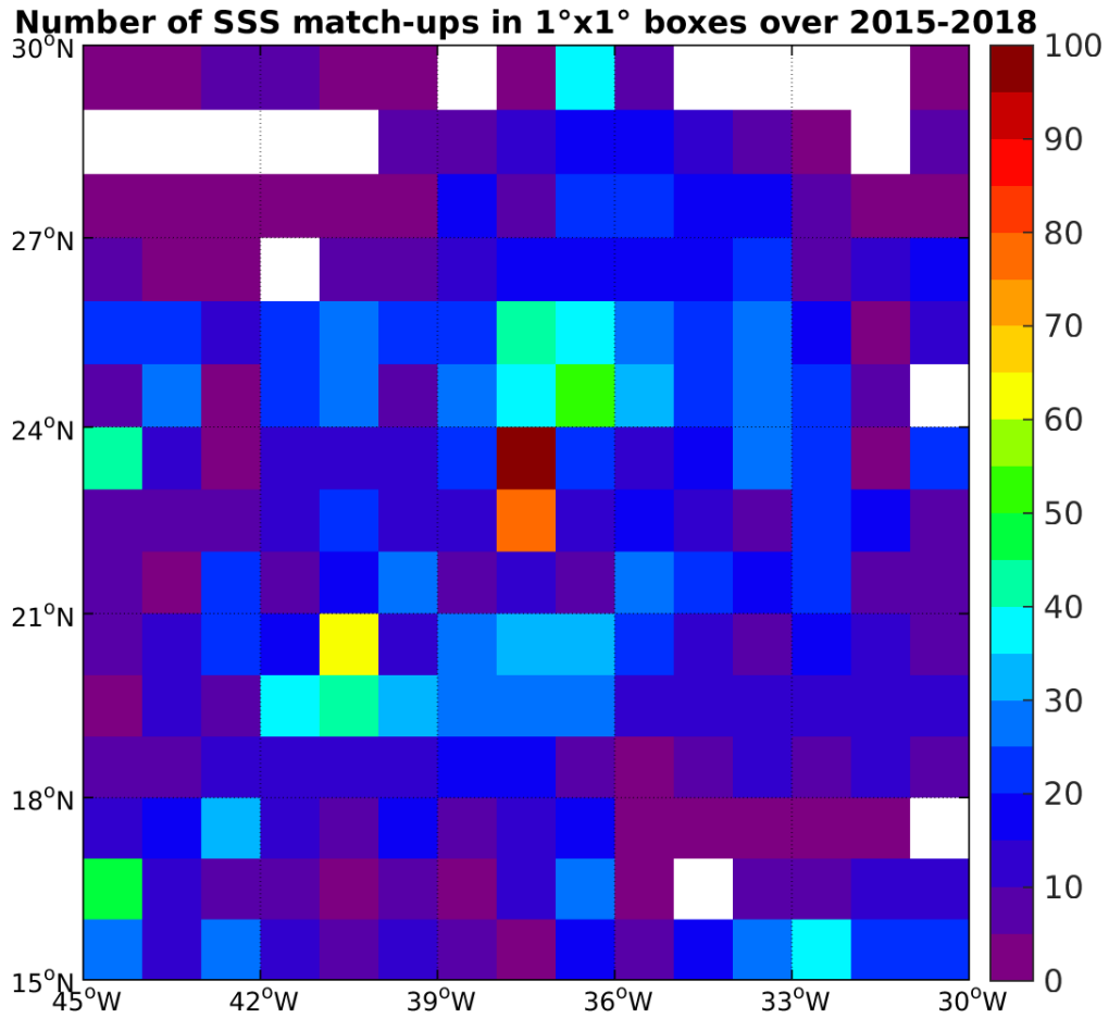
Figure 4: Number of SSS match-ups between Argo SSS and the SMAP-L3-JPL-V4-8DAY-RUNNING-60KM SSS product for the SPURS 1 Pi-MEP region over 1°x1° boxes and for the full satellite product period.
