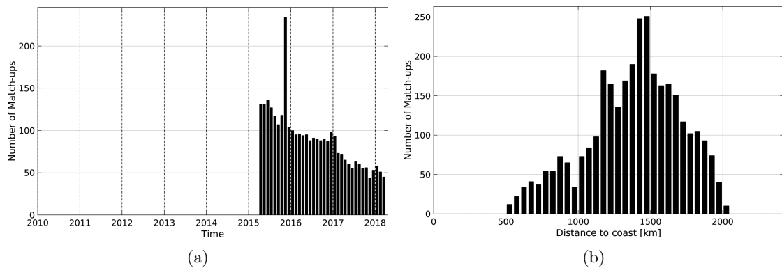
Figure 1: Number of match-ups between Argo and SMAP-L3-JPL-V4-8DAY-RUNNING-60KM SSS as a function of time (a) and as function of the distance to coast (b) over the SPURS 1 Pi-MEP region and for the full satellite product period.
