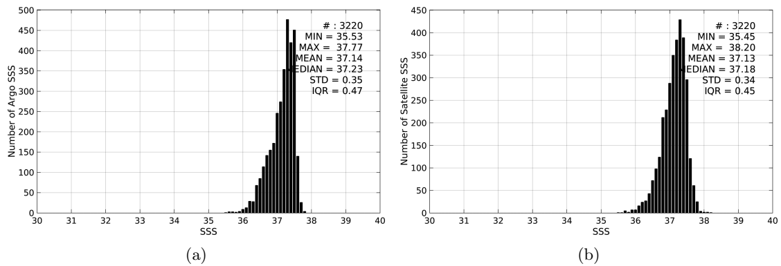
Figure 2: Histograms of SSS from Argo (a) and SMAP-L3-JPL-V4-8DAY-RUNNING-60KM (b) considering all match-up pairs per bins of 0.1 over the SPURS 1 Pi-MEP region and for the full satellite product period.
