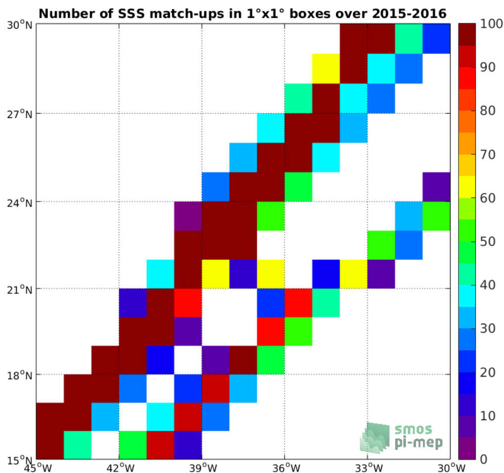
Figure 4: Number of SSS match-ups between TSG-LEGOS-DM SSS and the SMAP-L3-JPL-V4-MONTHLY-60KM SSS product for the SPURS 1 Pi-MEP region over 1°x1° boxes and for the full satellite product period.
