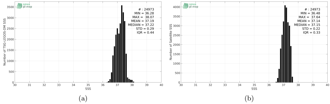
Figure 2: Histograms of SSS from TSG-LEGOS-DM (a) and SMAP-L3-JPL-V4-MONTHLY-60KM (b) considering all match-up pairs per bins of 0.1 over the SPURS 1 Pi-MEP region and for the full satellite product period.
