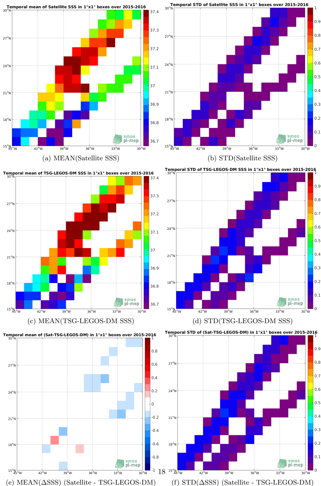
Figure 6: Temporal mean (left) and STD (right) of SSS from SMAP-L3-JPL-V4-MONTHLY-60KM (top), TSG-LEGOS-DM (middle), and of \Delta SSS (Satellite - TSG-LEGOS-DM). Only match-up pairs are used to generate these maps.
