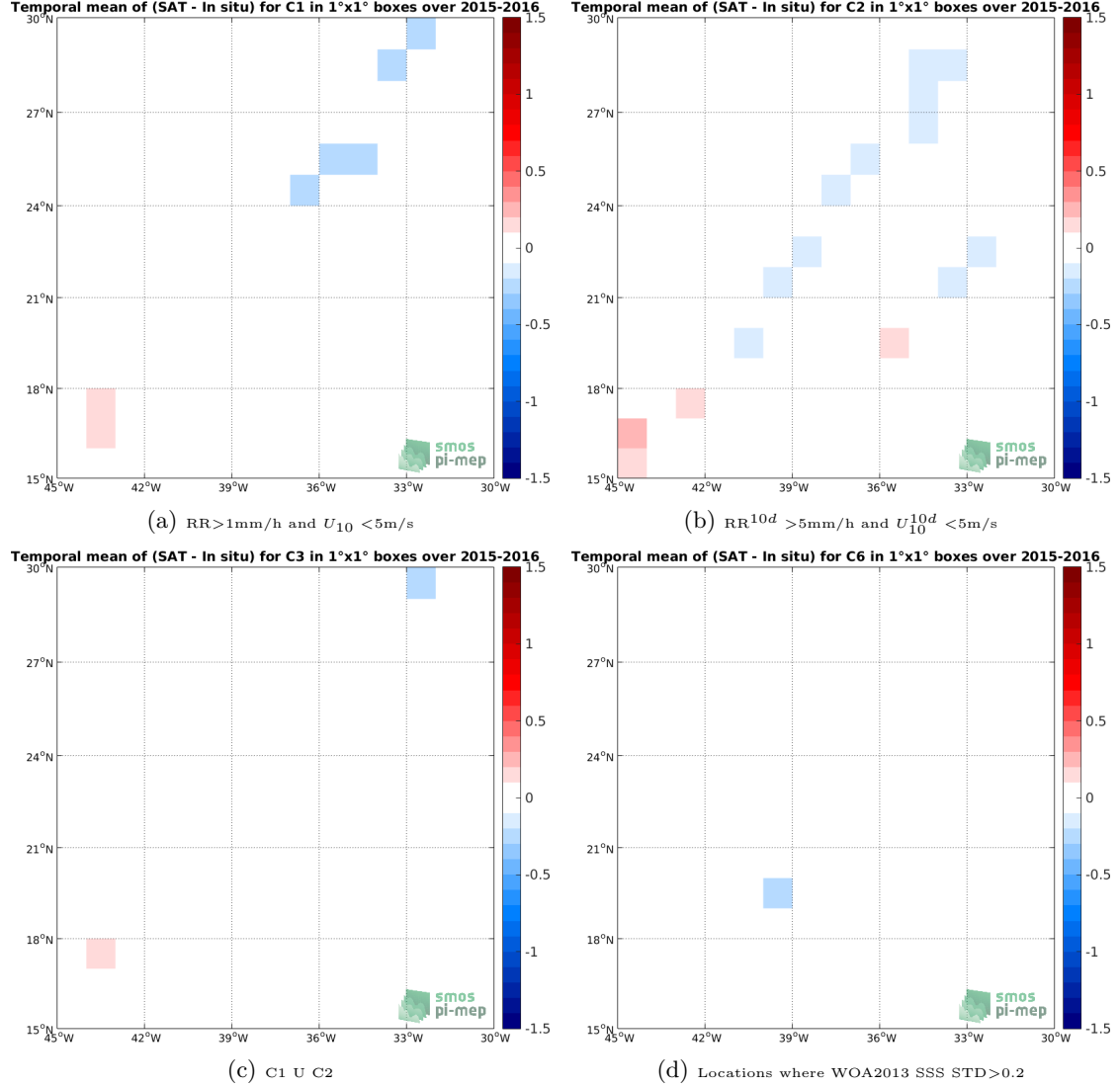
Figure 12: Temporal mean gridded over spatial boxes of size 1^\circ \times 1^\circ of \Delta SSS (SMAP-L3-JPL-V4-MONTHLY-60KM - TSG-LEGOS-DM) for 4 different subdatasets corresponding to: RR > 1\text{mm/h} and U_{10} < 5\text{m/s} (a), RR^{10d} > 5\text{mm/h} and U_{10}^{10d} < 5\text{m/s} (b), C1 U C2 (c), Locations where WOA2013 SSS STD > 0.2 (d).
