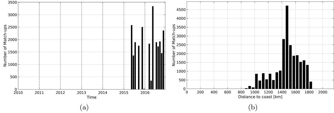
Figure 1: Number of match-ups between TSG-LEGOS-DM and SMAP-L3-JPL-V4-MONTHLY-60KM SSS as a function of time (a) and as function of the distance to coast (b) over the SPURS 1 Pi-MEP region and for the full satellite product period.
