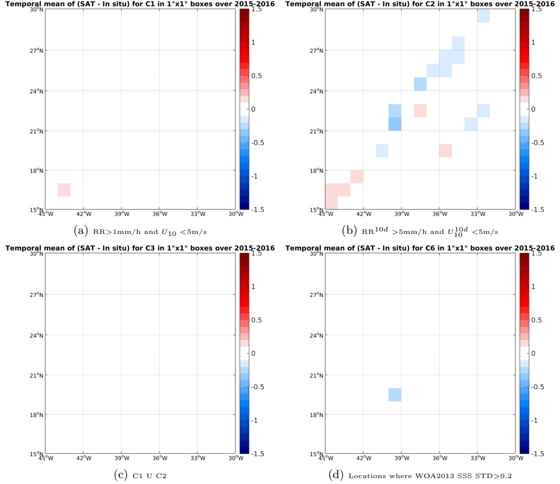
Figure 12: Temporal mean gridded over spatial boxes of size 1^\circ \times 1^\circ of \Delta SSS (SMAP-L3-JPL-V4-MONTHLY-60KM - TSG-LEGOS-DM) for 4 different subdatasets corresponding to: RR > 1 mm/h and U_{10} < 5 m/s (a), RR^{10d} > 5 mm/h and U_{10}^{10d} < 5 m/s (b), C1 U C2 (c), Locations where WOA2013 SSS STD > 0.2 (d).
