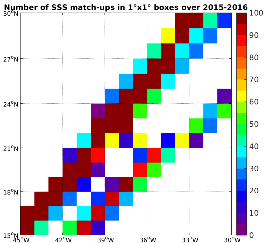
Figure 4: Number of SSS match-ups between TSG-LEGOS-DM SSS and the SMAP-L3-JPL-V4-MONTHLY-60KM SSS product for the SPURS 1 Pi-MEP region over 1°x1° boxes and for the full satellite product period.
