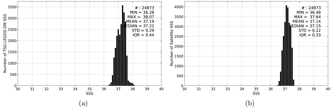
Figure 2: Histograms of SSS from TSG-LEGOS-DM (a) and SMAP-L3-JPL-V4-MONTHLY-60KM (b) considering all match-up pairs per bins of 0.1 over the SPURS 1 Pi-MEP region and for the full satellite product period.
