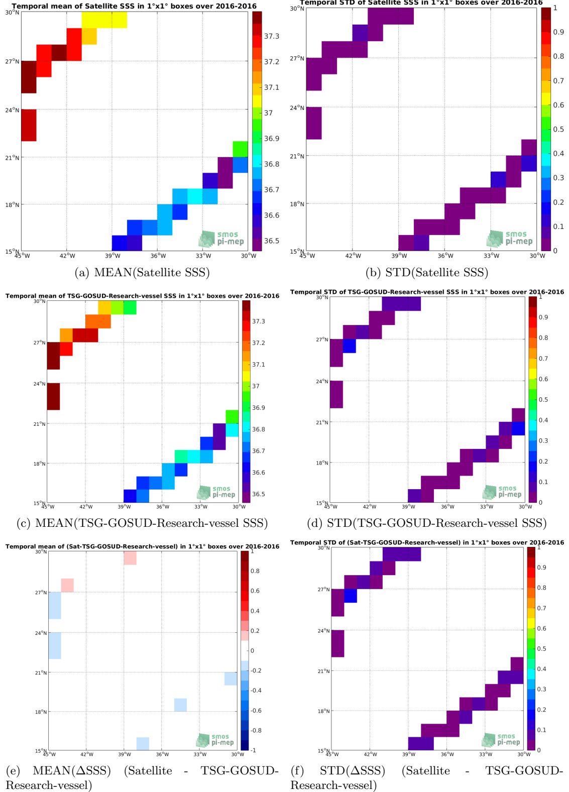
Figure 6: Temporal mean (left) and STD (right) of SSS from SMAP-L3-JPL-V4-MONTHLY-60KM (top), TSG-GOSUD-Research-vessel (middle), and of \Delta SSS (Satellite - TSG-GOSUD-Research-vessel). Only match-up pairs are used to generate these maps.
