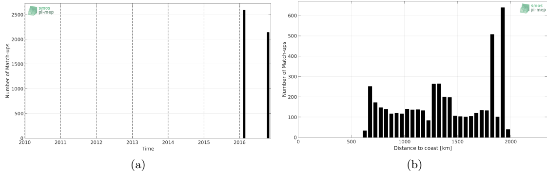
Figure 1: Number of match-ups between TSG-GOSUD-Research-vessel and SMAP-L3-JPL-V4-MONTHLY-60KM SSS as a function of time (a) and as function of the distance to coast (b) over the SPURS 1 Pi-MEP region and for the full satellite product period.
