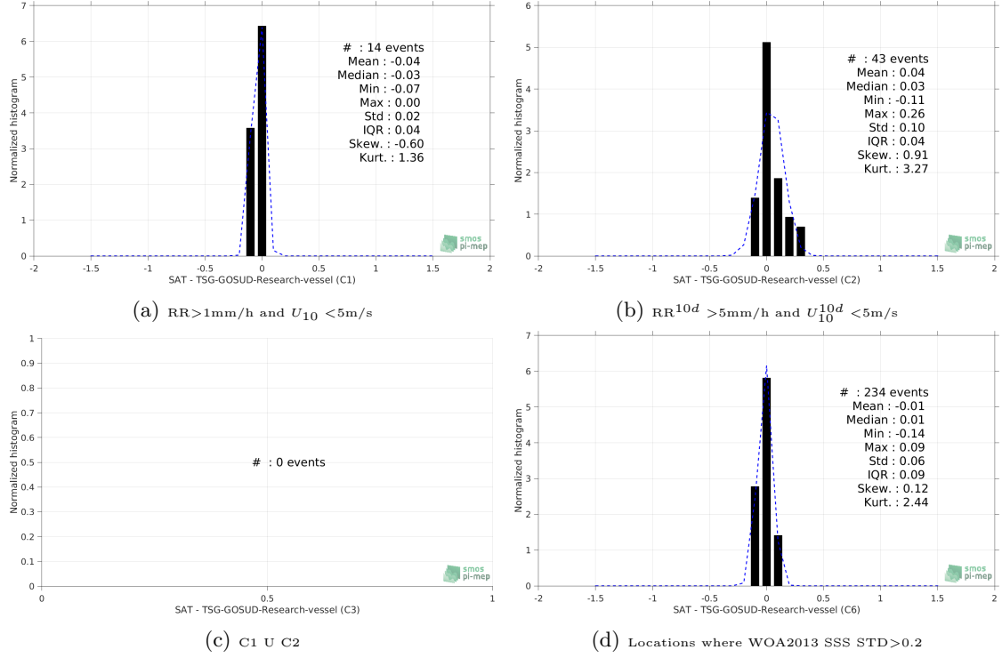
Figure 13: Normalized histogram of \Delta\text{SSS} (SMAP-L3-JPL-V4-MONTHLY-60KM - TSG-GOSUD-Research-vessel) for 6 different subdatasets corresponding to: RR > 1\text{mm/h} and U_{10} < 5\text{m/s} (a), RR^{10d} > 5\text{mm/h} and U_{10}^{10d} < 5\text{m/s} (b), C1 U C2 (c), Locations where WOA2013 SSS STD > 0.2 (d).
