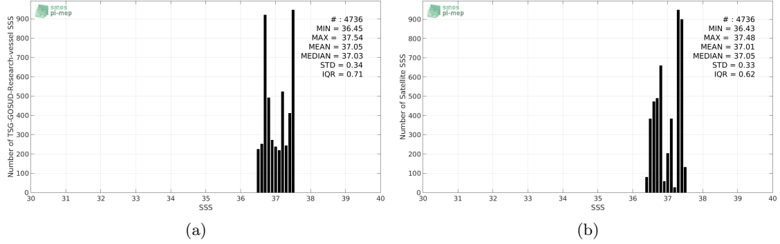
Figure 2: Histograms of SSS from TSG-GOSUD-Research-vessel (a) and SMAP-L3-JPL-V4-MONTHLY-60KM (b) considering all match-up pairs per bins of 0.1 over the SPURS 1 Pi-MEP region and for the full satellite product period.
