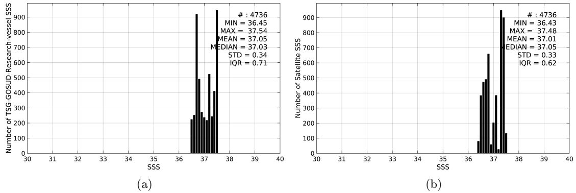
Figure 2: Histograms of SSS from TSG-GOSUD-Research-vessel (a) and SMAP-L3-JPL-V4-MONTHLY-60KM (b) considering all match-up pairs per bins of 0.1 over the SPURS 1 Pi-MEP region and for the full satellite product period.
