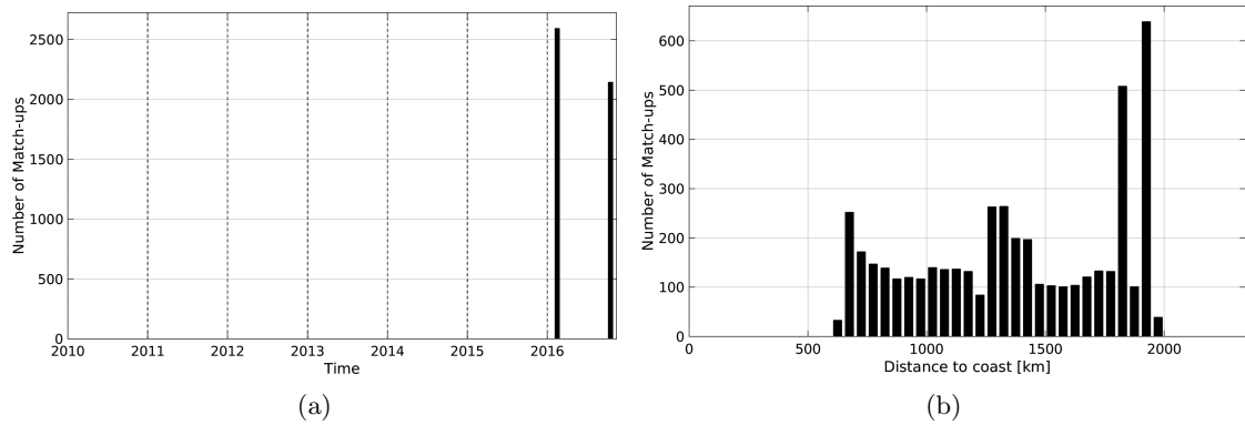
Figure 1: Number of match-ups between TSG-GOSUD-Research-vessel and SMAP-L3-JPL-V4-MONTHLY-60KM SSS as a function of time (a) and as function of the distance to coast (b) over the SPURS 1 Pi-MEP region and for the full satellite product period.
