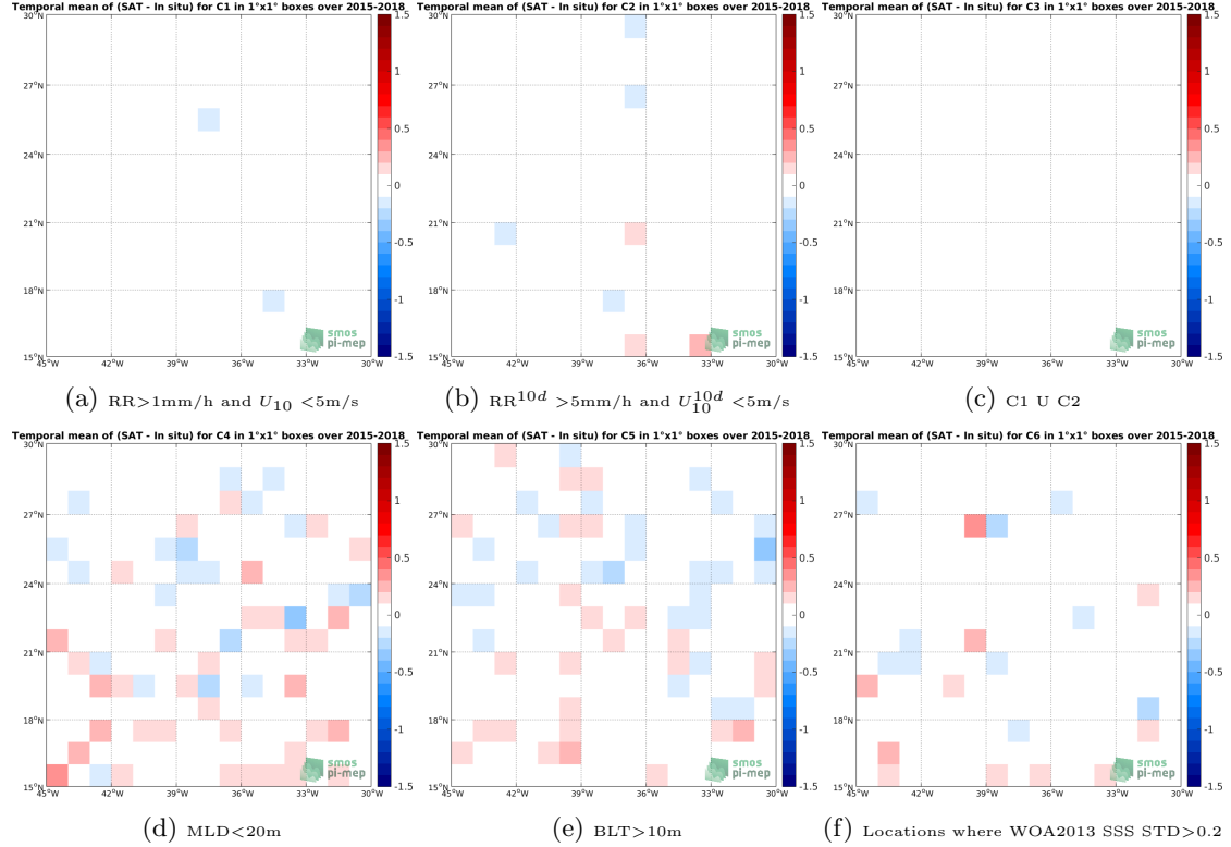
Figure 12: Temporal mean gridded over spatial boxes of size 1^\circ \times 1^\circ of \Delta\text{SSS} (SMAP-L3-JPL-V4-MONTHLY-60KM - Argo) for 6 different subdatasets corresponding to: \text{RR} > 1\text{mm/h} and U_{10} < 5\text{m/s} (a), \text{RR}^{10d} > 5\text{mm/h} and U_{10}^{10d} < 5\text{m/s} (b), C1 U C2 (c), \text{MLD} < 20\text{m} (d), \text{BLT} > 10\text{m} (e), Locations where WOA2013 SSS STD > 0.2 (f).
