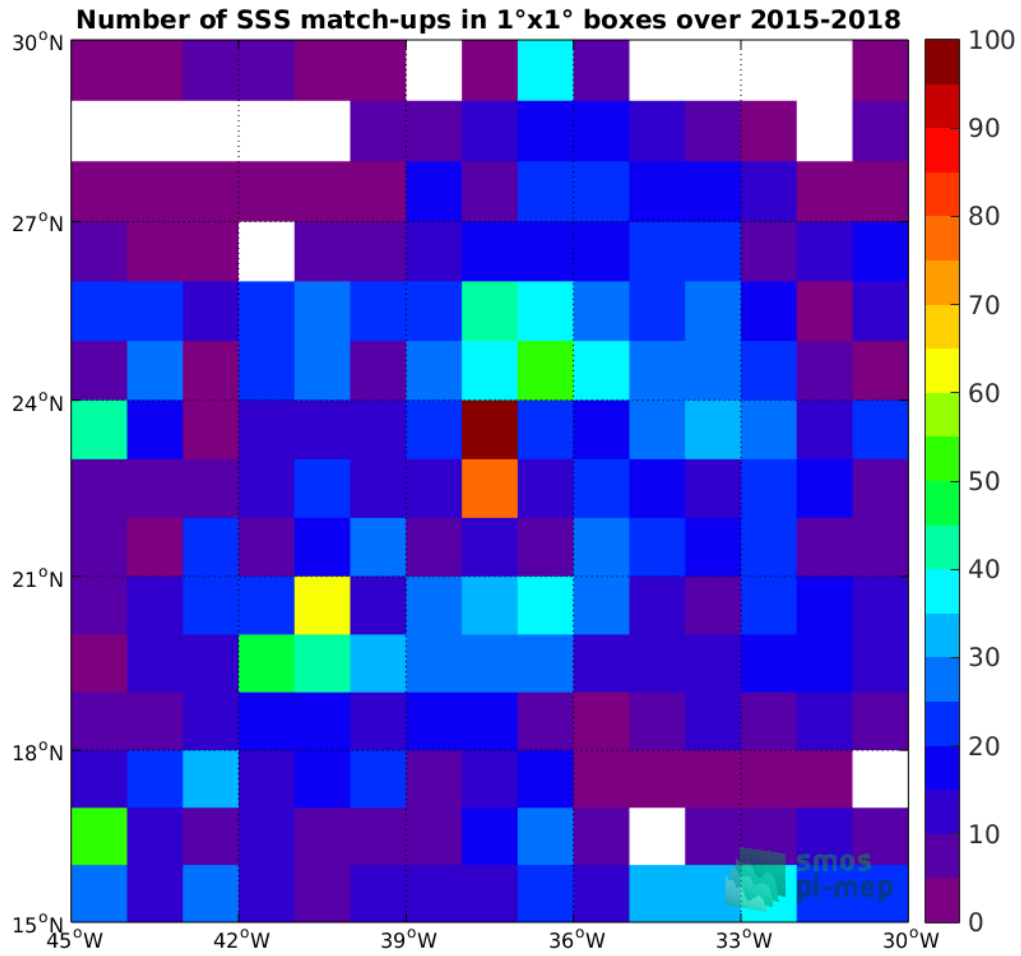
Figure 4: Number of SSS match-ups between Argo SSS and the SMAP-L3-JPL-V4-MONTHLY-60KM SSS product for the SPURS 1 Pi-MEP region over 1°x1° boxes and for the full satellite product period.
