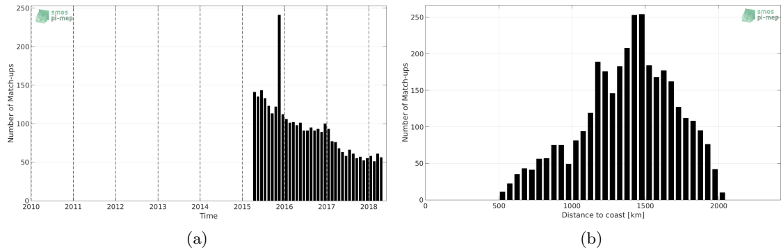
Figure 1: Number of match-ups between Argo and SMAP-L3-JPL-V4-MONTHLY-60KM SSS as a function of time (a) and as function of the distance to coast (b) over the SPURS 1 Pi-MEP region and for the full satellite product period.
