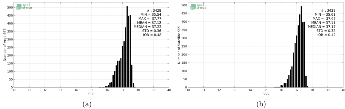
Figure 2: Histograms of SSS from Argo (a) and SMAP-L3-JPL-V4-MONTHLY-60KM (b) considering all match-up pairs per bins of 0.1 over the SPURS 1 Pi-MEP region and for the full satellite product period.
