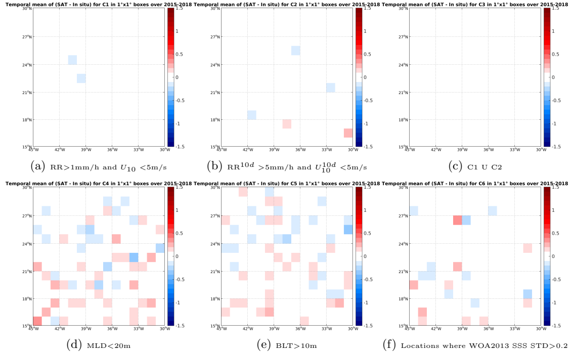
Figure 12: Temporal mean gridded over spatial boxes of size 1^\circ \times 1^\circ of \Delta SSS (SMAP-L3-JPL-V4-MONTHLY-60KM - Argo) for 6 different subdatasets corresponding to: RR > 1mm/h and U_{10} < 5\text{m/s} (a), RR^{10d} > 5\text{mm/h} and U_{10}^{10d} < 5\text{m/s} (b), C1 U C2 (c), MLD < 20m (d), BLT > 10m (e), Locations where WOA2013 SSS STD > 0.2 (f).
