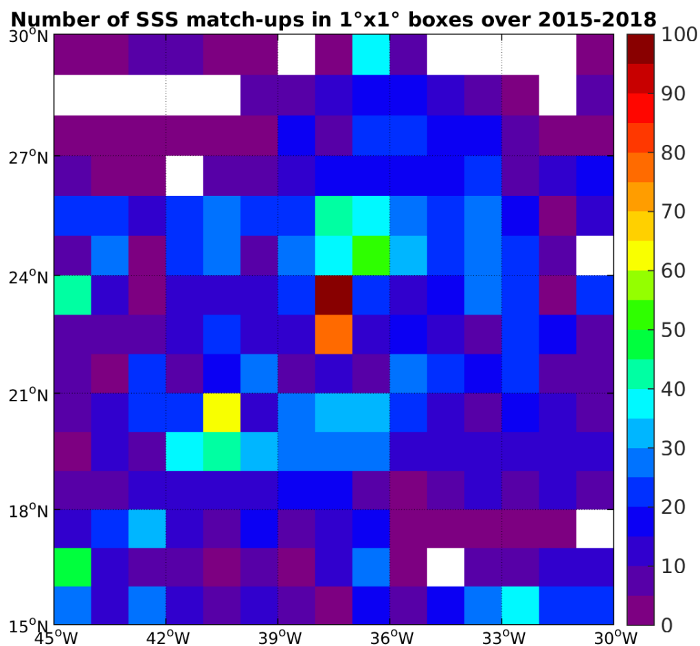
Figure 4: Number of SSS match-ups between Argo SSS and the SMAP-L3-JPL-V4-MONTHLY-60KM SSS product for the SPURS 1 Pi-MEP region over 1°x1° boxes and for the full satellite product period.
