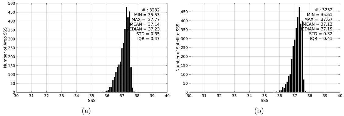
Figure 2: Histograms of SSS from Argo (a) and SMAP-L3-JPL-V4-MONTHLY-60KM (b) considering all match-up pairs per bins of 0.1 over the SPURS 1 Pi-MEP region and for the full satellite product period.
