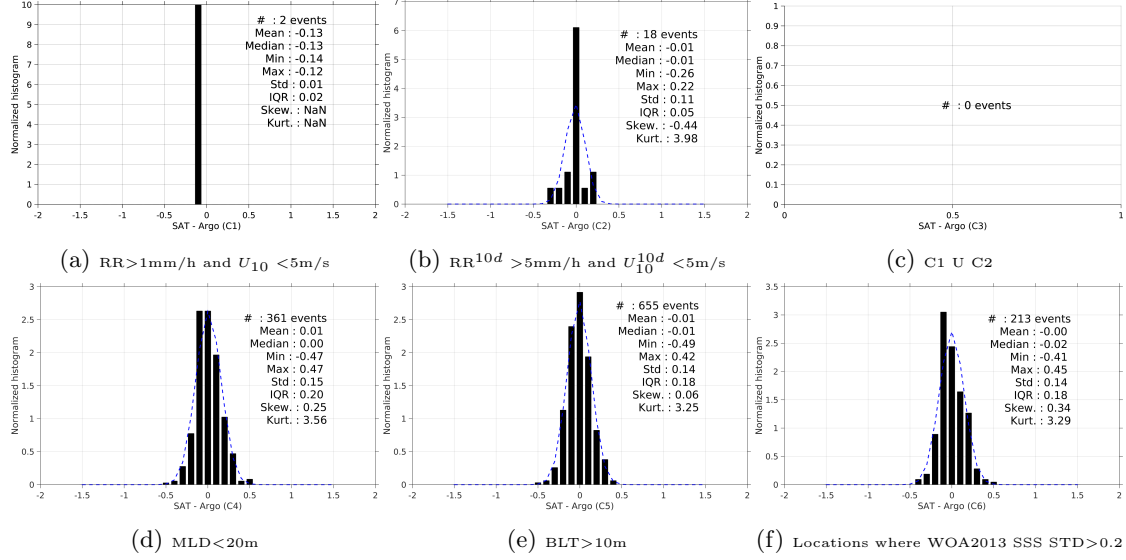
Figure 13: Normalized histogram of \Delta\text{SSS} (SMAP-L3-JPL-V4-MONTHLY-60KM - Argo) for 6 different subdatasets corresponding to: \text{RR}>1\text{mm/h} and U_{10}<5\text{m/s} (a), \text{RR}^{10d}>5\text{mm/h} and U_{10}^{10d}<5\text{m/s} (b), \text{C1 U C2} (c), \text{MLD}<20\text{m} (d), \text{BLT}>10\text{m} (e), Locations where WOA2013 SSS \text{STD}>0.2 (f).
