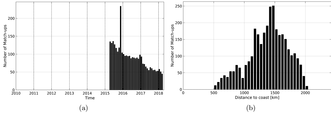
Figure 1: Number of match-ups between Argo and SMAP-L3-JPL-V4-MONTHLY-60KM SSS as a function of time (a) and as function of the distance to coast (b) over the SPURS 1 Pi-MEP region and for the full satellite product period.
