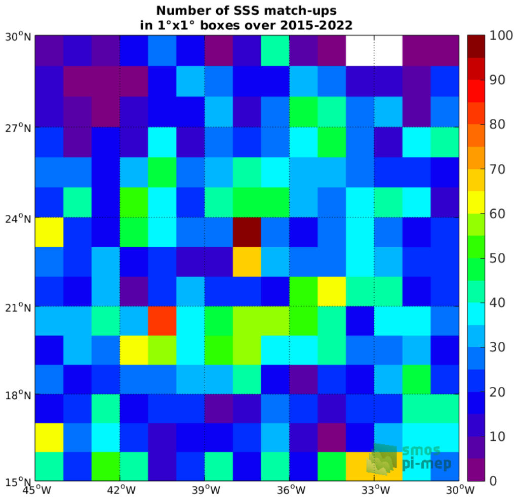
Figure 4: Number of SSS match-ups between Argo SSS and the SMAP SSS L2-AVERAGED v5 (RSS) SSS product for the SPURS 1 Pi-MEP region over 1°x1° boxes and for the full satellite product period.
