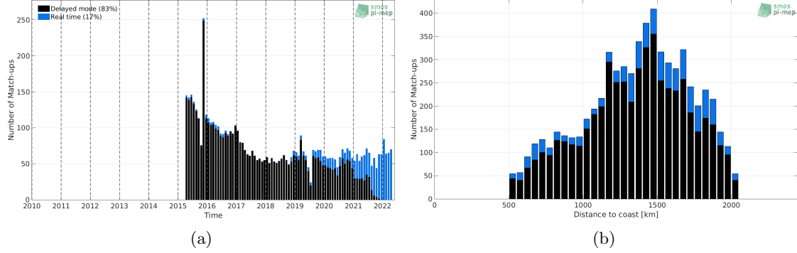
Figure 1: Number of match-ups between Argo and SMAP SSS L2-AVERAGED v5 (RSS) SSS as a function of time (a) and as function of the distance to coast (b) over the SPURS 1 Pi-MEP region and for the full satellite product period.
