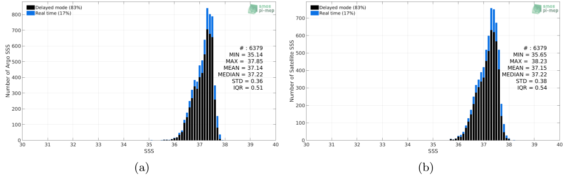
Figure 2: Histograms of SSS from Argo (a) and SMAP SSS L2-AVERAGED v5 (RSS) (b) considering all match-up pairs per bins of 0.1 over the SPURS 1 Pi-MEP region and for the full satellite product period.
