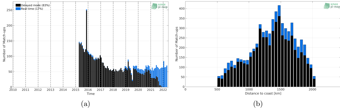
Figure 1: Number of match-ups between Argo and SMAP SSS L2-AVERAGED v5.0 (JPL) SSS as a function of time (a) and as function of the distance to coast (b) over the SPURS 1 Pi-MEP region and for the full satellite product period.
