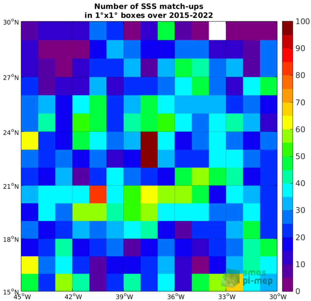
Figure 4: Number of SSS match-ups between Argo SSS and the SMAP SSS L2-AVERAGED v5.0 (JPL) SSS product for the SPURS 1 Pi-MEP region over 1°x1° boxes and for the full satellite product period.
