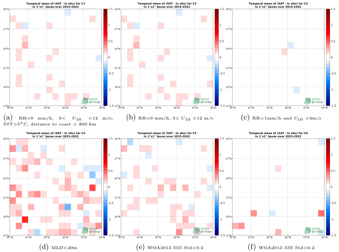
Figure 12: Temporal mean gridded over spatial boxes of size 1^\circ \times 1^\circ of \Delta SSS (SMAP SSS L2-AVERAGED v5.0 (JPL) - Argo) for 6 different subdatasets corresponding to:RR=0 mm/h, 3 < U_{10} < 12 m/s, SST >5^\circ C, distance to coast > 800 km (a), RR=0 mm/h, 3 < U_{10} < 12 m/s (b), RR >1 mm/h and U_{10} < 4 m/s (c),MLD <20 m (d),WOA2013 SSS Std <0.2 (e),WOA2013 SSS Std >0.2 (f).
