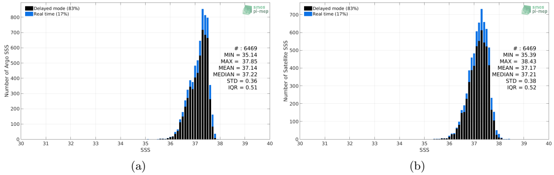
Figure 2: Histograms of SSS from Argo (a) and SMAP SSS L2-AVERAGED v5.0 (JPL) (b) considering all match-up pairs per bins of 0.1 over the SPURS 1 Pi-MEP region and for the full satellite product period.
