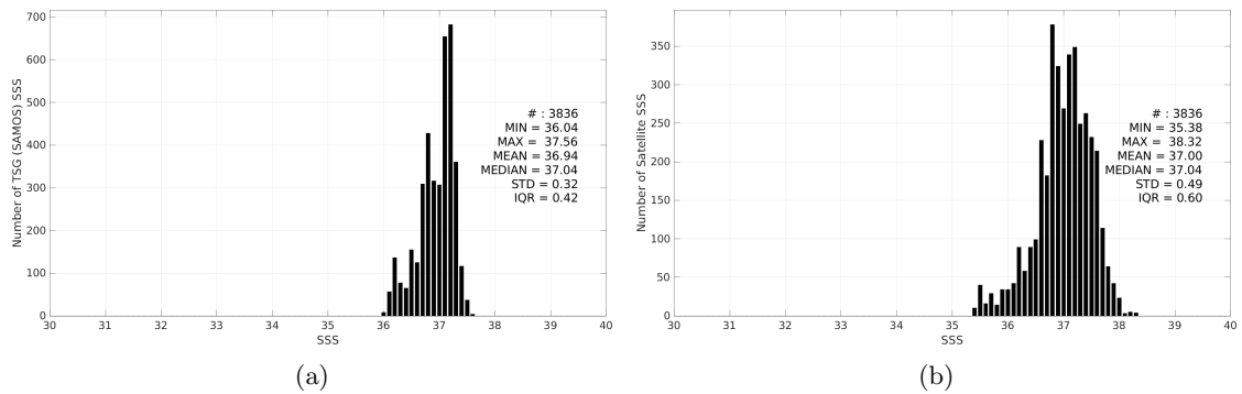
Figure 3: Histograms of SSS from TSG (SAMOS) (a) and SMAP SSS L2 v6 (RSS) (b) considering all match-up pairs per bins of 0.1 over the SPURS 1 Pi-MEP region and for the full satellite product period.
