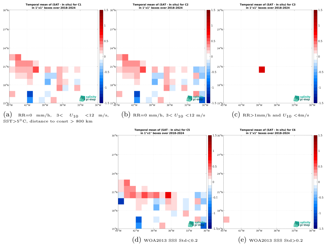
Figure 14: Temporal mean gridded over spatial boxes of size 1^\circ \times 1^\circ of \Delta SSS (SMAP SSS L2 v6 (RSS) - TSG (SAMOS)) for 5 different subdatasets corresponding to:RR=0 mm/h, 3 < U_{10} < 12 m/s, SST>5°C, distance to coast > 800 km (a), RR=0 mm/h, 3 < U_{10} < 12 m/s (b), RR>1mm/h and U_{10} < 4 m/s (c), WOA2013 SSS Std<0.2 (d), WOA2013 SSS Std>0.2 (e).
