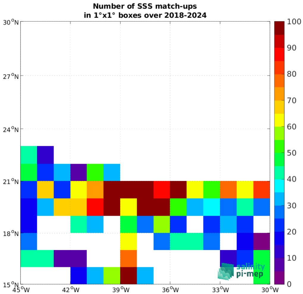
Figure 5: Number of SSS match-ups between TSG (SAMOS) SSS and the SMAP SSS L2 v6 (RSS) SSS product for the SPURS 1 Pi-MEP region over 1°x1° boxes and for the full satellite product period.
