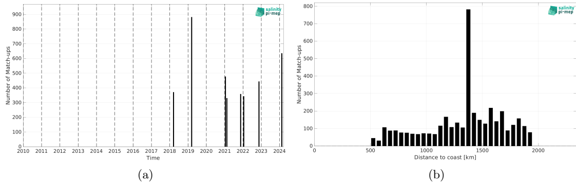
Figure 2: Number of match-ups between TSG (SAMOS) and SMAP SSS L2 v6 (RSS) SSS as a function of time (a) and as function of the distance to coast (b) over the SPURS 1 Pi-MEP region and for the full satellite product period.
