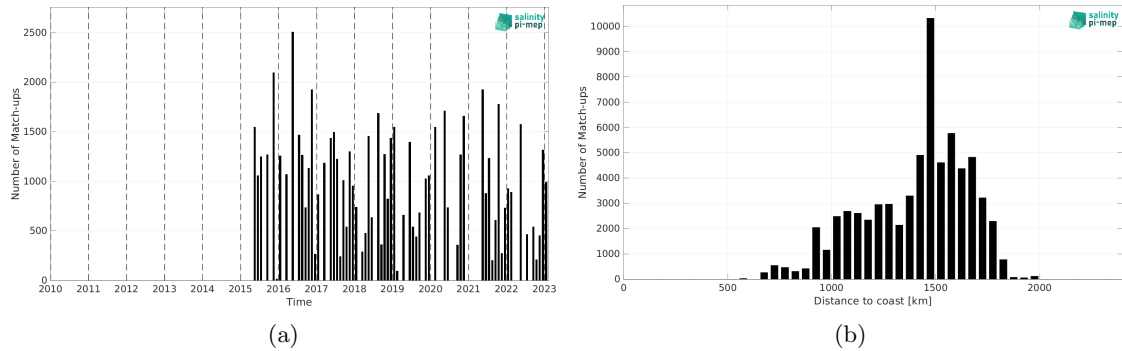
Figure 2: Number of match-ups between TSG (LEGOS-DM) and SMAP SSS L2 v6 (RSS) SSS as a function of time (a) and as function of the distance to coast (b) over the SPURS 1 Pi-MEP region and for the full satellite product period.
