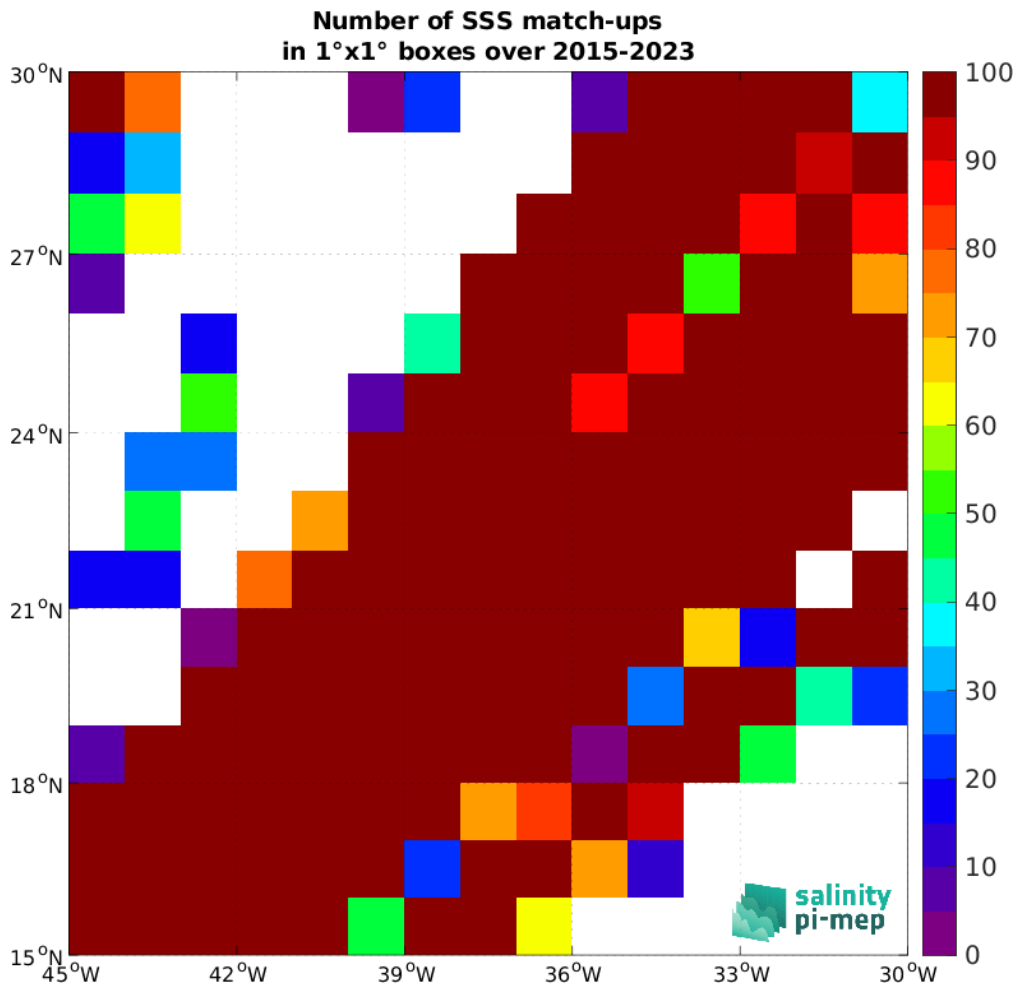
Figure 5: Number of SSS match-ups between TSG (LEGOS-DM) SSS and the SMAP SSS L2 v6 (RSS) SSS product for the SPURS 1 Pi-MEP region over 1°x1° boxes and for the full satellite product period.
