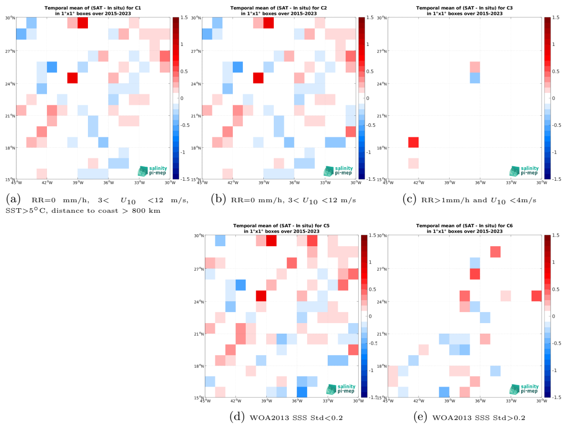
Figure 14: Temporal mean gridded over spatial boxes of size 1^\circ \times 1^\circ of \Delta\text{SSS} (SMAP SSS L2 v6 (RSS) - TSG (LEGOS-DM)) for 5 different subdatasets corresponding to:RR=0 mm/h, 3 < U_{10} < 12 m/s, SST>5°C, distance to coast > 800 km (a), RR=0 mm/h, 3 < U_{10} < 12 m/s (b), RR>1mm/h and U_{10} < 4 m/s (c), WOA2013 SSS Std<0.2 (d), WOA2013 SSS Std>0.2 (e).
