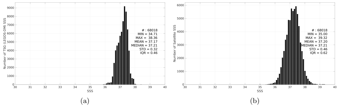
Figure 3: Histograms of SSS from TSG (LEGOS-DM) (a) and SMAP SSS L2 v6 (RSS) (b) considering all match-up pairs per bins of 0.1 over the SPURS 1 Pi-MEP region and for the full satellite product period.
