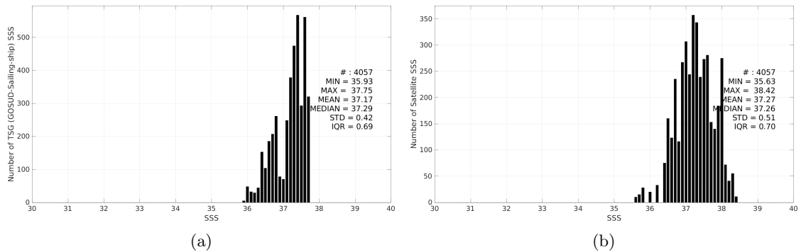
Figure 3: Histograms of SSS from TSG (GOSUD-Sailing-ship) (a) and SMAP SSS L2 v6 (RSS) (b) considering all match-up pairs per bins of 0.1 over the SPURS 1 Pi-MEP region and for the full satellite product period.
