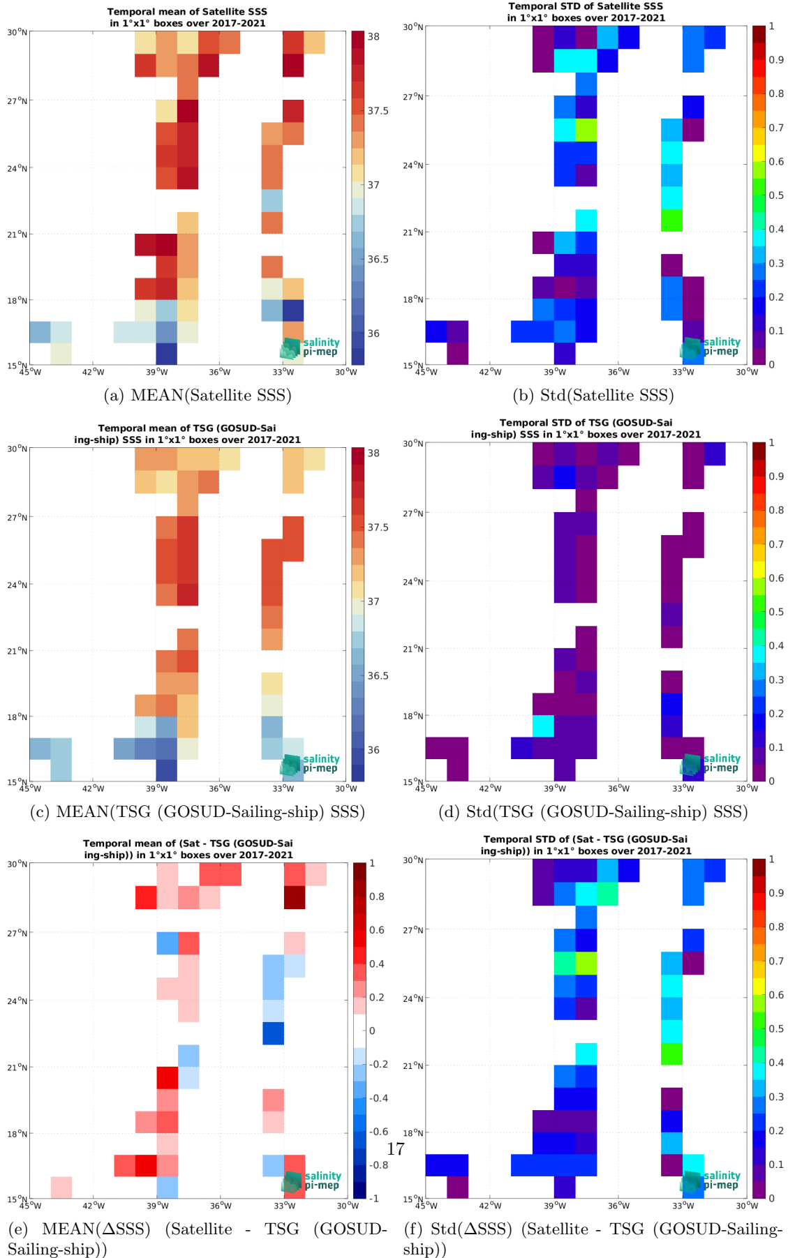
Figure 7: Temporal mean (left) and Std (right) of SSS from SMAP SSS L2 v6 (RSS) (top), TSG (GOSUD-Sailing-ship) (middle), and of \Delta SSS (Satellite - TSG (GOSUD-Sailing-ship)). Only match-up pairs are used to generate these maps.
