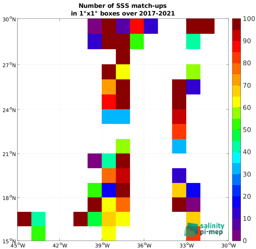
Figure 5: Number of SSS match-ups between TSG (GOSUD-Sailing-ship) SSS and the SMAP SSS L2 v6 (RSS) SSS product for the SPURS 1 Pi-MEP region over 1°x1° boxes and for the full satellite product period.
