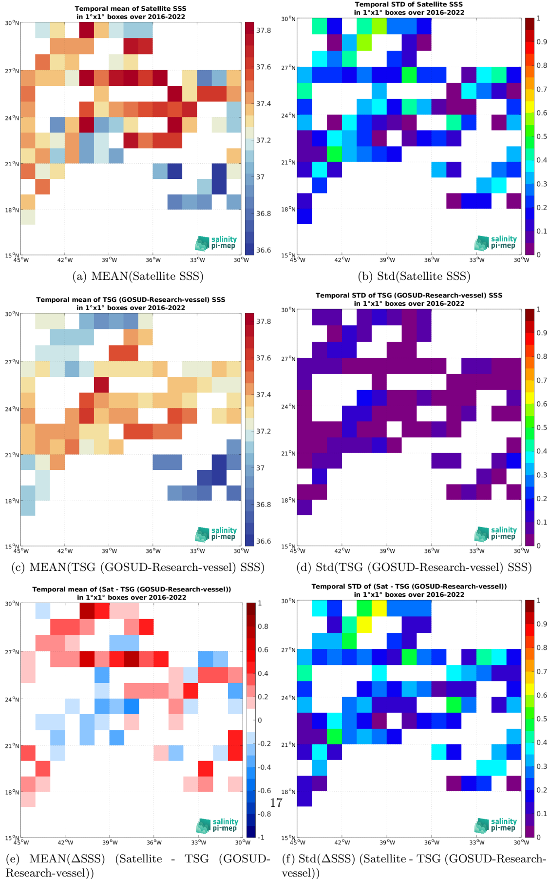
Figure 7: Temporal mean (left) and Std (right) of SSS from SMAP SSS L2 v6 (RSS) (top), TSG (GOSUD-Research-vessel) (middle), and of \Delta SSS (Satellite - TSG (GOSUD-Research-vessel)). Only match-up pairs are used to generate these maps.
