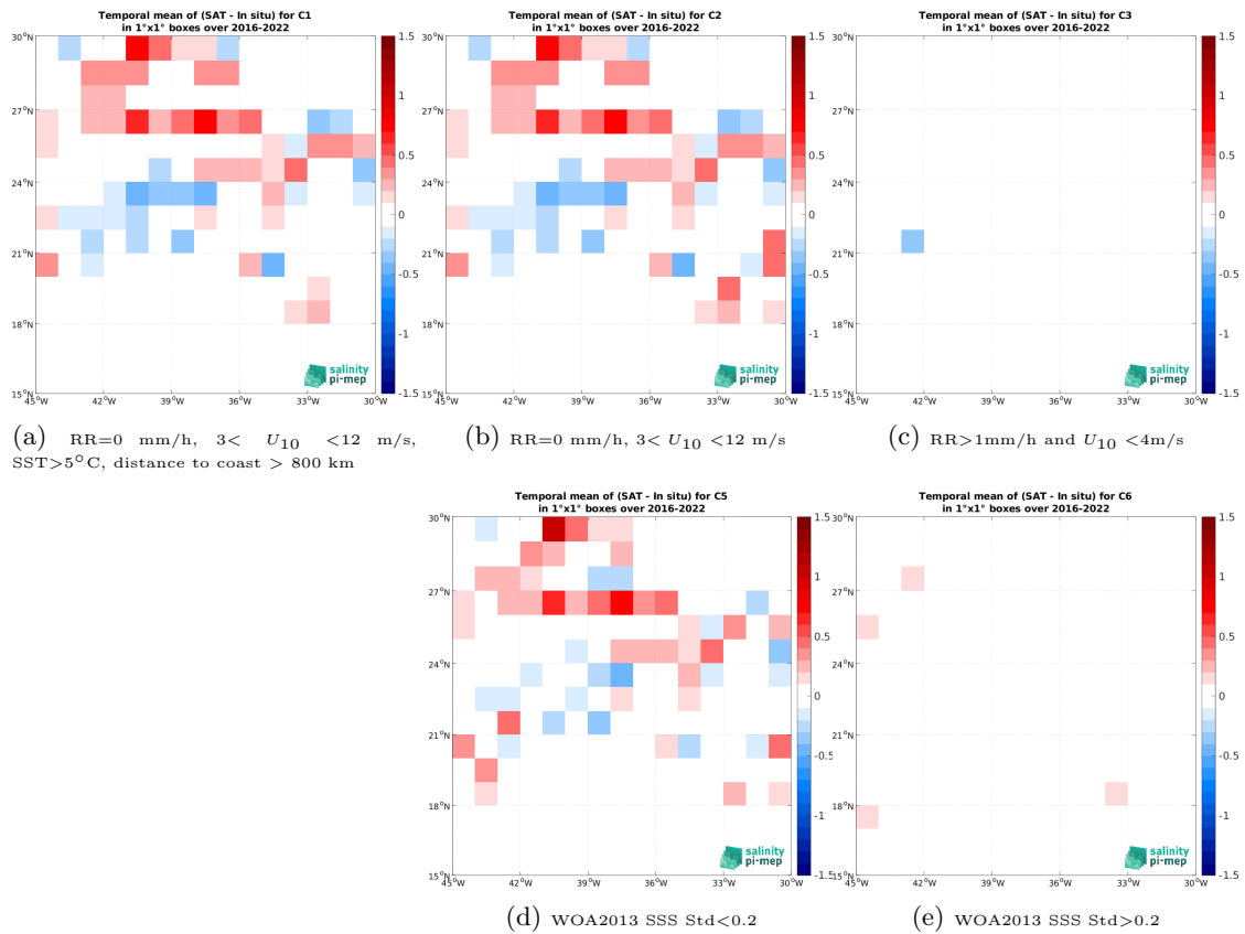
Figure 14: Temporal mean gridded over spatial boxes of size 1^\circ \times 1^\circ of \Delta SSS (SMAP SSS L2 v6 (RSS) - TSG (GOSUD-Research-vessel)) for 5 different subdatasets corresponding to:RR=0 mm/h, 3 < U_{10} < 12 m/s, SST >5^\circ C, distance to coast > 800 km (a), RR=0 mm/h, 3 < U_{10} < 12 m/s (b), RR >1 mm/h and U_{10} < 4 m/s (c), WOA2013 SSS Std <0.2 (d), WOA2013 SSS Std >0.2 (e).
