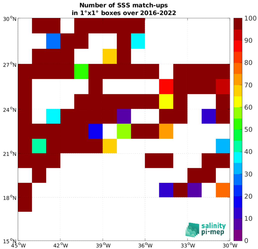
Figure 5: Number of SSS match-ups between TSG (GOSUD-Research-vessel) SSS and the SMAP SSS L2 v6 (RSS) SSS product for the SPURS 1 Pi-MEP region over 1°x1° boxes and for the full satellite product period.
