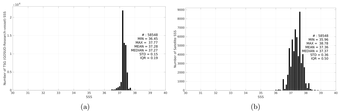
Figure 3: Histograms of SSS from TSG (GOSUD-Research-vessel) (a) and SMAP SSS L2 v6 (RSS) (b) considering all match-up pairs per bins of 0.1 over the SPURS 1 Pi-MEP region and for the full satellite product period.
