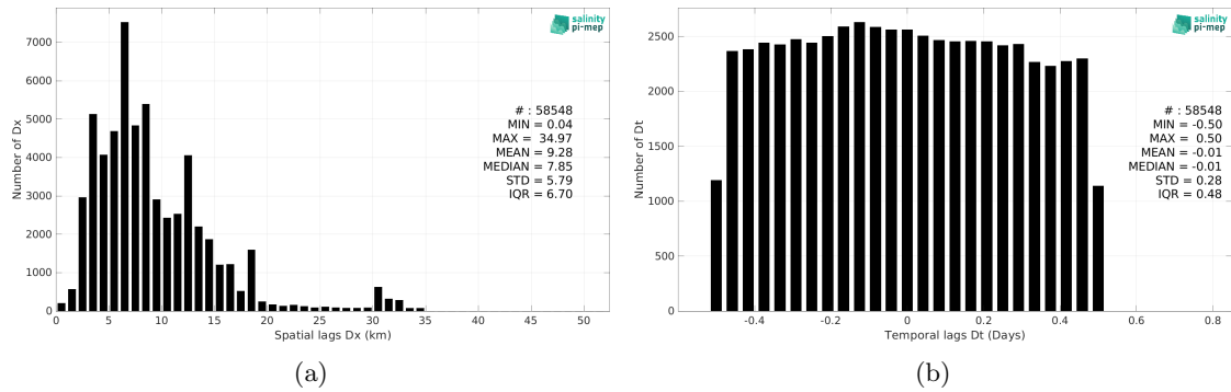
Figure 6: Histograms of the spatial (a) and temporal (b) lags between the location/time of the TSG (GOSUD-Research-vessel) measurement and the date of the corresponding SMAP SSS L2 v6 (RSS) SSS pixel.
