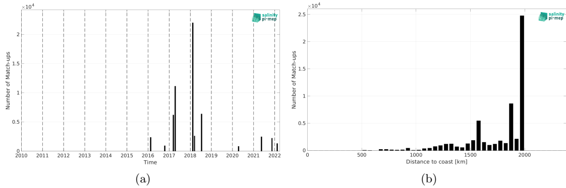
Figure 2: Number of match-ups between TSG (GOSUD-Research-vessel) and SMAP SSS L2 v6 (RSS) SSS as a function of time (a) and as function of the distance to coast (b) over the SPURS 1 Pi-MEP region and for the full satellite product period.
